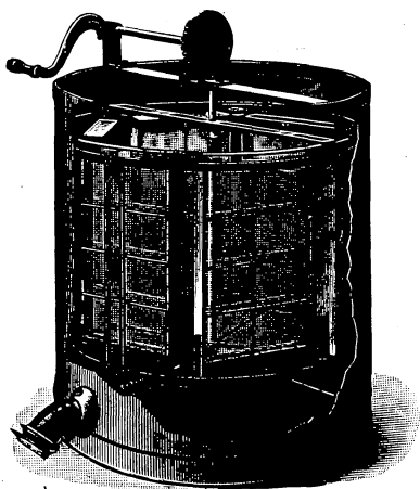
FIG. 10.—The Williams automatic reversible honey extractor.
