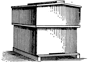
FIG. 17.—Double-walled hive adapted to outdoor wintering as well as summer use below 40° north latitude in the United States. Thickness of each wall, \frac{3}{8} inch; space between walls, 2 inches, packed with dry chaff or ground cork.
