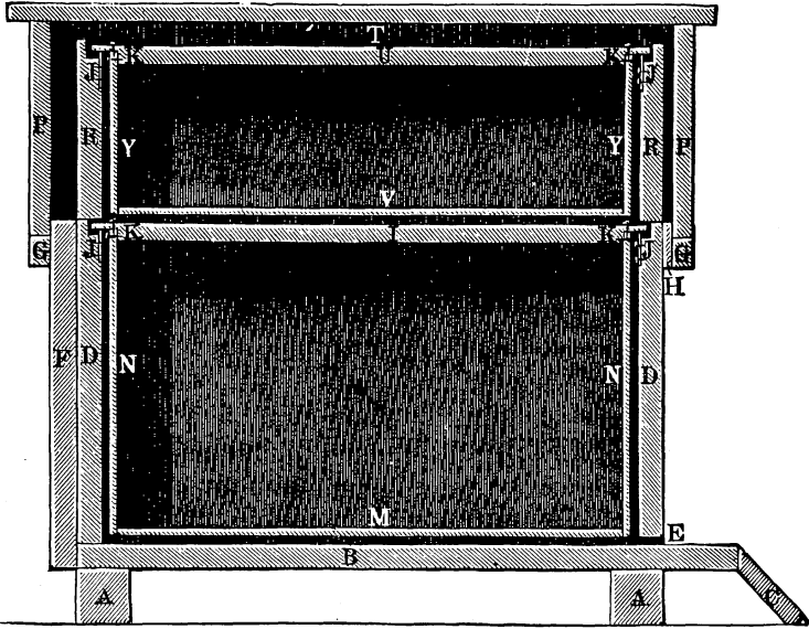
FIG. 5.—The Langstroth hive—Dadant-Quinby form—cross section showing construction.
