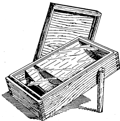
FIG. 15.—Solar wax-extractor.
