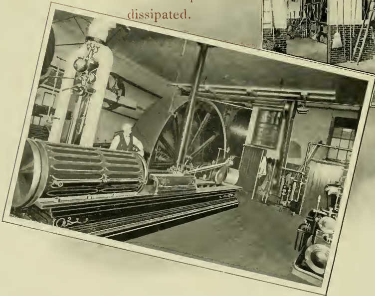
ENGINE AND BOILER ROOM, MILL NO. 1.
