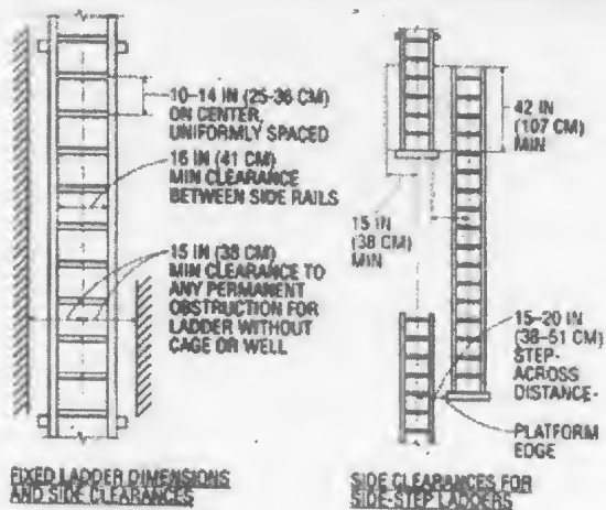
Figure D-2 -- Side-Step Fixed Ladder Sections
