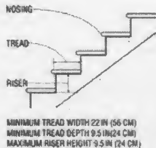
Figure D-8 -- Dimensions of Standard Stairs
