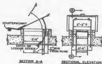
Figure D-2 -- Side-Step Fixed Ladder Sections
