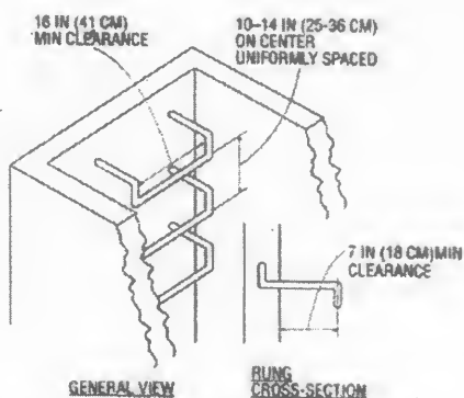
Figure D-4 -- Individual Rung Ladder
