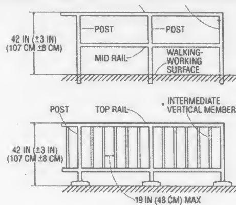
Figure D-10 – Guard Rail Systems
