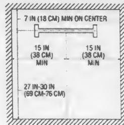
Figure 13 -- Clearances for Fixed Ladders in Wells
