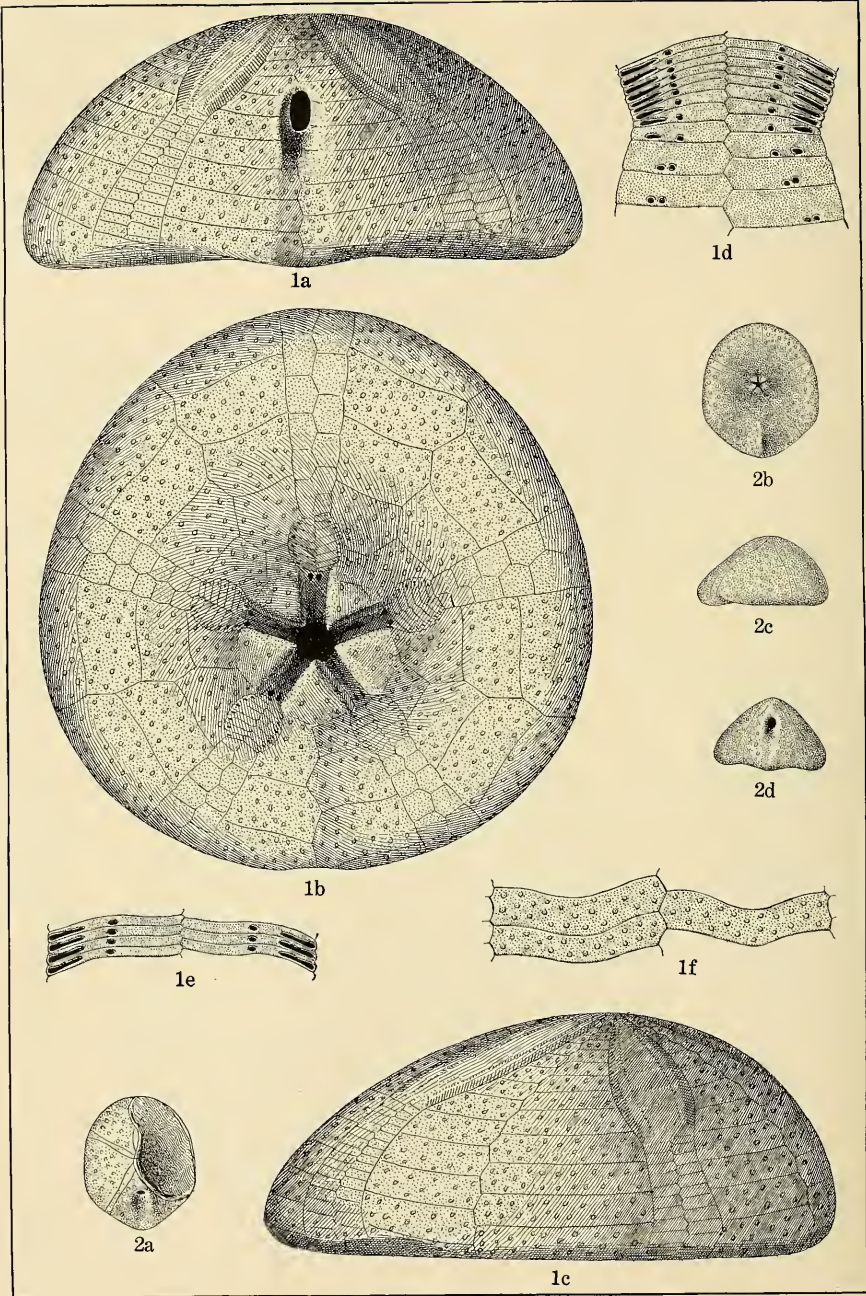
CRETACEOUS ECHINOIDEA.
