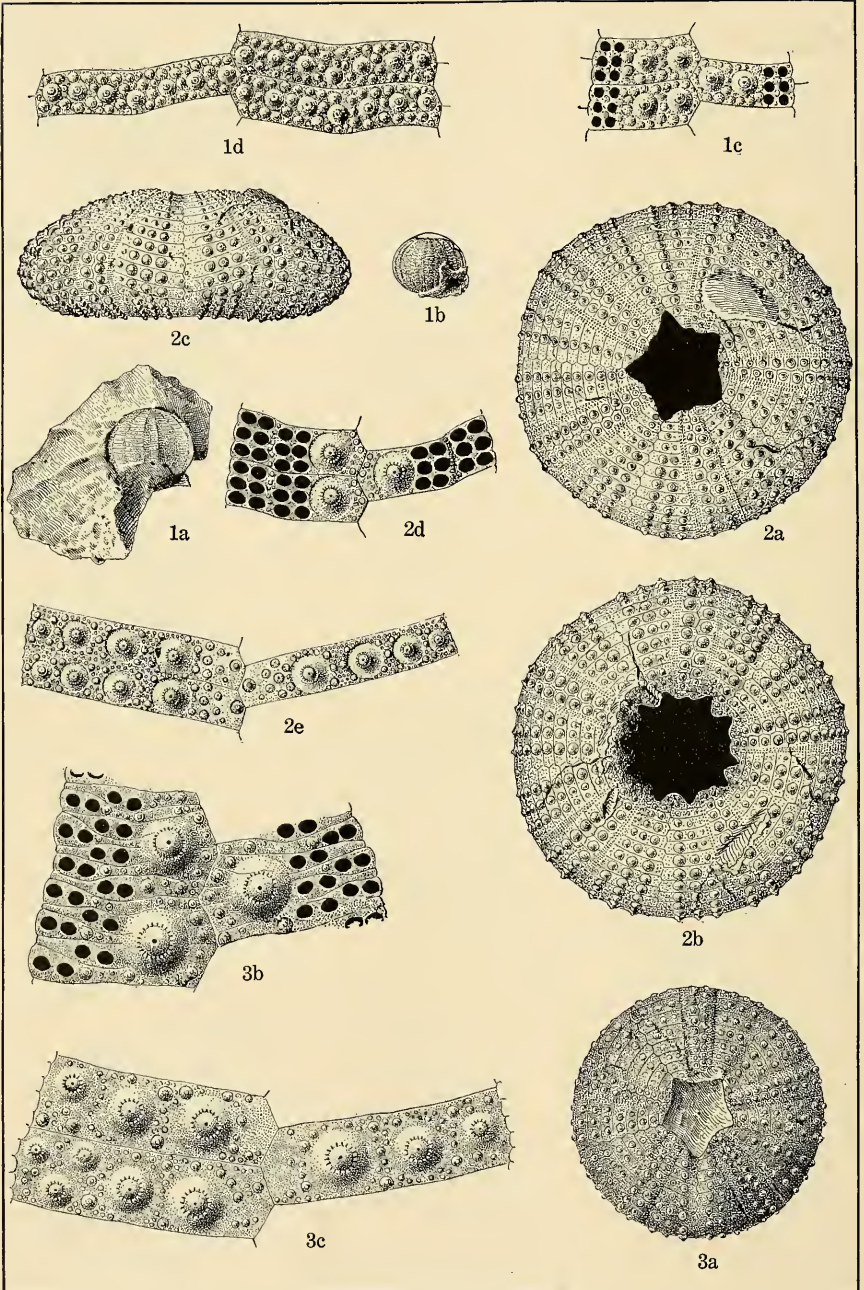
CRETACEOUS ECHINOIDEA.
