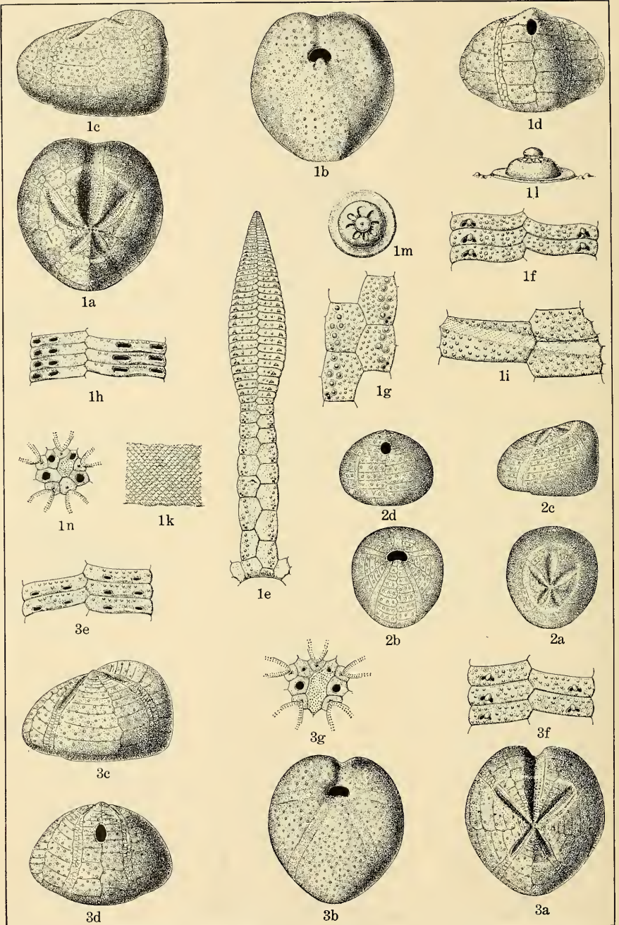
CRETACEOUS ECHINOIDEA.
