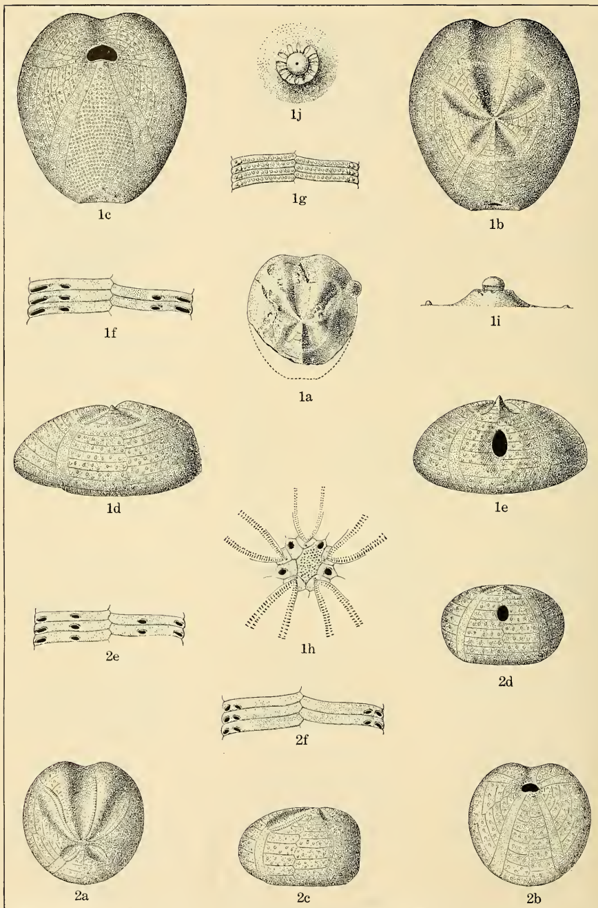
CRETACEOUS ECHINOIDEA.
