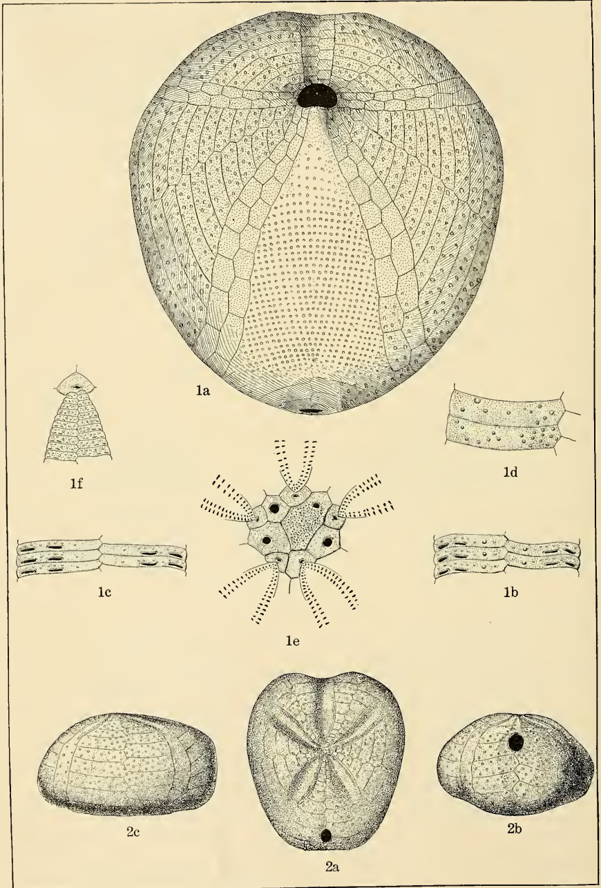
CRETACEOUS ECHINOIDEA.
