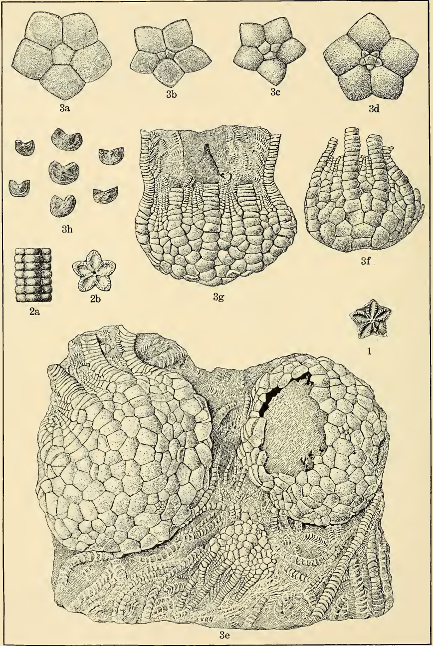
CRETACEOUS CRINOIDEA.
