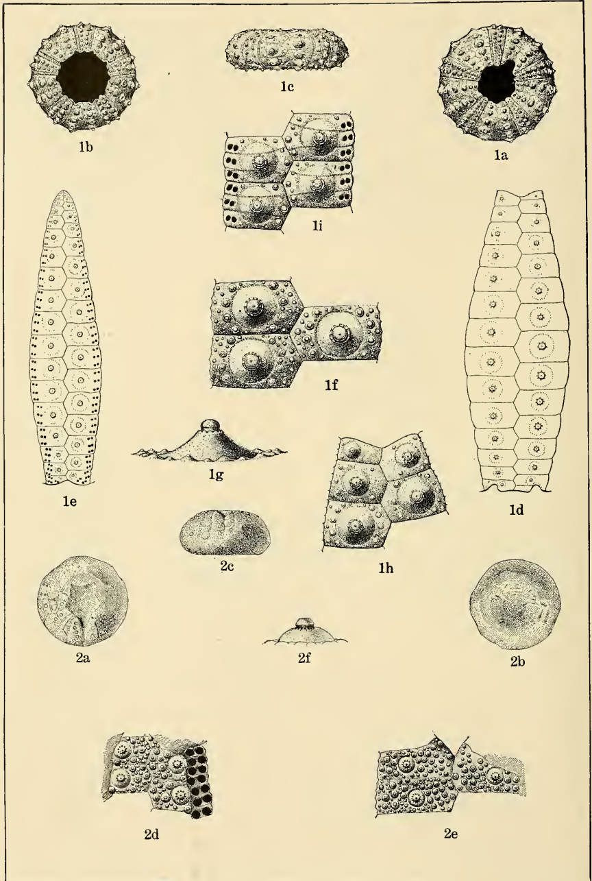
CRETACEOUS ECHINOIDEA.
