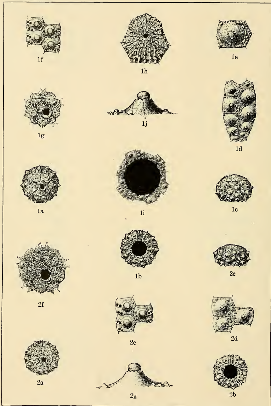
CRETACEOUS ECHINOIDEA.
