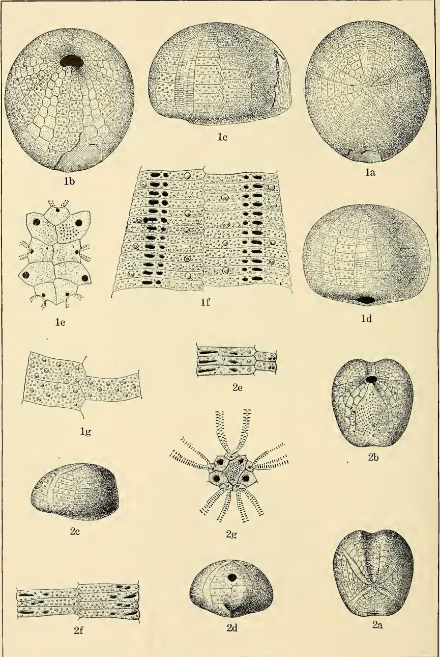
CRETACEOUS ECHINOIDEA.
