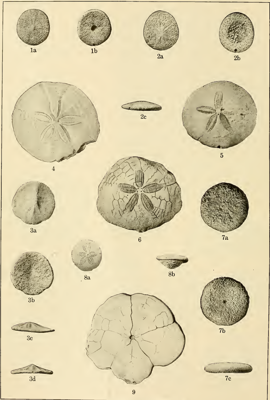
MIOCENE ECHINOIDEA.
