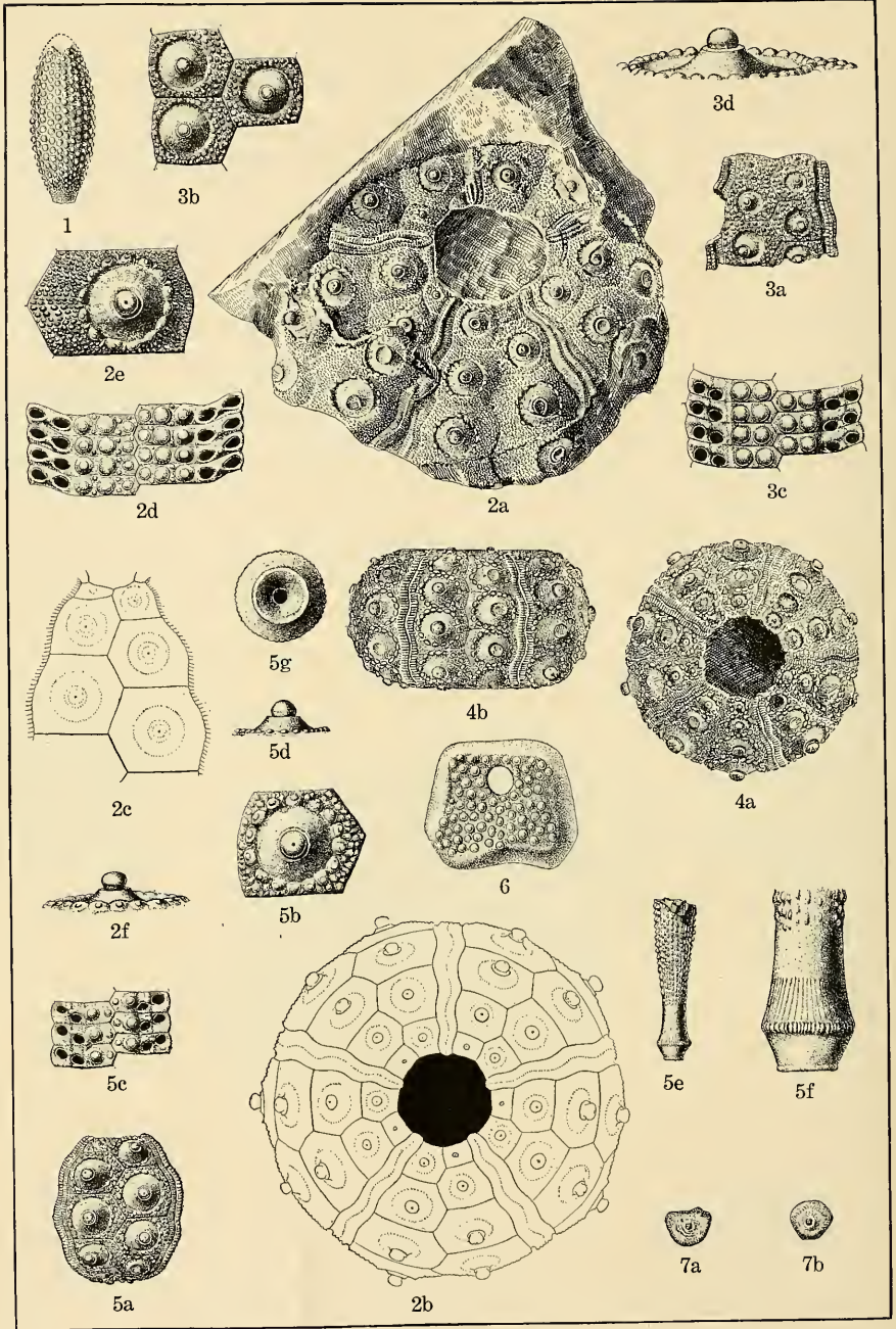
CRETACEOUS ECHINOIDEA.
