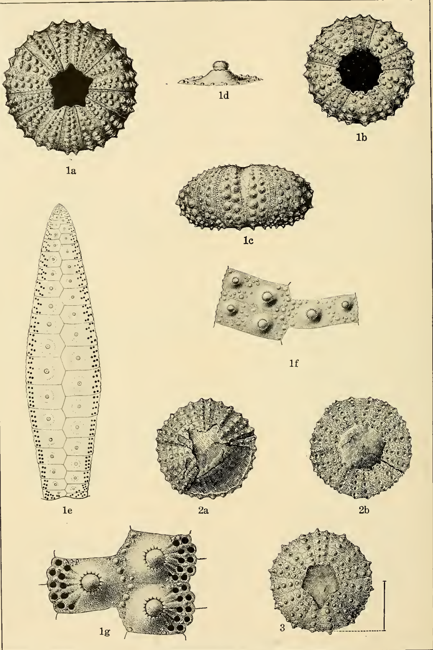
CRETACEOUS ECHINOIDEA.
