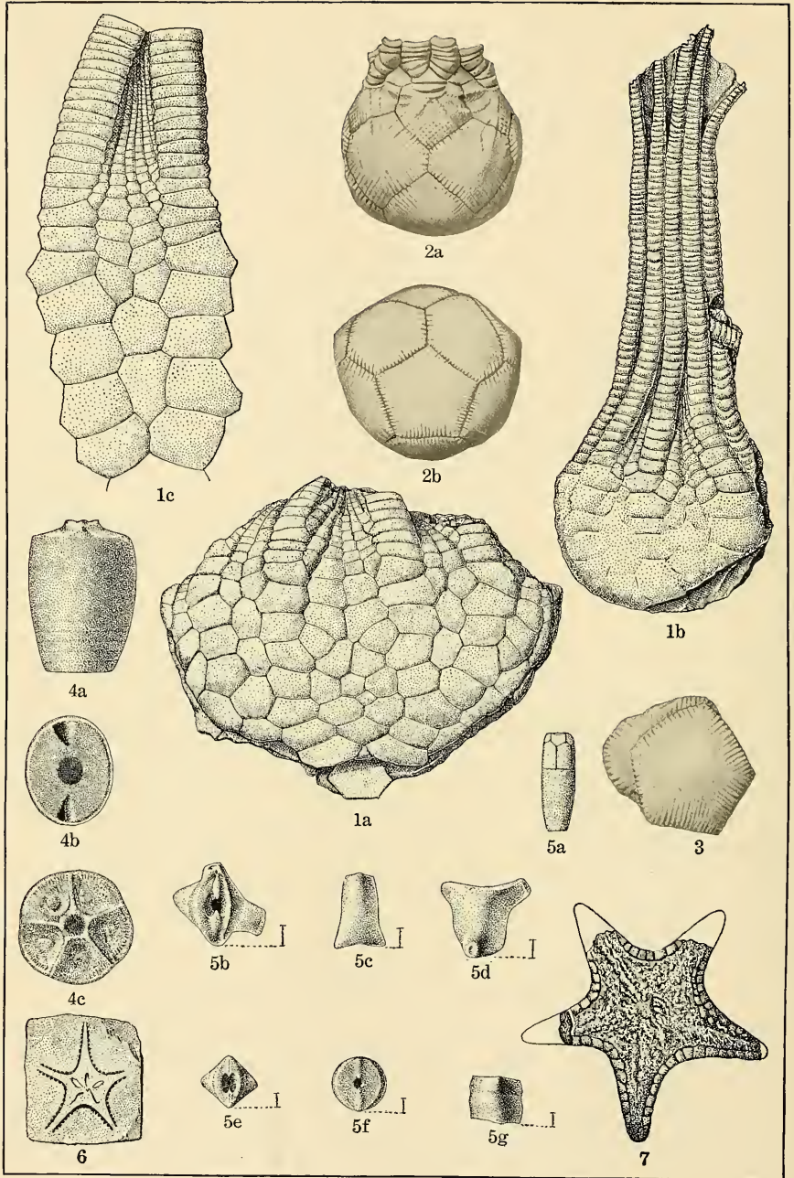
CRETACEOUS CRINOIDEA AND STELLEROIDEA.
