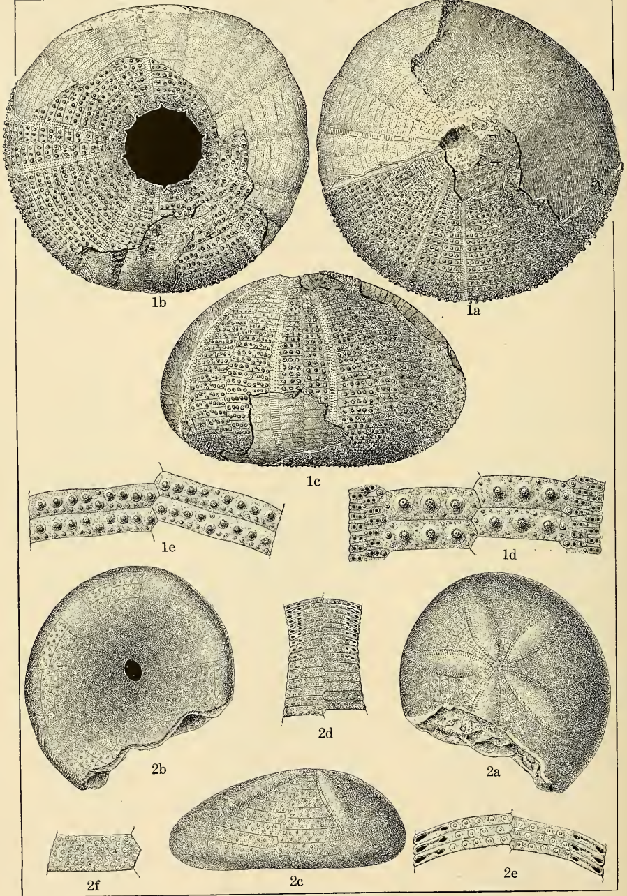
CRETACEOUS ECHINOIDEA.
