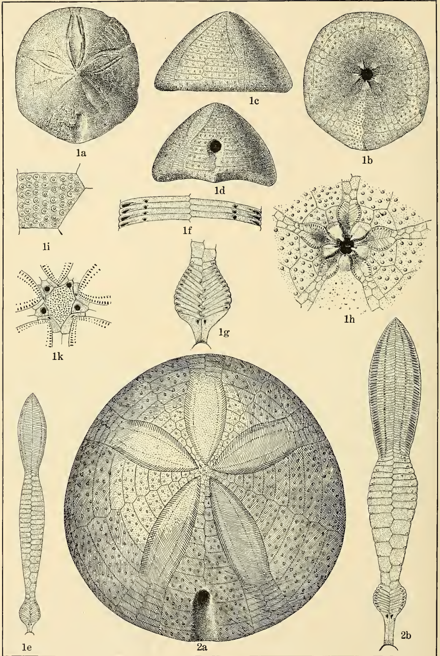
CRETACEOUS ECHINOIDEA.
