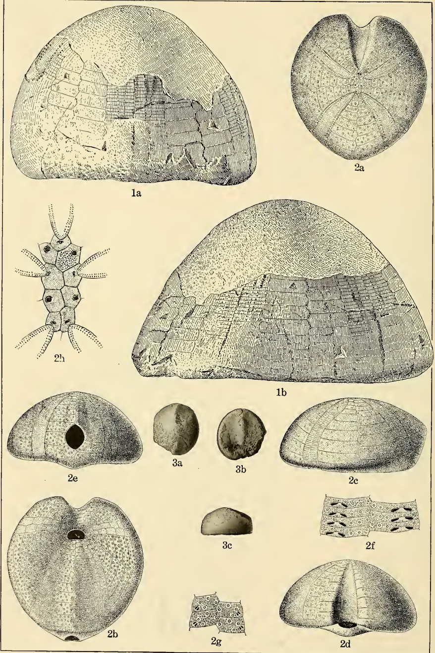
CRETACEOUS ECHINOIDEA.
