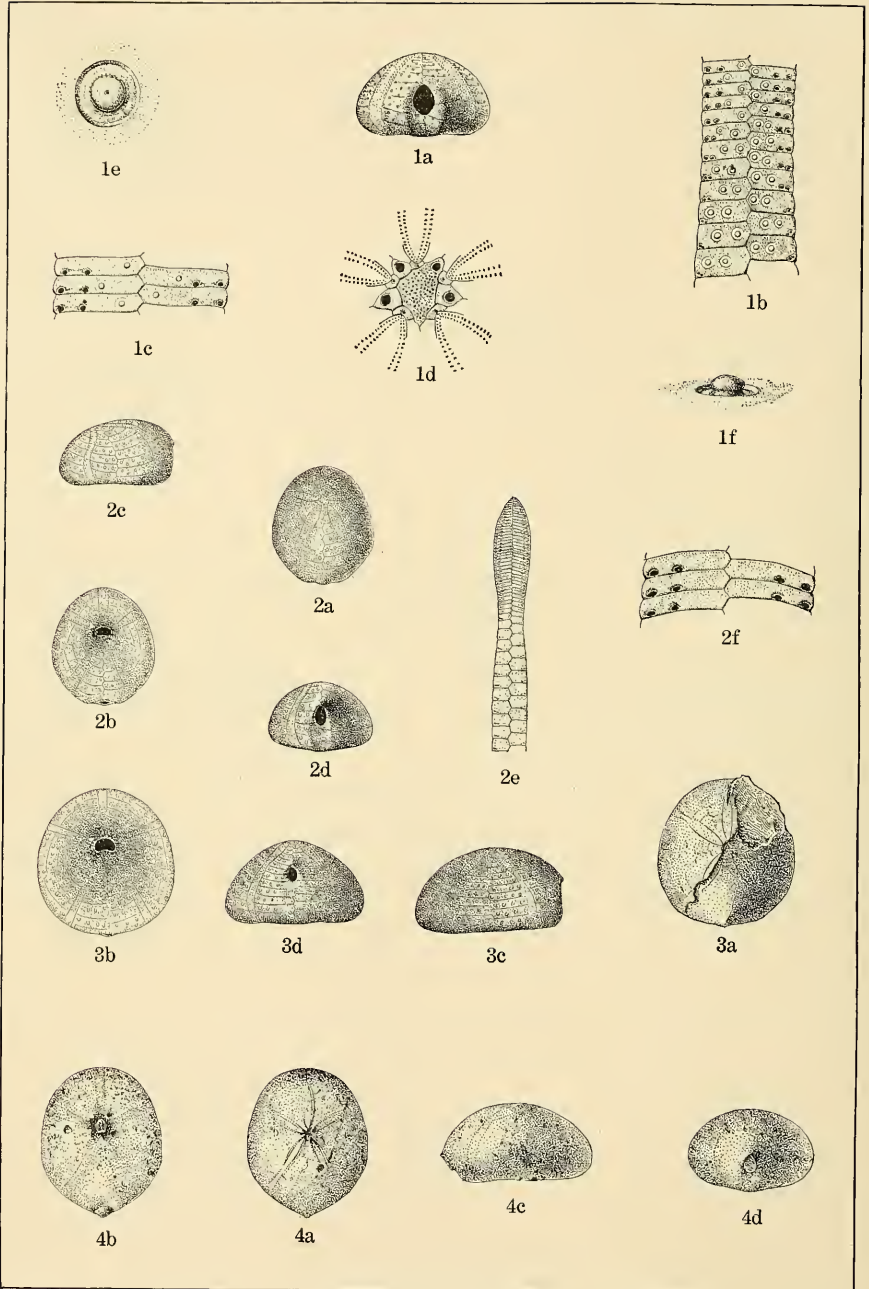
CRETACEOUS ECHINOIDEA.
