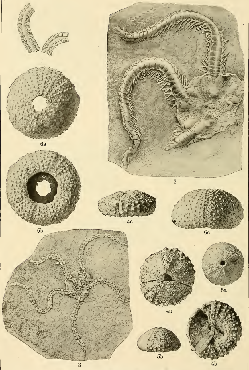
MIOCENE STELLEROIDEA AND ECHINOIDEA.
