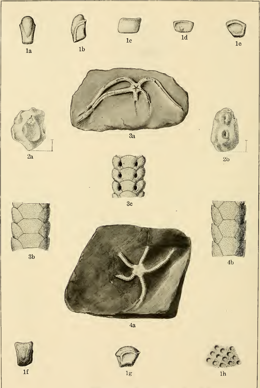
CRETACEOUS STELLEROIDEA.
