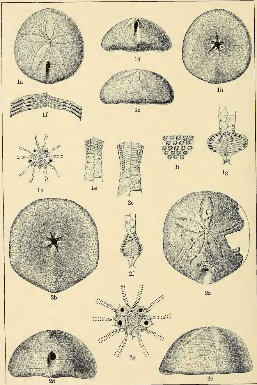
CRETACEOUS ECHINOIDEA.
