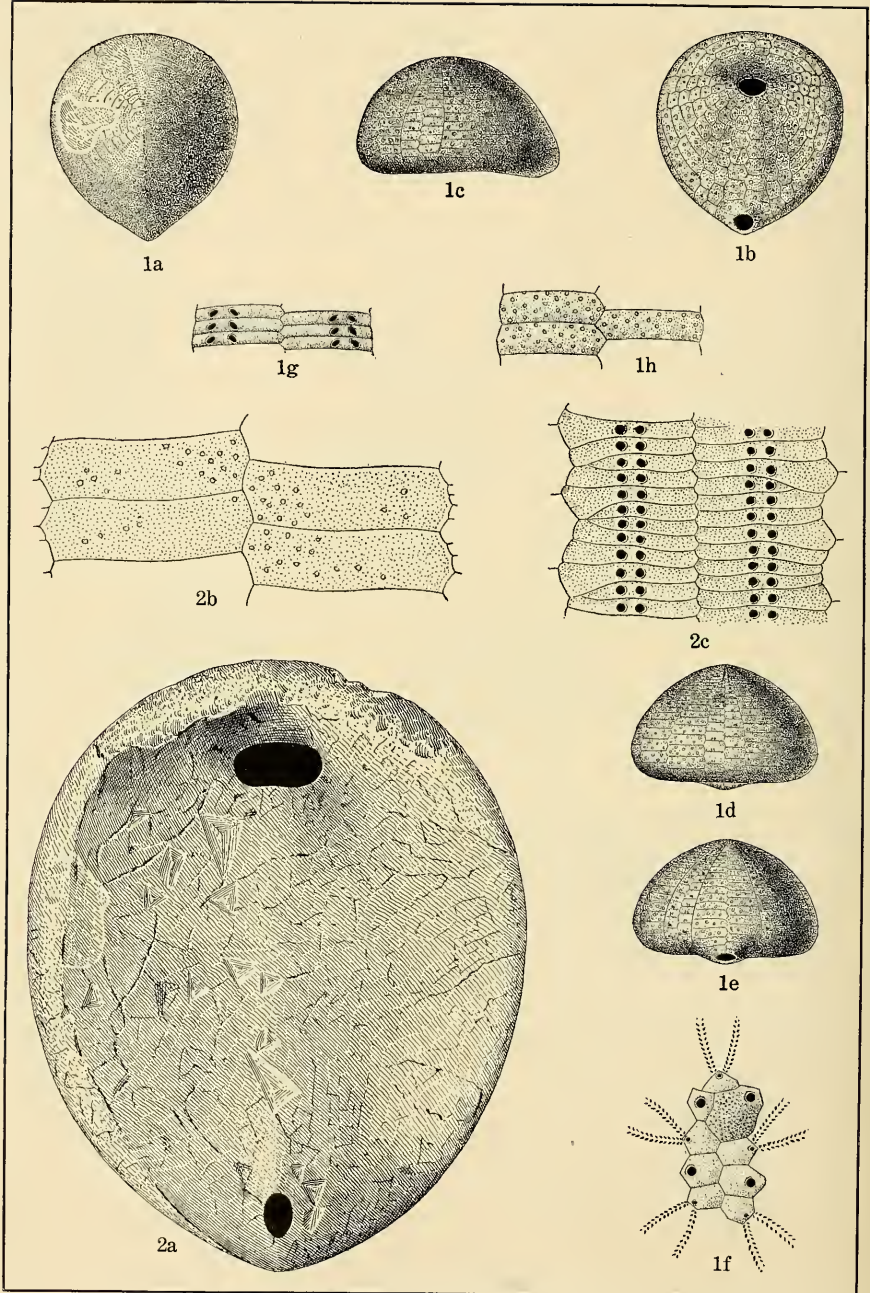
CRETACEOUS ECHINOIDEA.
