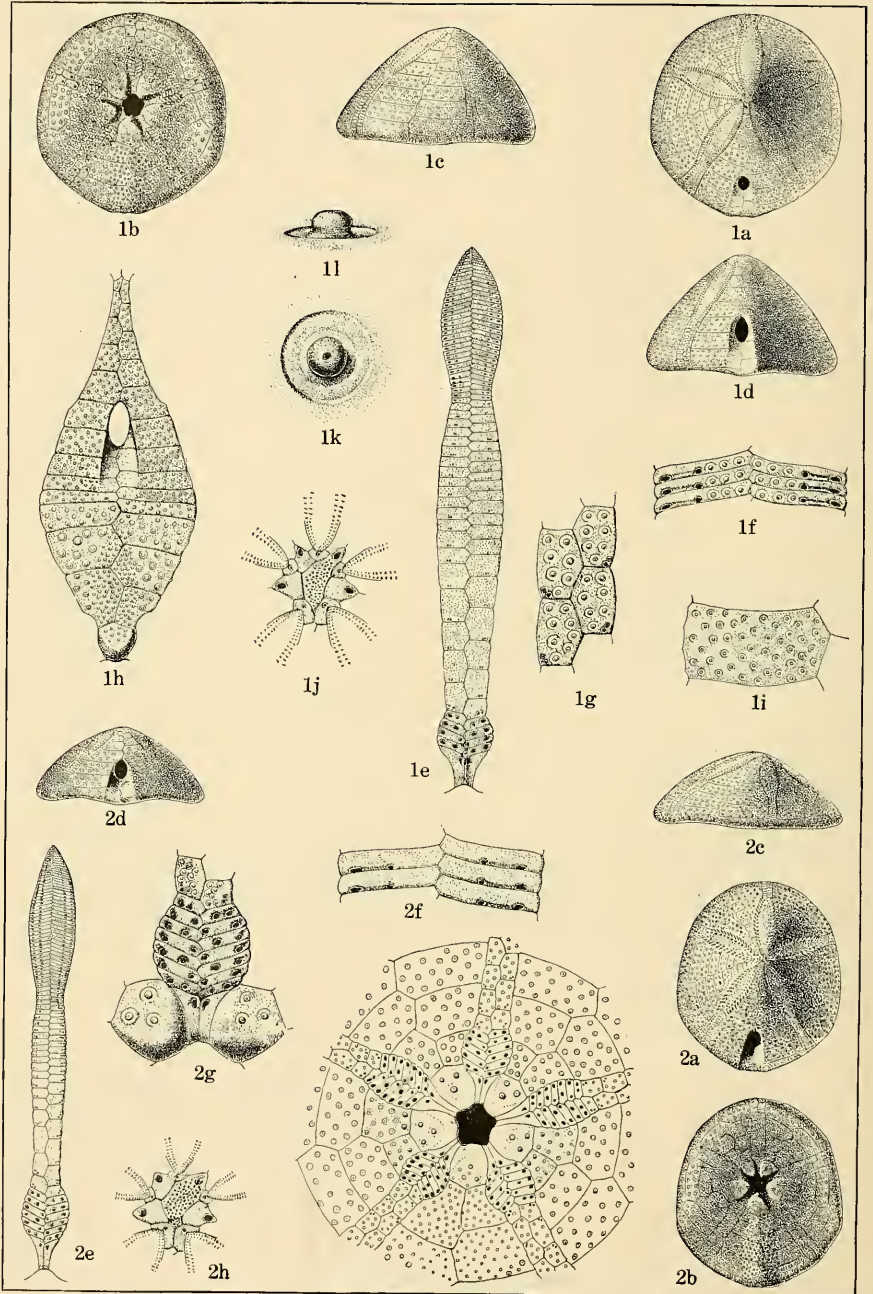
CRETACEOUS ECHINOIDEA.
