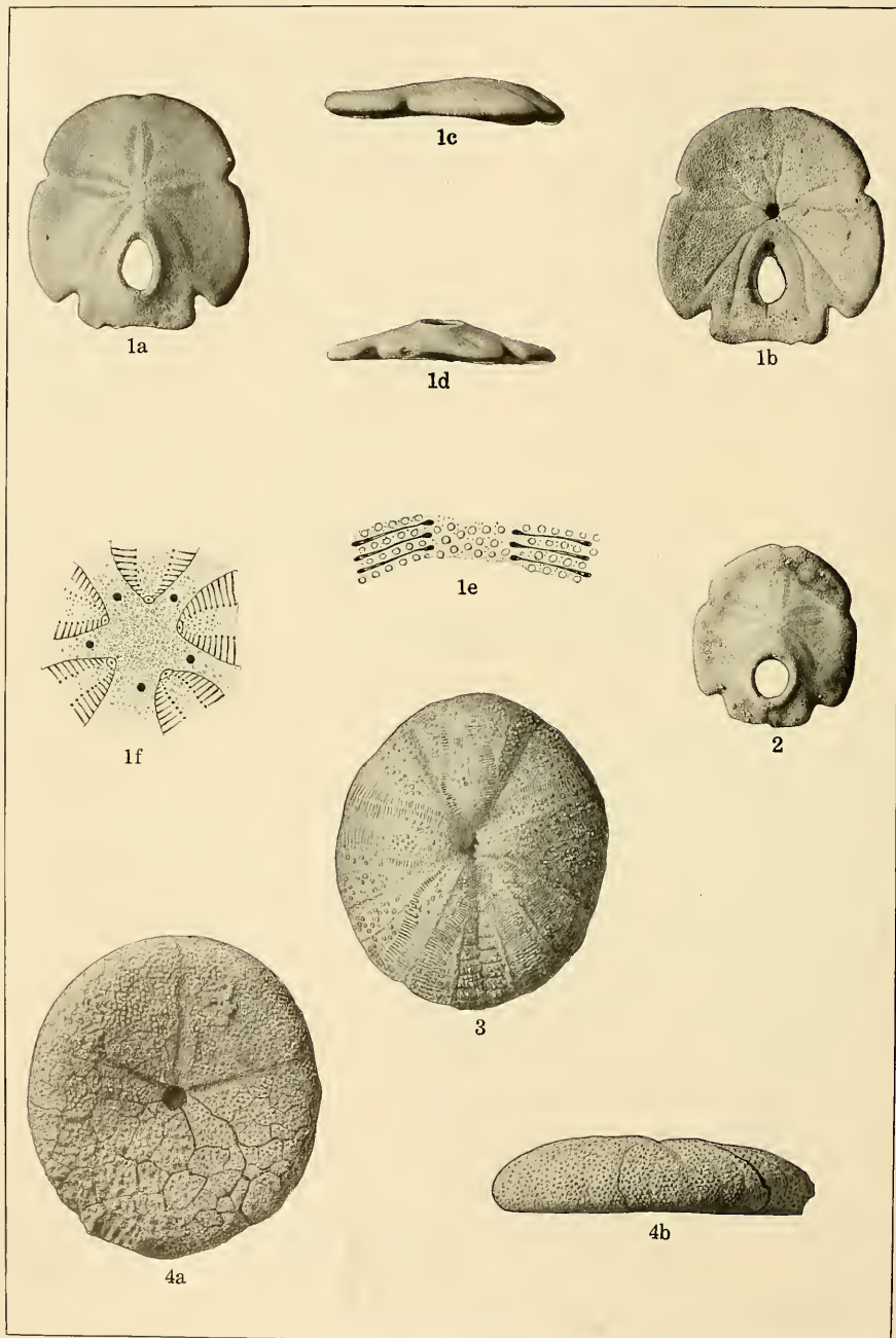
MIocene ECHINOIDEA.
