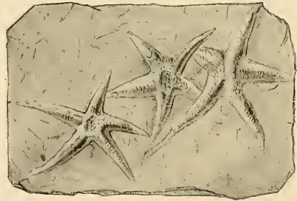
JURASSIC CRINOIDEA AND STELLEROIDEA.
