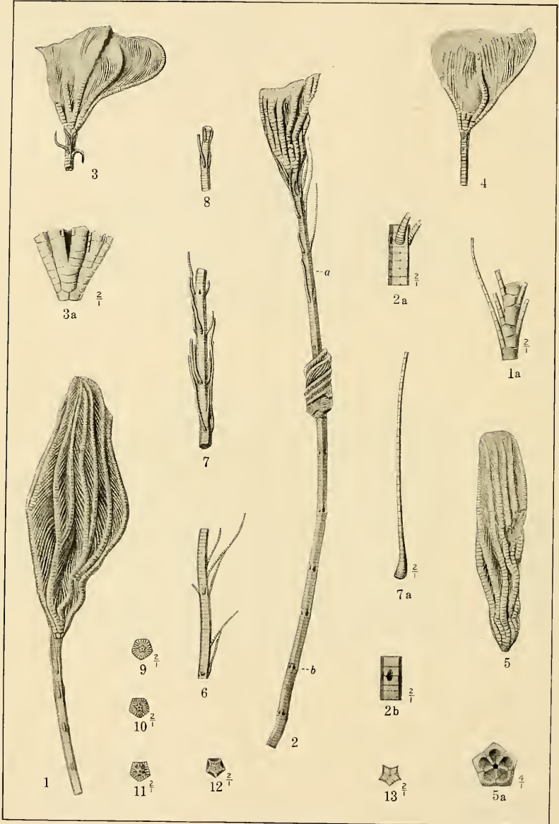
JURASSIC CRINOIDEA.
