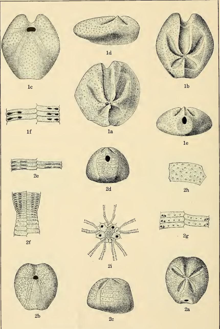
CRETACEOUS ECHINOIDEA.
