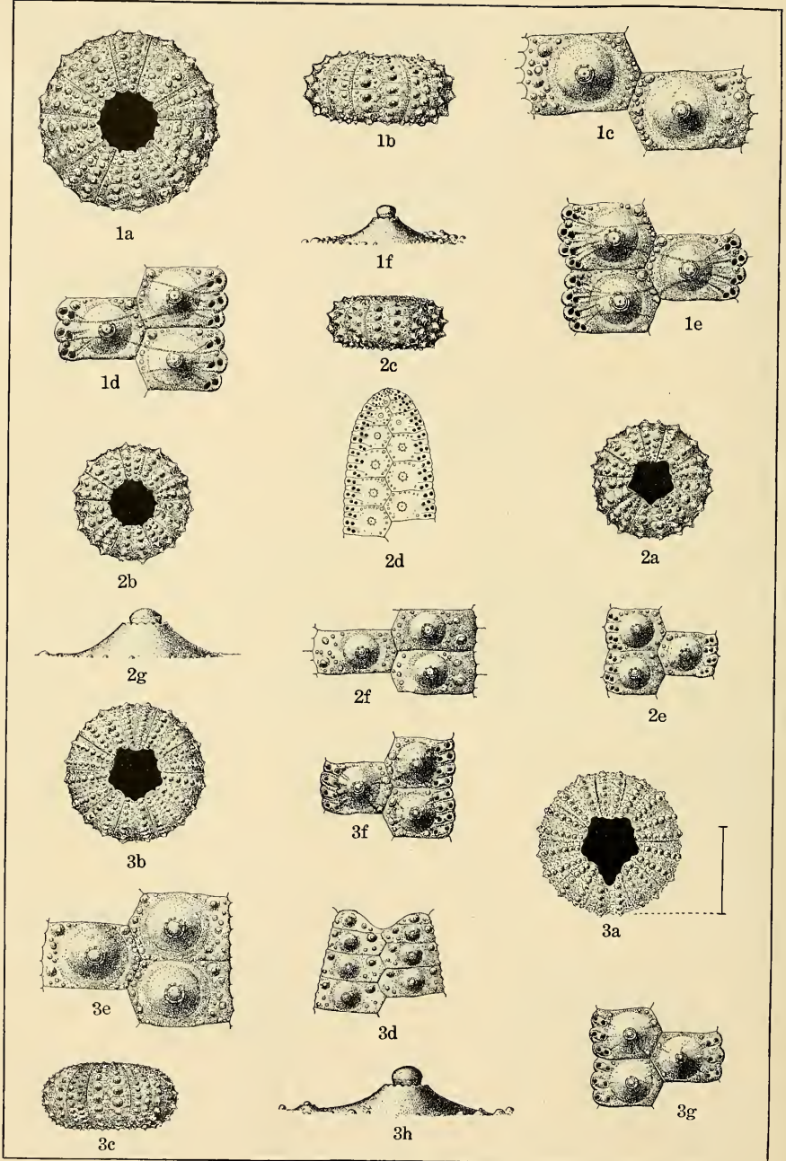
CRETACEOUS ECHINOIDEA.
