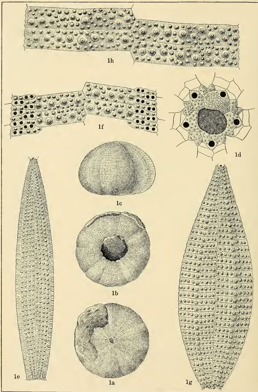
CRETACEOUS ECHINOIDEA.
