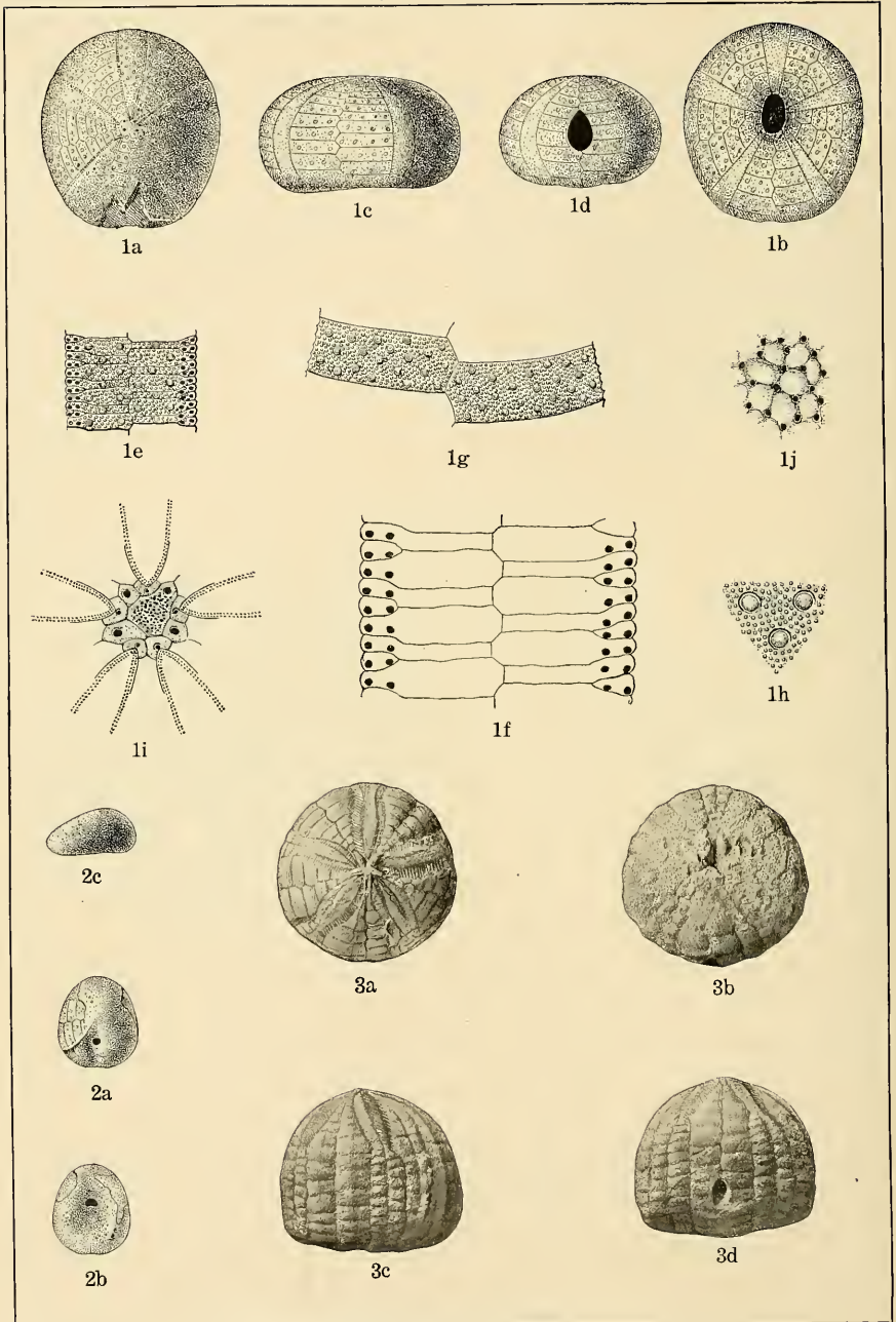
CRETACEOUS ECHINOIDEA.
