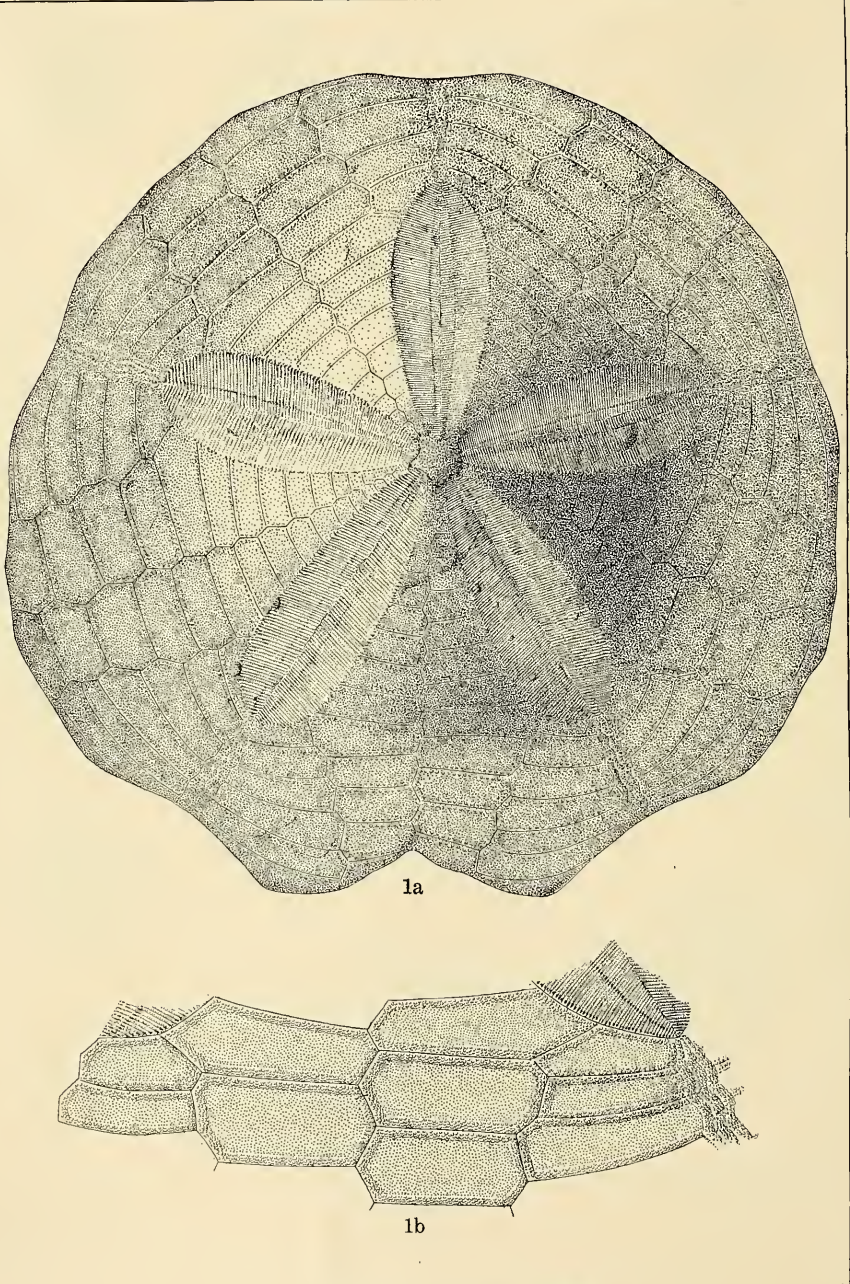
MIOCENE ECHINOIDEA.
