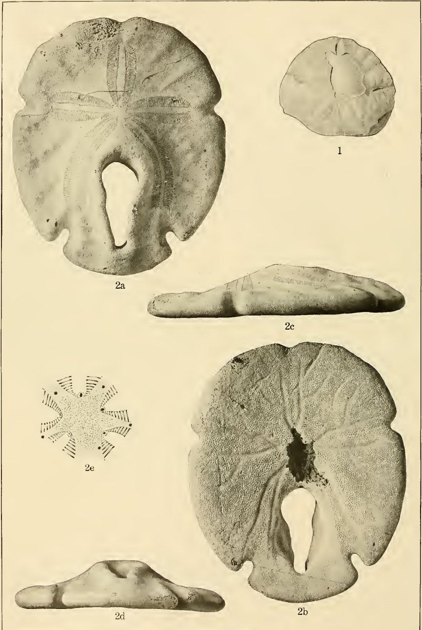
MIOCENE ECHINOIDEA.
