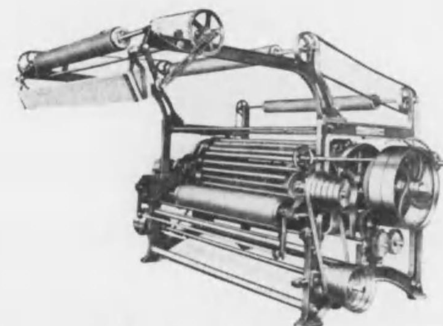
Wire-Card Raising Machine
