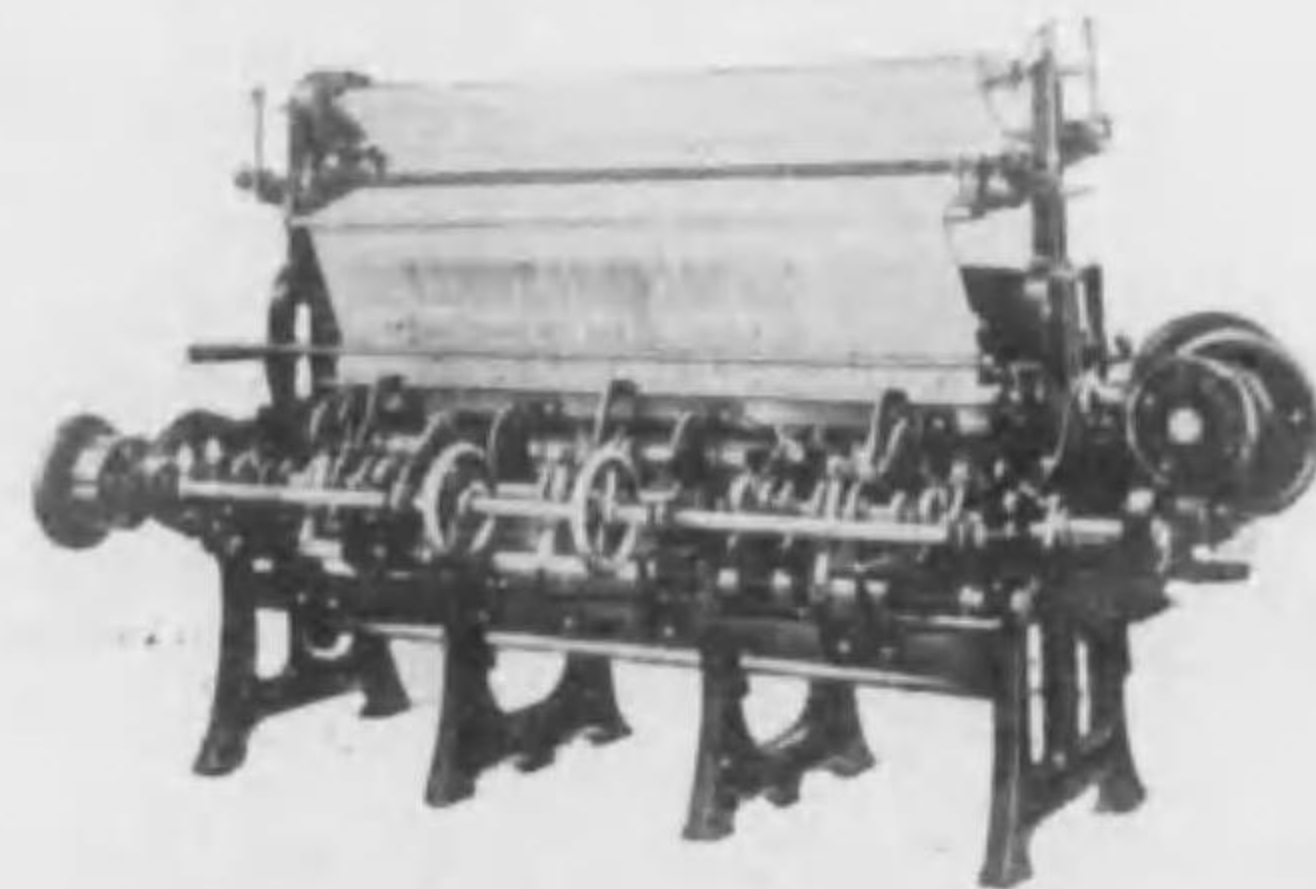
Double Warp Loom
