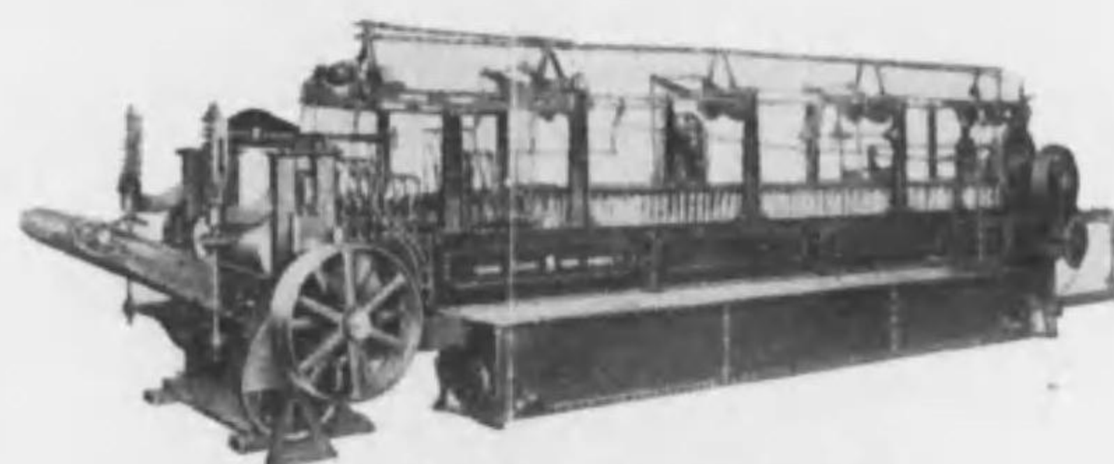
Mcnaught Self Cleaning Wool Washer with Self cleaning Apparatus
