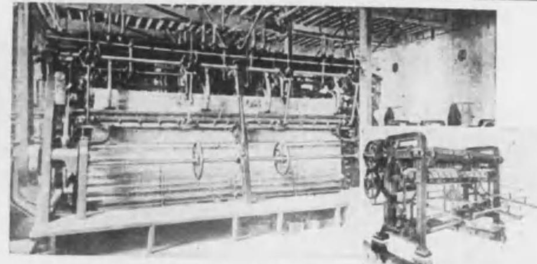
Go-Through Lace Machine
