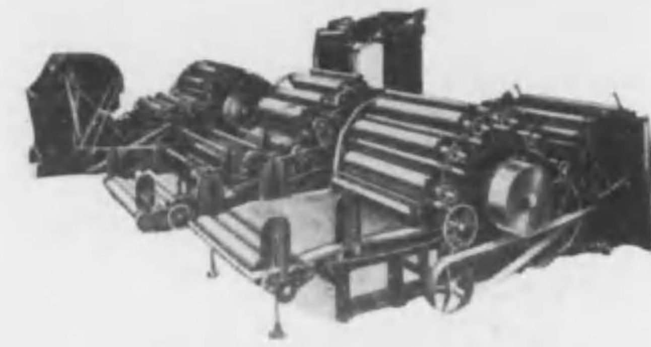
Gessner's Set of Three Carding Engine, Single Doffer Type.
