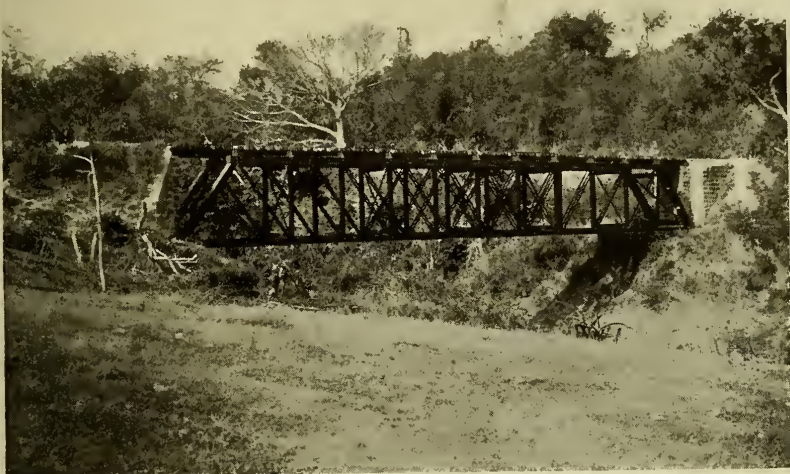
DECK BRIDGE ON SALVADOR RAILWAY.
