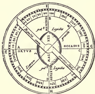
FIG. I.—AZIMUTH COMPASS
