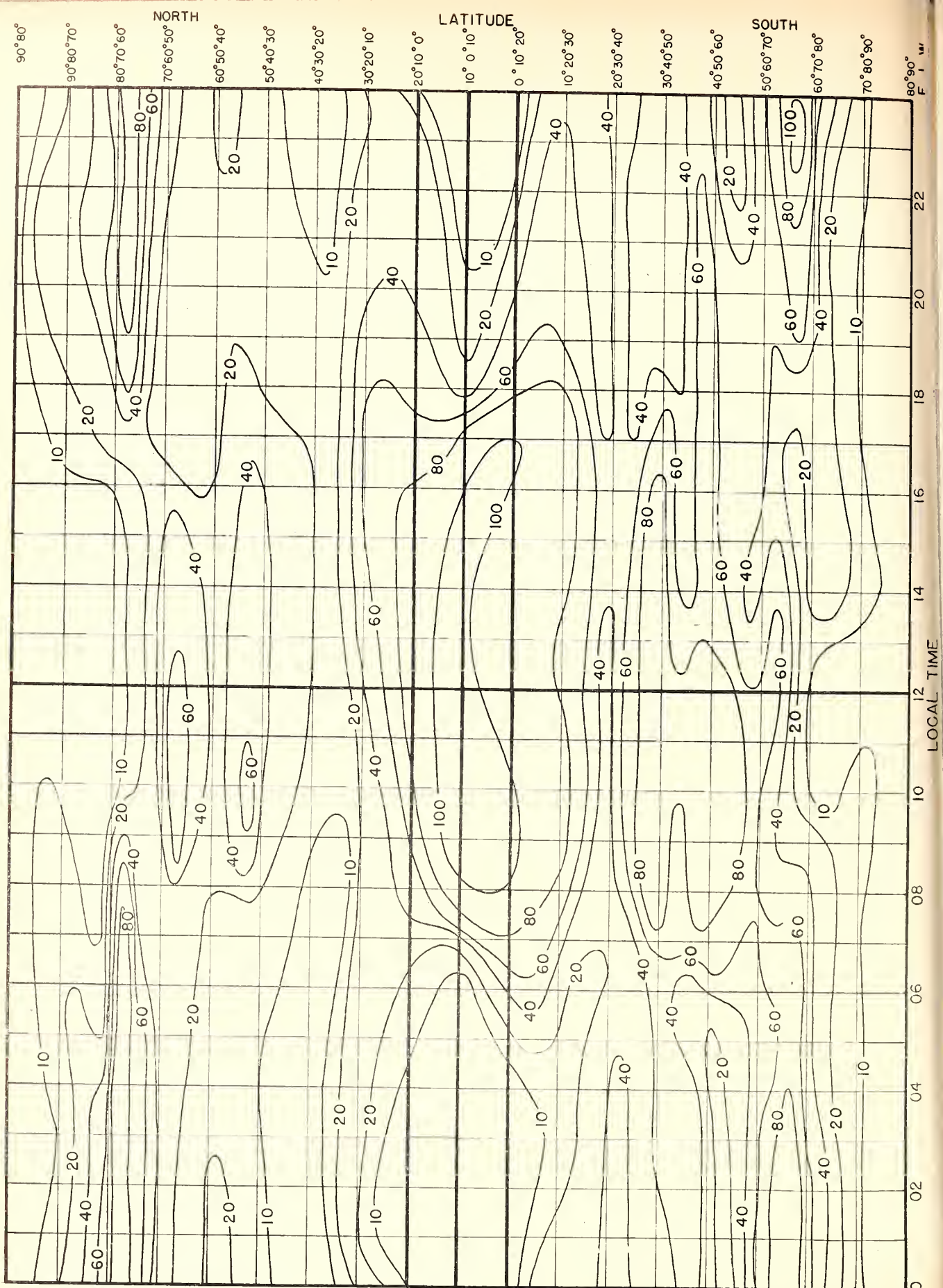
Fig. 15. PERCENTAGE OF TIME OCCURRENCE FOR E_s IN EXCESS OF 15 Mc, PREDICTED FOR FEBRUARY, 1946
