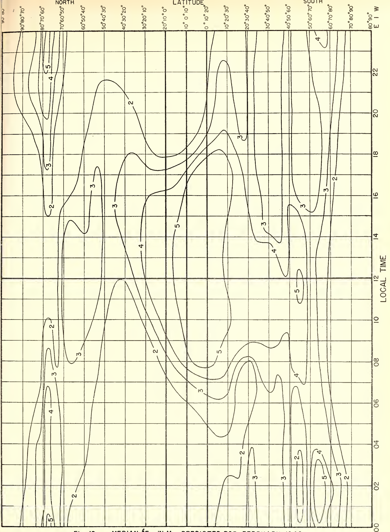
Fig. 12. MEDIAN fE_s , IN Mc, PREDICTED FOR FEBRUARY, 1946.
