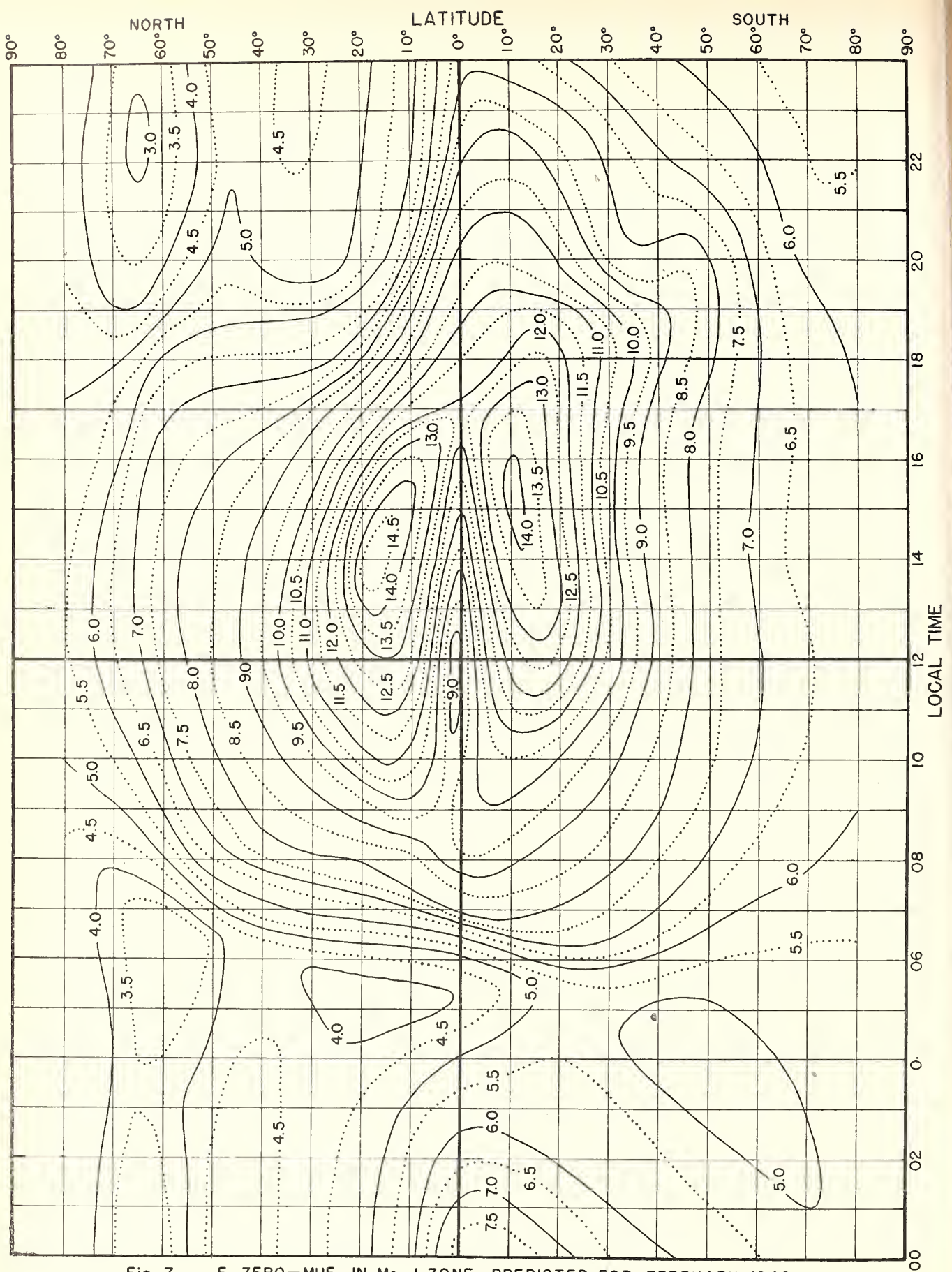
Fig. 7. F_2 ZERO-MUF, IN Mc, I ZONE, PREDICTED FOR FEBRUARY, 1946.
