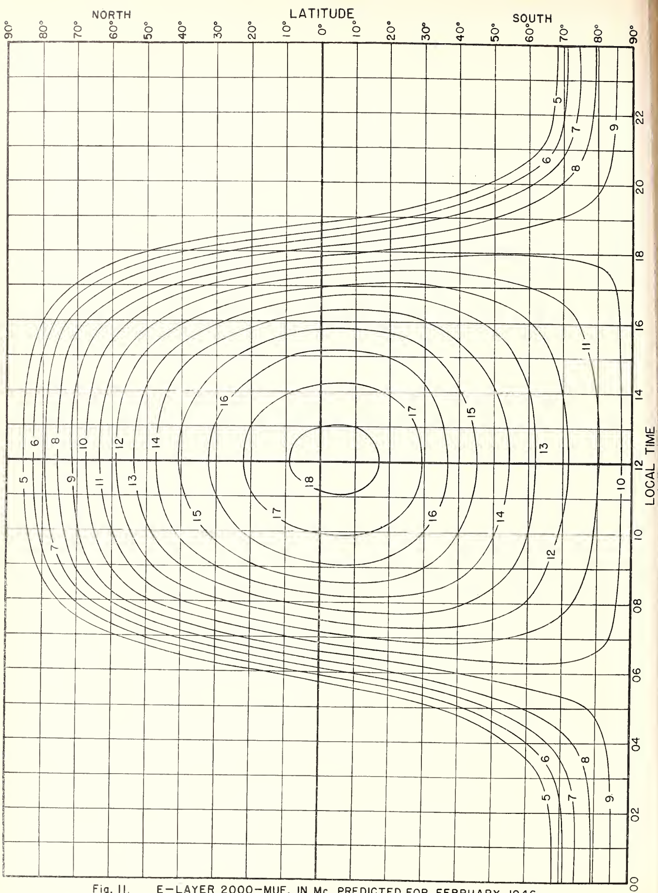
Fig. II. E-LAYER 2000-MUF, IN Mc, PREDICTED FOR FEBRUARY, 1946.
