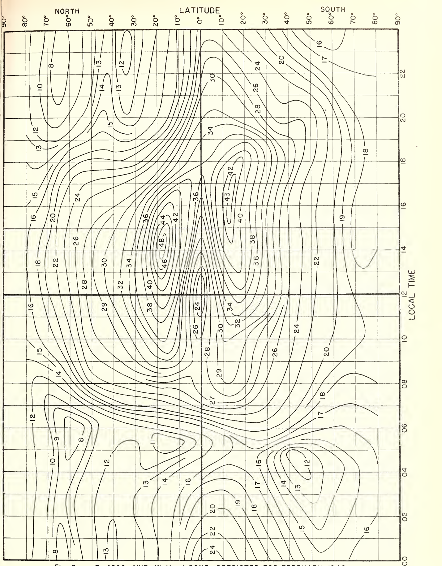
Fig. 8. F 2 4000-MUF, IN Mc, I ZONE, PREDICTED FOR FEBRUARY, 1946.
