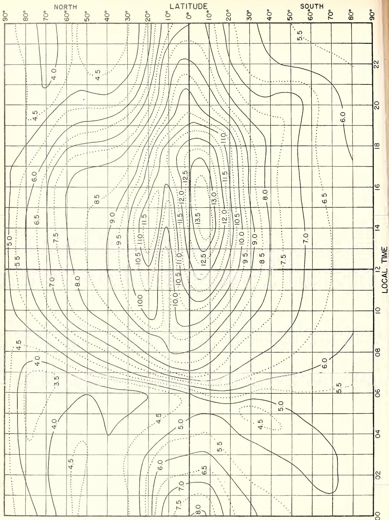
Fig. 9. F_2 ZERO-MUF, IN Mc, E ZONE, PREDICTED FOR FEBRUARY, 1946.
