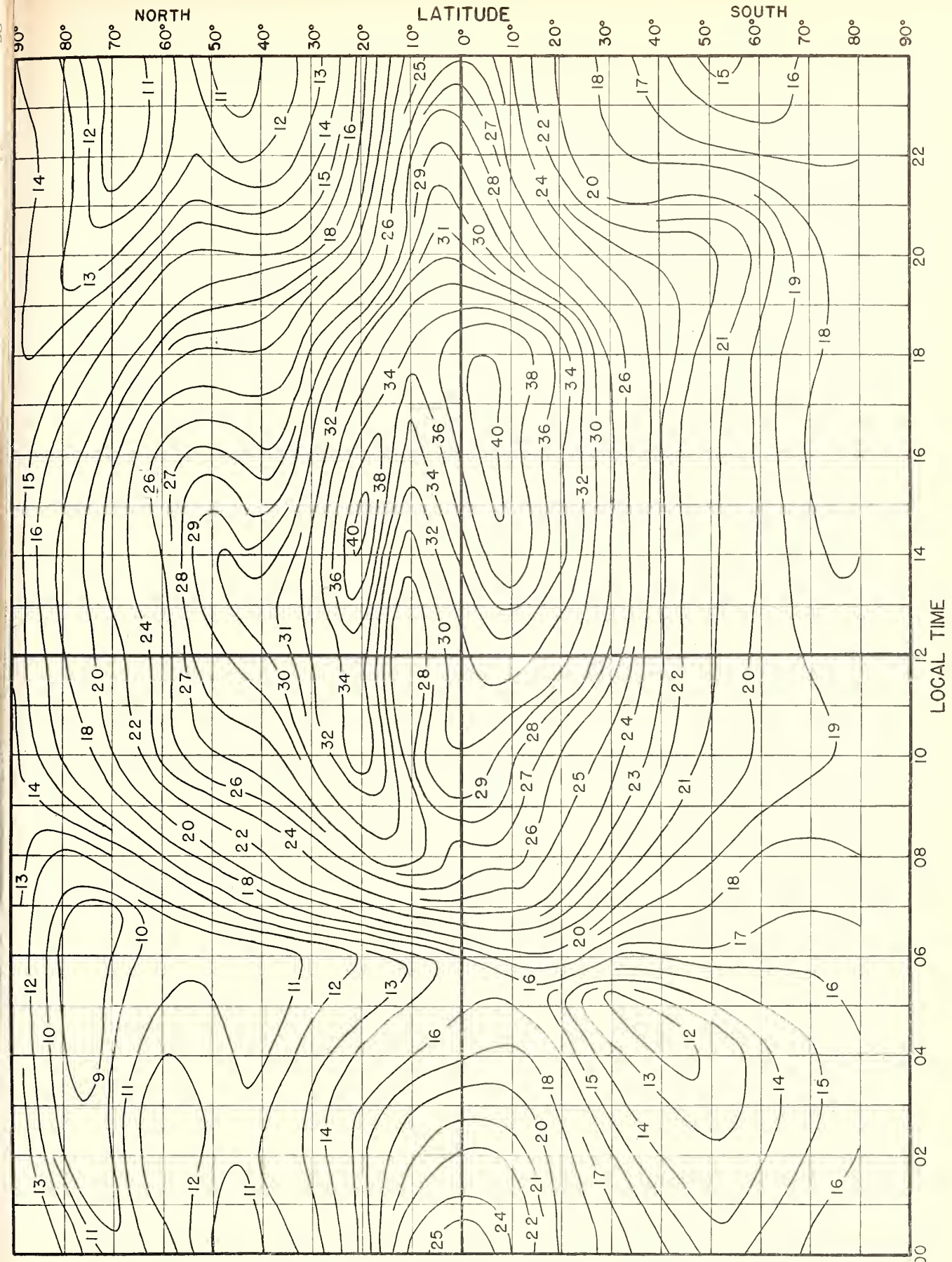
Fig. 10. F 2 4000-MUF, IN Mc, E ZONE, PREDICTED FOR FEBRUARY, 1946.
