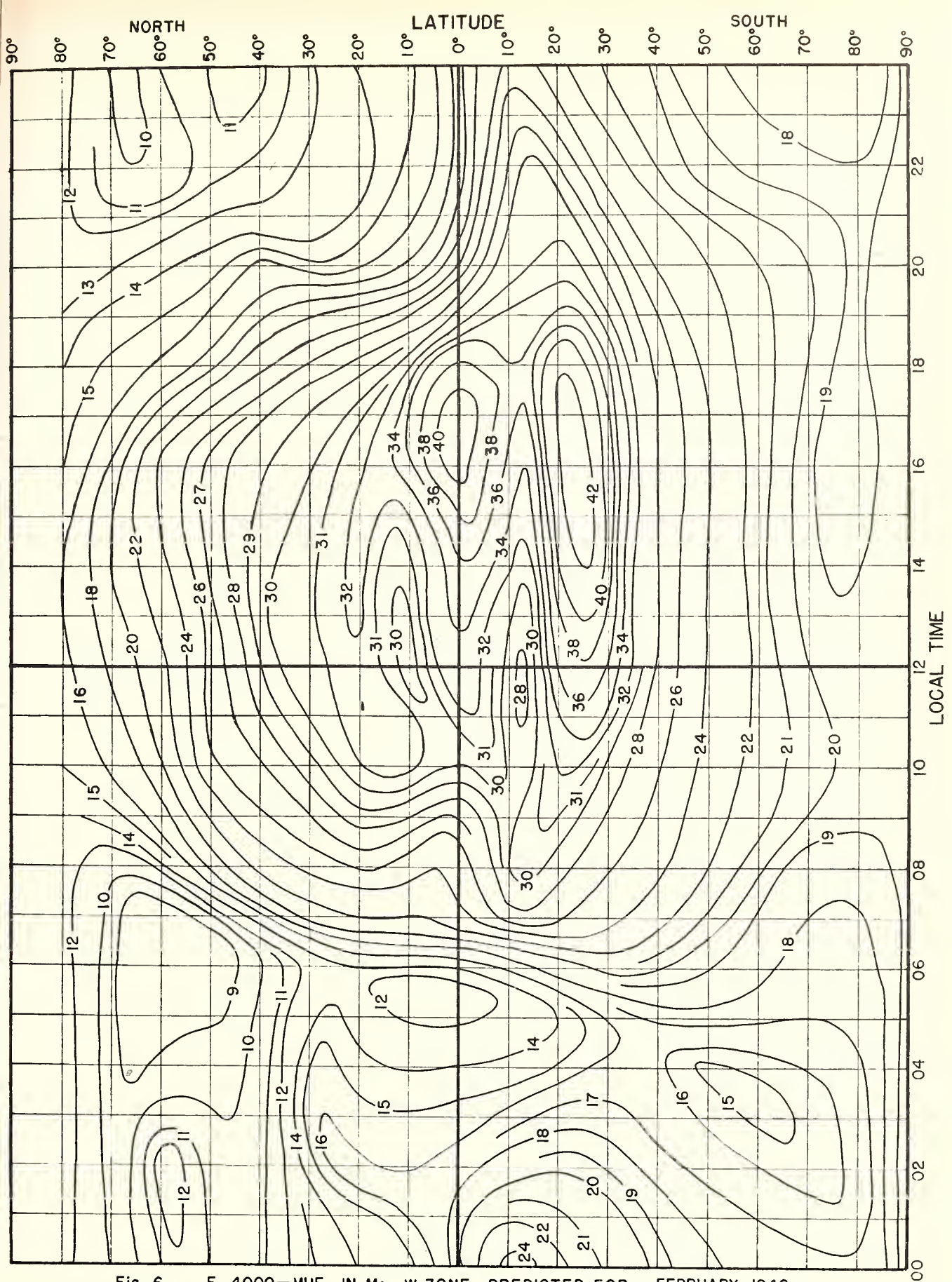
Fig. 6. F 2 4000-MUF, IN Mc, W ZONE, PREDICTED FOR FEBRUARY, 1946.
