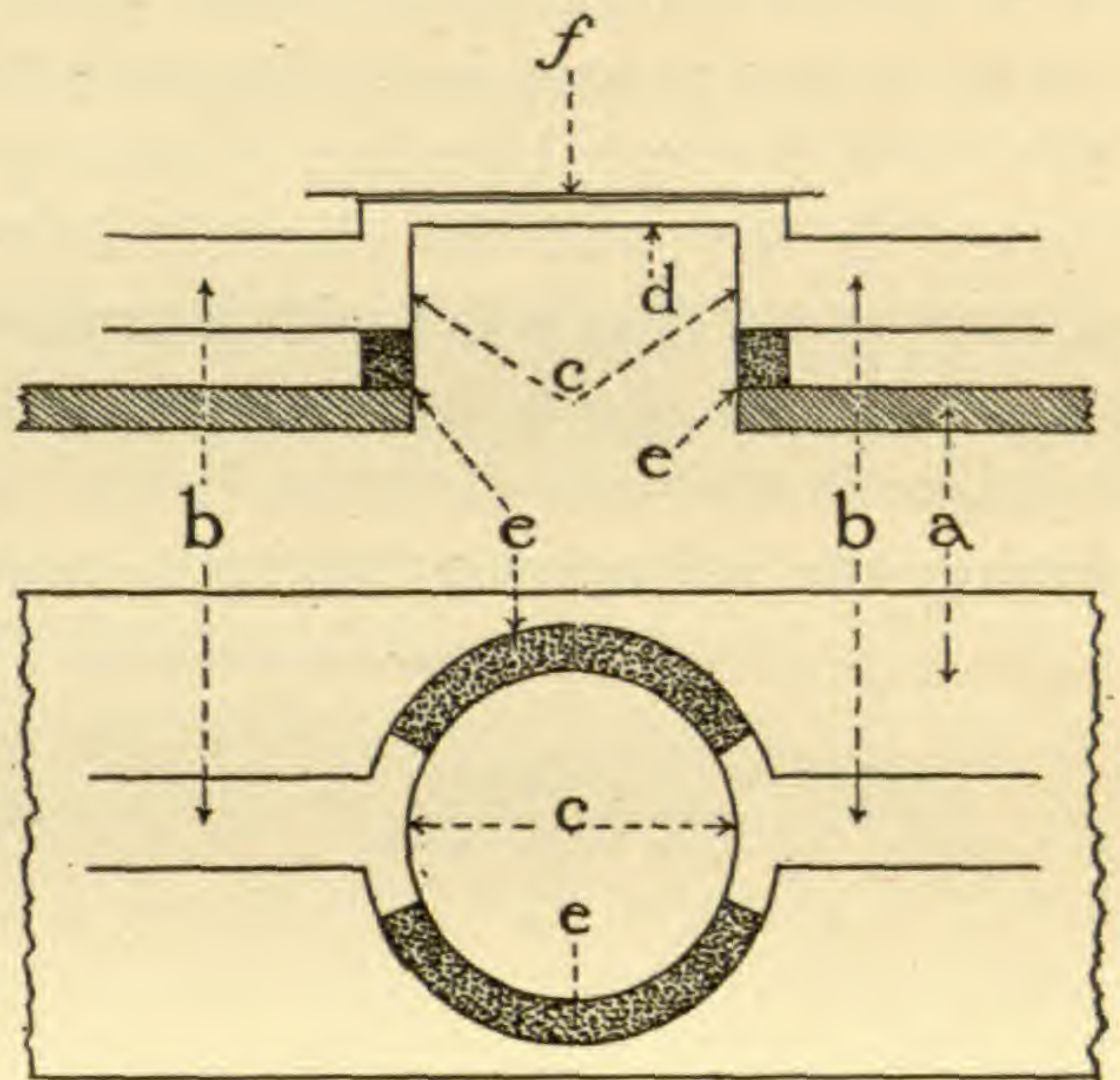
FIG. 1.—Sectional views of irrigation chamber: a , slide; b , inlet and outlet tubes; c , glass cylinder; d , glass plate; f , cover glass (upper line) and material (lower line).
