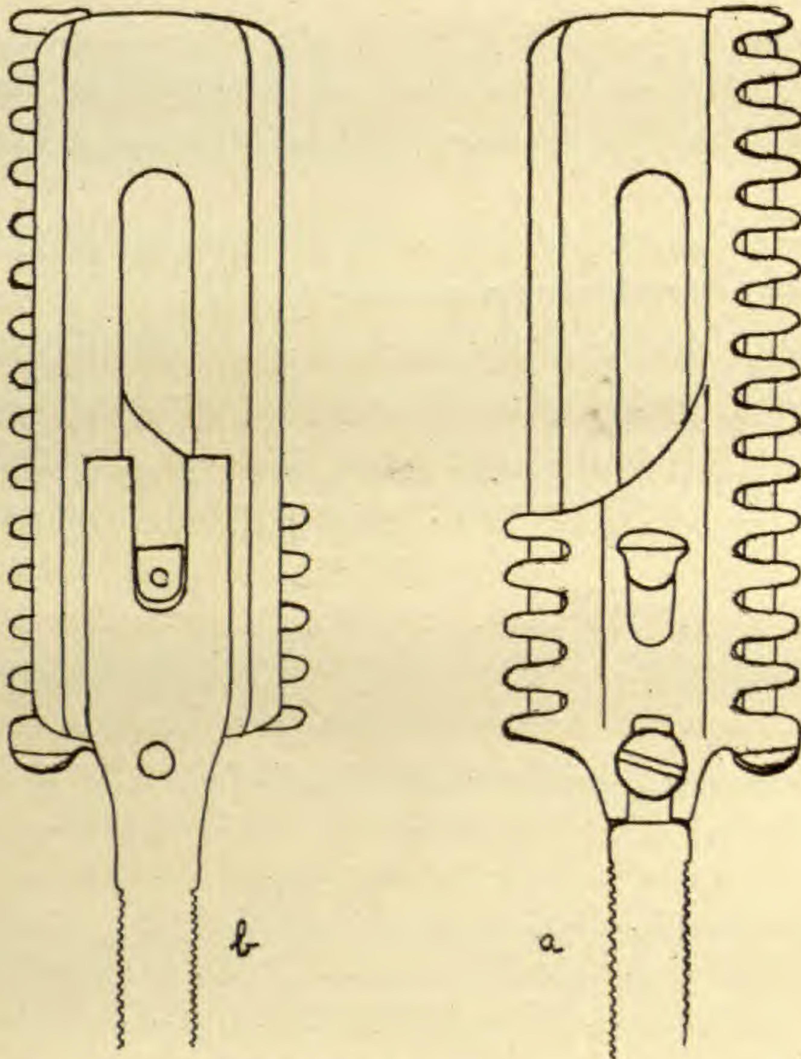
FIG. 1.—Modified safety razor: explained in text
