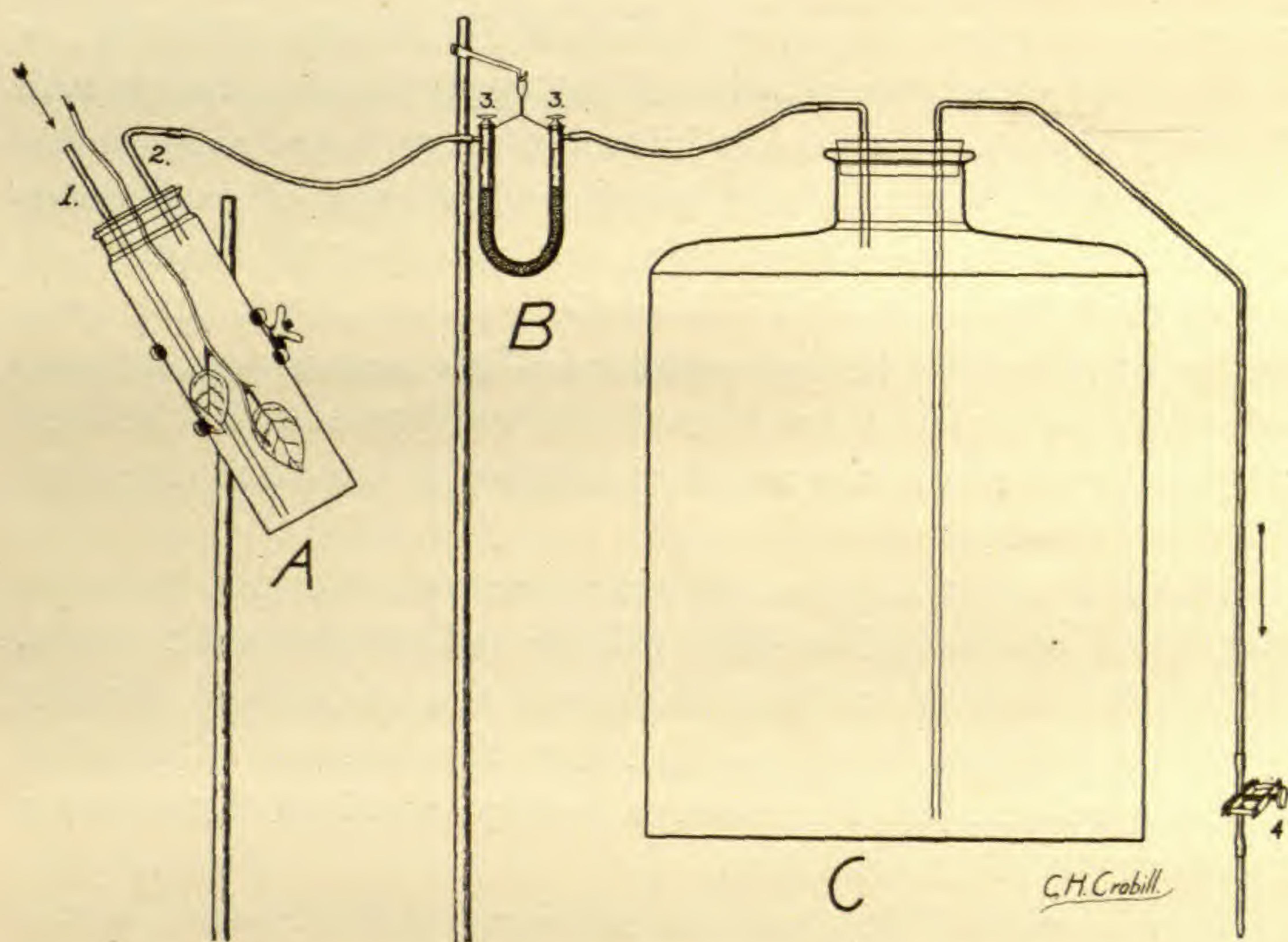
FIG. 1.—Apparatus for measuring transpiration: explained in text
