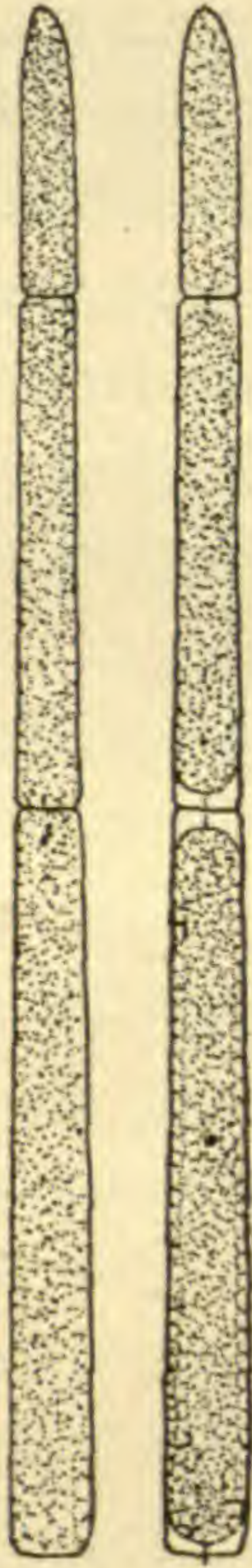
FIG. 6.—Surface view of the end of a hair of Polysiphonia violacea : at the left in natural condition; at the right after treatment for two minutes with distilled water (diagrammatic).
