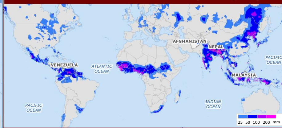
PRECIPITATION FORECAST FOR THE NEXT 7 DAYS (as of 20 July, NOAA)
