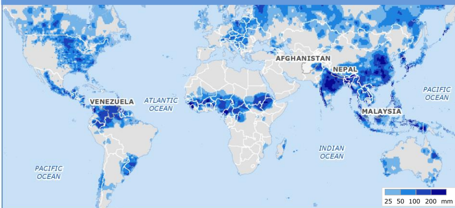
PRECIPITATION ACCUMULATION OVER THE LAST 15 DAYS (as of 19 July, NOAA)
