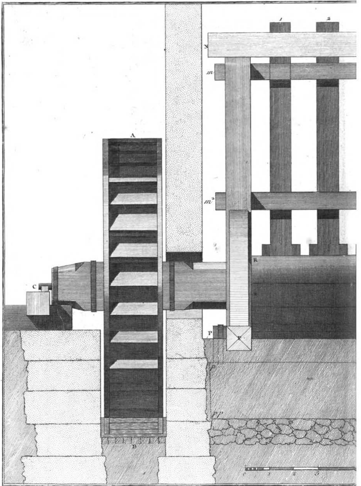
Tanneur, Elevation Att.
