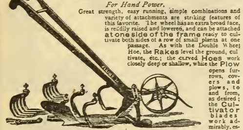
Fig. 9.—The "Planet Jr." Single Wheel Hoe Complete
