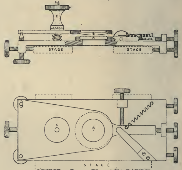
FIG. 1.—Section and plan of apparatus for applying pressure to coloured test-pieces.
