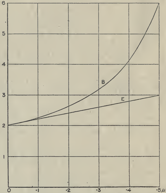
FIG. 1.—The ordinates of the curves show respectively the values of the coefficients E and B as multiples of the rigidity ( \mu ) in terms of Poisson's ratio ( \mu ).
