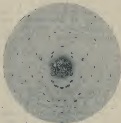
FIG. 1.—Adularia from St. Gotthard, plate parallel (001).
