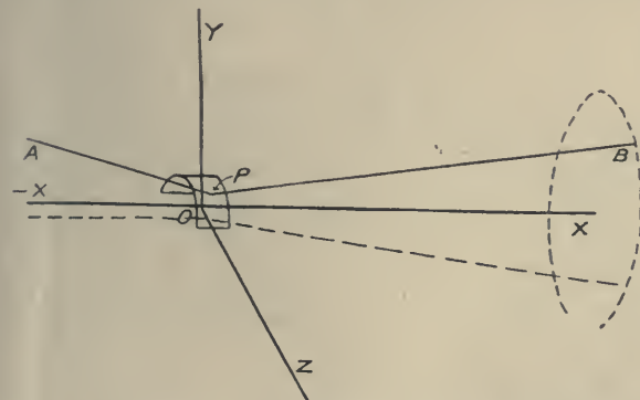
FIG. 1.—AP=incident ray; PB=reflected ray. Broken lines are projections on XZ plane of these rays; broken ring shows form of "halo" on a screen parallel to the YZ plane.
