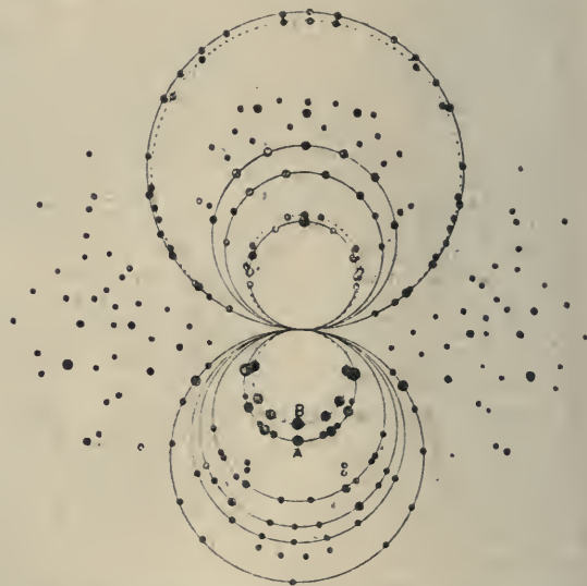
FIG. 4.—Stereographic projection of Laue spots of moonstone (001).
