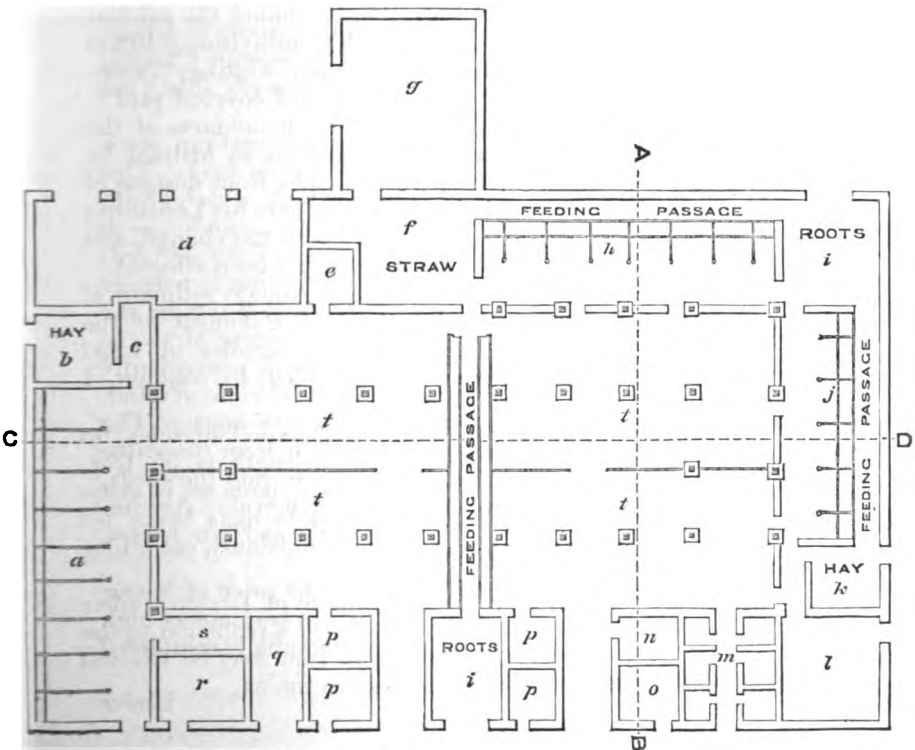
GROUND PLAN.
