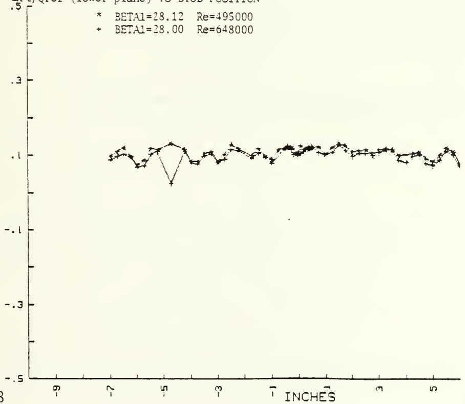
\Delta P_t/Q_{ref} (lower plane) VS BTOB POSITION
