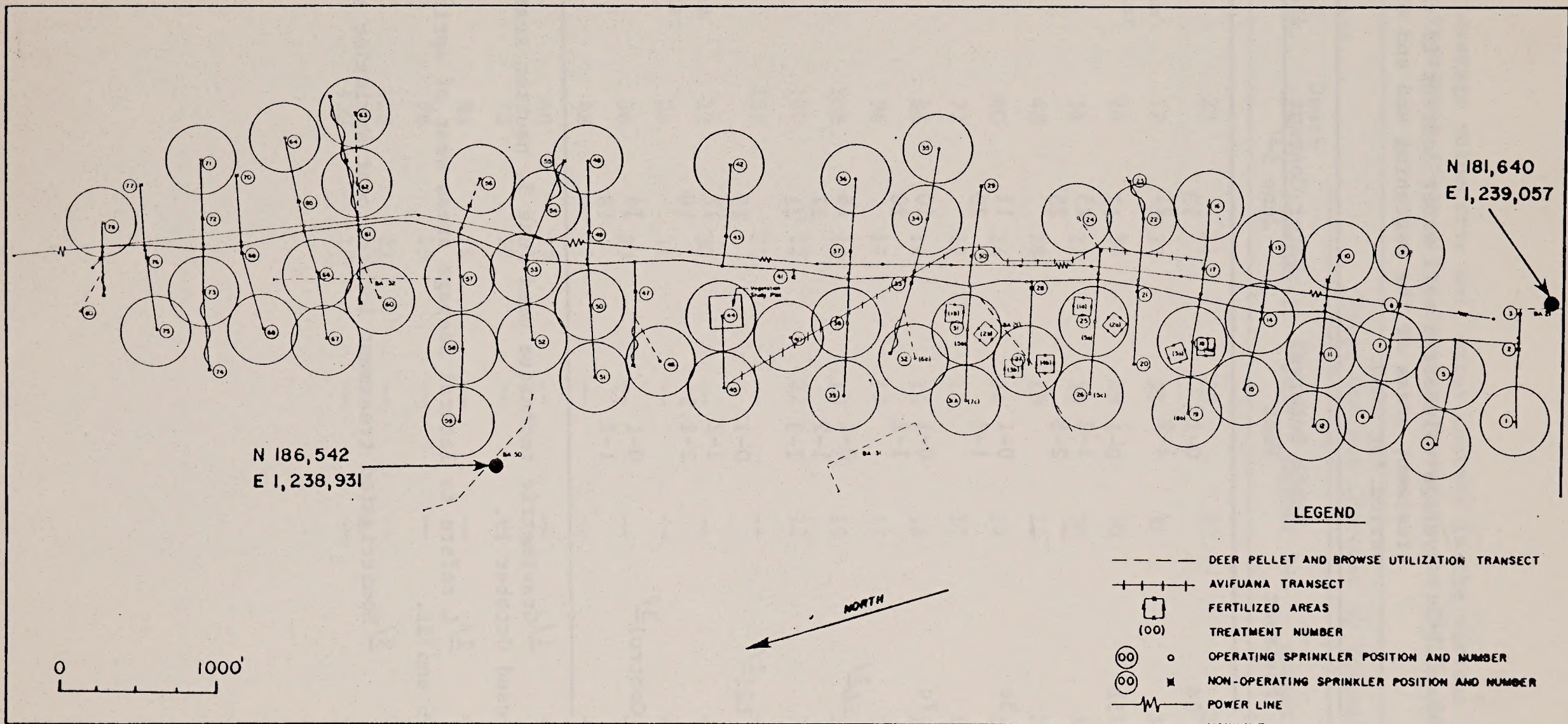
Figure A8.11.3-1 Map of C-b Tract irrigation system layout showing treatment locations.
