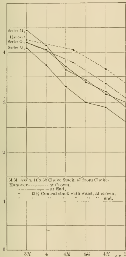
Fig. 5. American Engineer Tests of Locomotive Draft Appliances.
