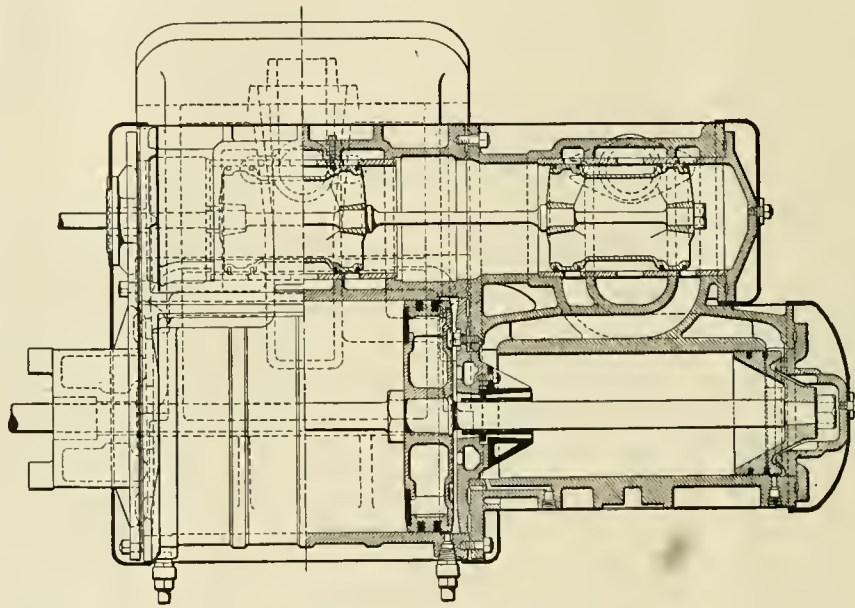
Section Through Cylinders and Steam Chests.
