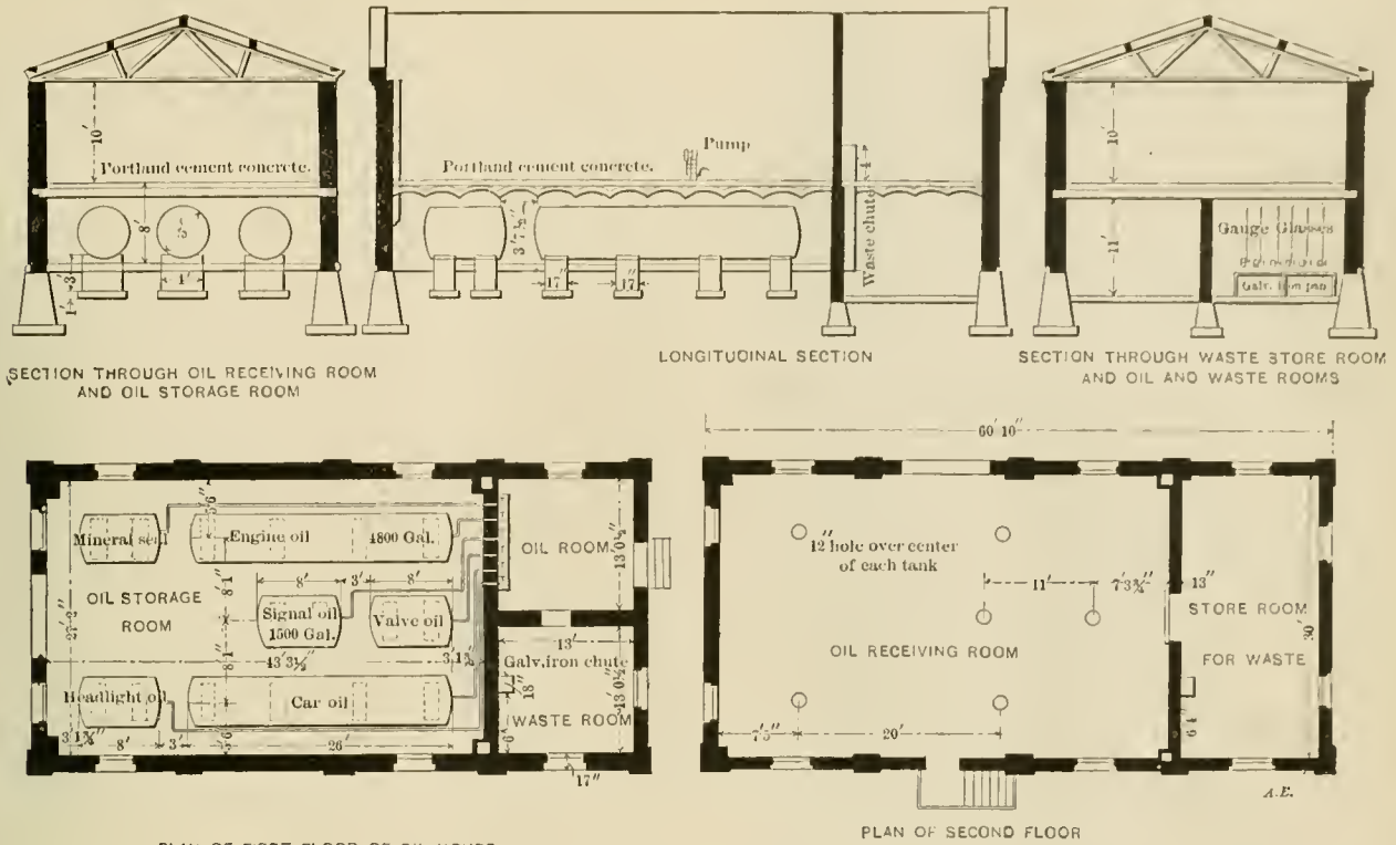
Oil House, Chicago, Indianapolis & Louisville Railway Lafayette, Ind.
