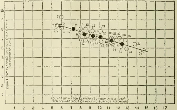
Fig. 3.—Rate of Evaporation and Efficiency.
