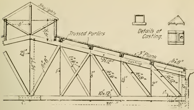
Roof of Blacksmith and Machine Shops.
