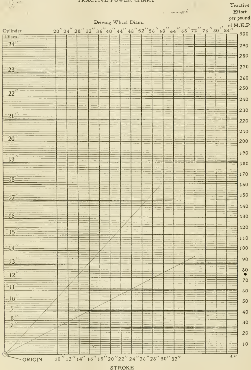
TRACTIVE POWER CHART
