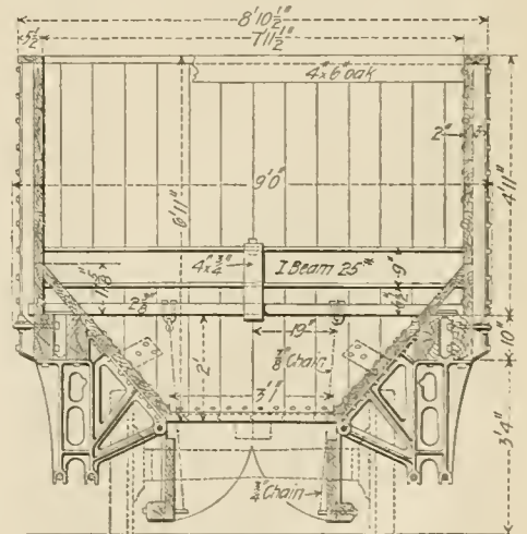
Section Through Hopper.
