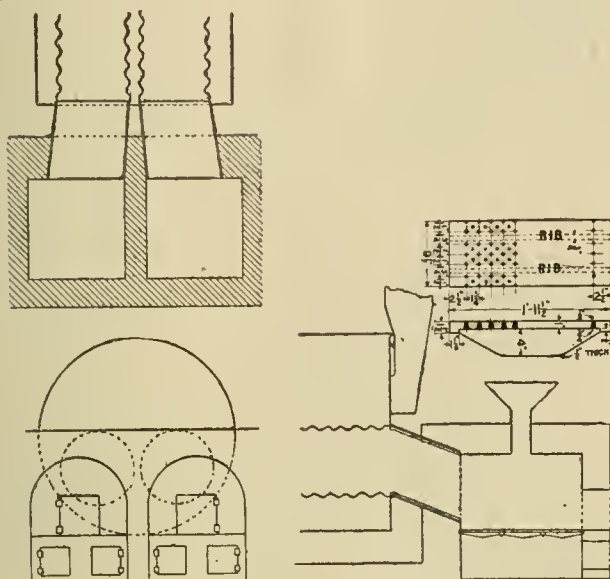
Arrangement of furnace for burning sawdust.
