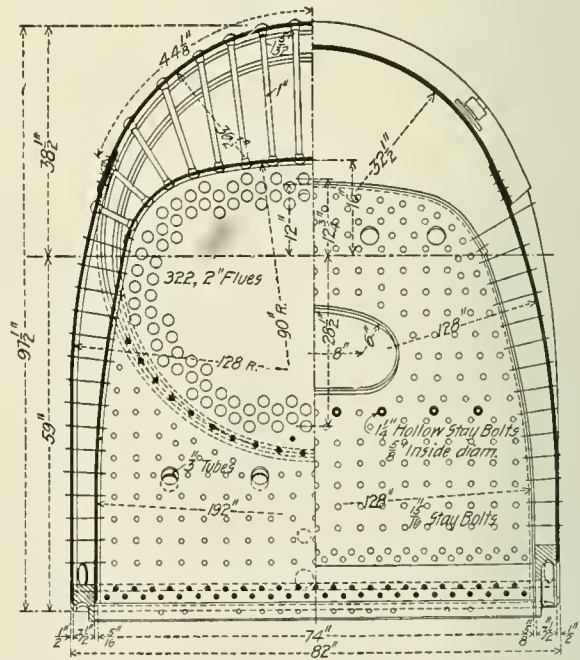
Sectional View of Firebox.
