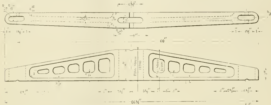
Cast-Steel Equalizer—Delaware Hudson Company.
