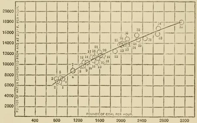
Fig. 5.—Combustion and Evaporation.
