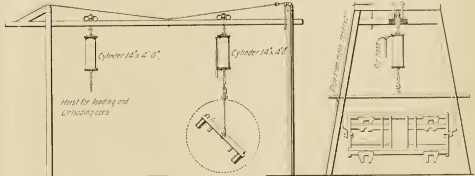
A Crane for Repairing Car Trucks.
