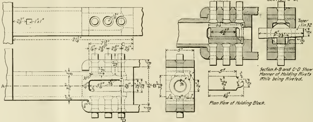
Proposed Butt for 5 x 7 in. Shank.
