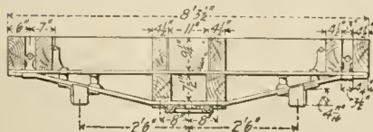
Transverse Section Near Body Bolster.
