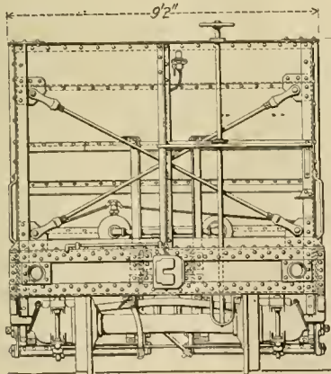
End elevation.
