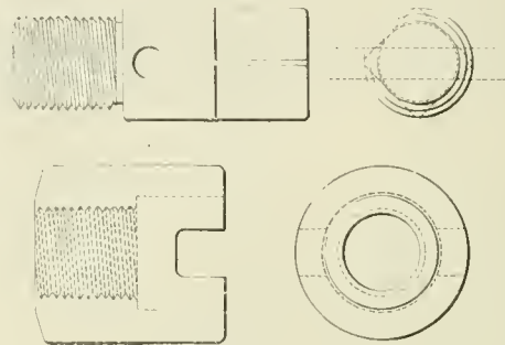
A "Stud Nut" for Staybolts.
