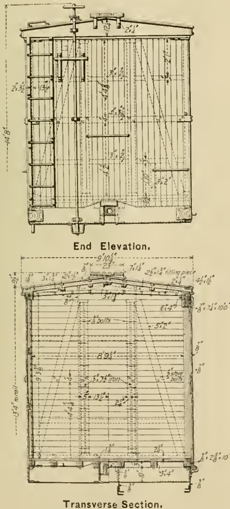
Fifty-Foot Furniture Car, with Steel Underframes—Erie Railroad.
