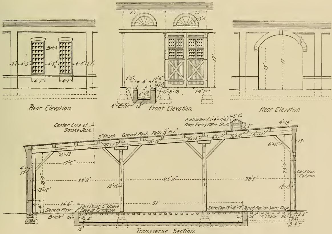
Sections and Details of Building.
