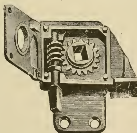
Fig. 2.—Roller Tightener.
