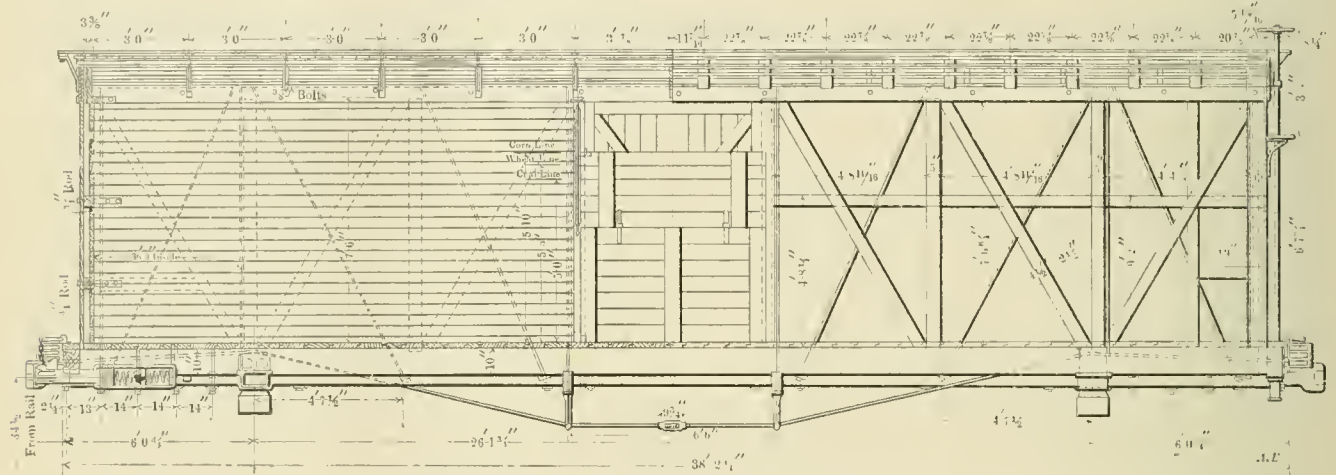
36-Foot, 40-Ton Box Car—Chesapeake & Ohio Railway.
