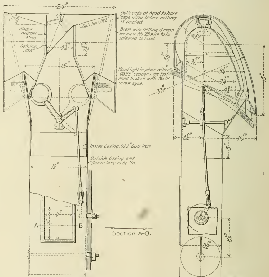
Fig. 2.—Arrangement of Intake Hood and Operating Device.
