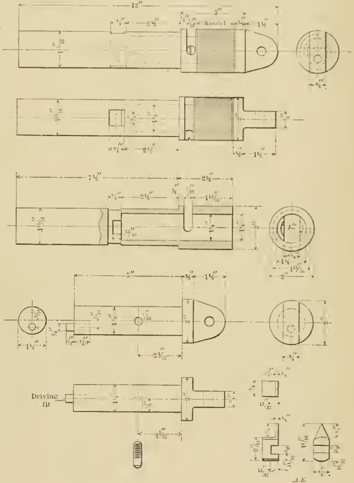
Tool for Cutting Out Boiler Flues.
