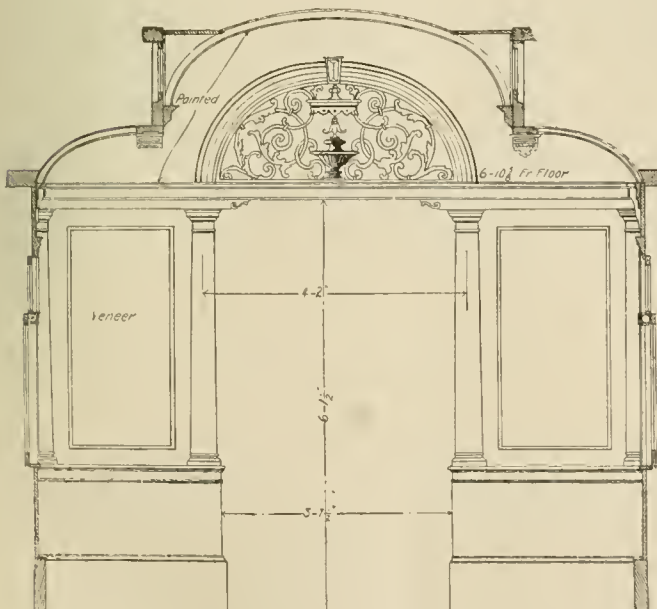
Bulkhead Partition.
