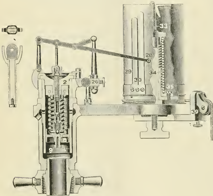
The Star Steam Engine Indicator.
