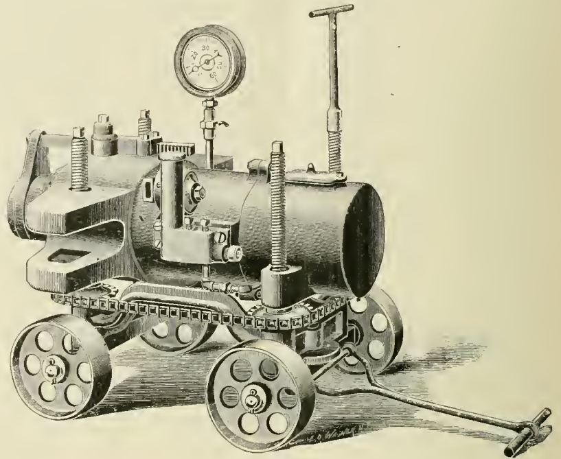
Improved Crank Pin Press.
