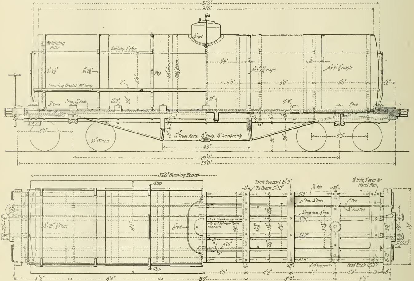
80,000 Pounds Capacity Tank Car—Atchison, Topeka & Santa Fe Railway.
