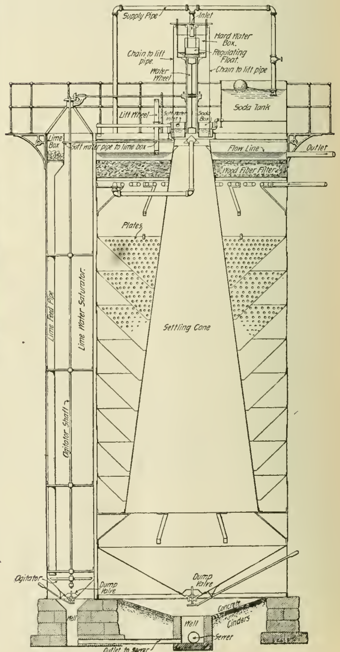
Section of Purifier.
