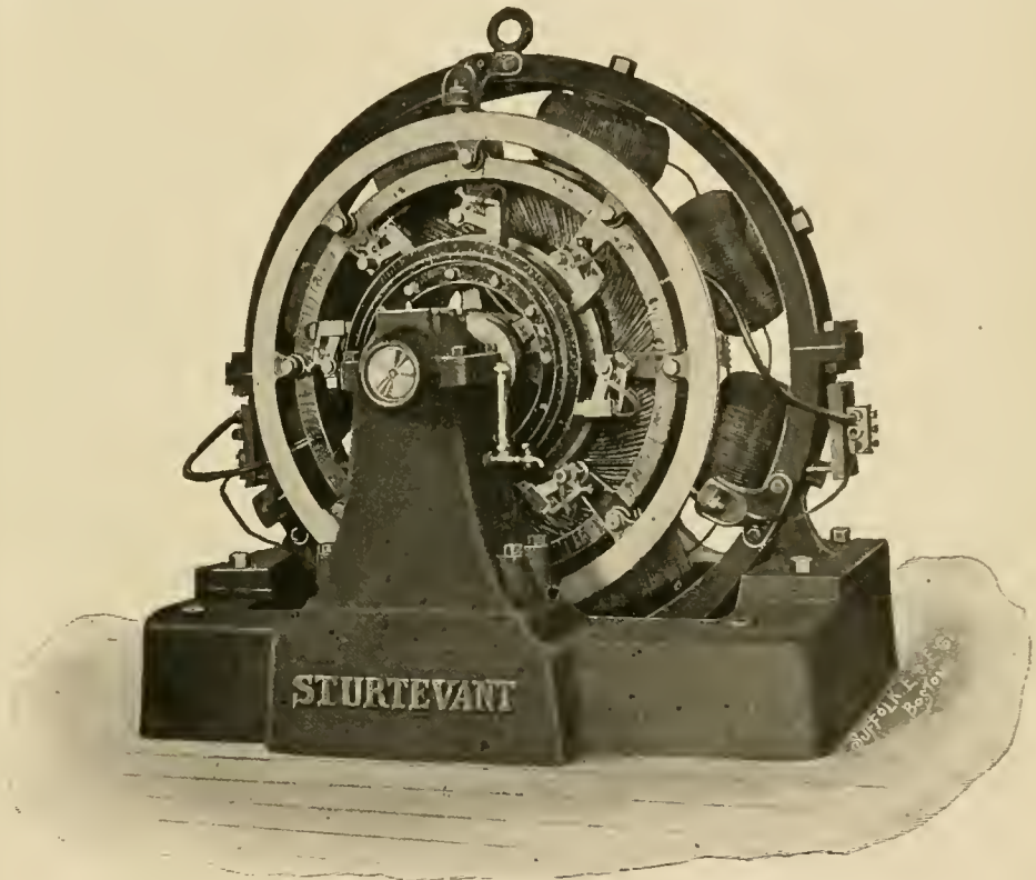
The Sturtevant Eight-Pole Motor and Generator.
