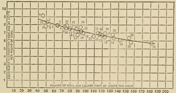
Fig. 6.—Rate of Combustion and Efficiency.
