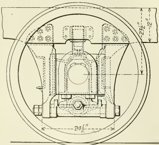
Class "J" Passenger Locomotive—Lake Shore & Michigan Southern Railway.
