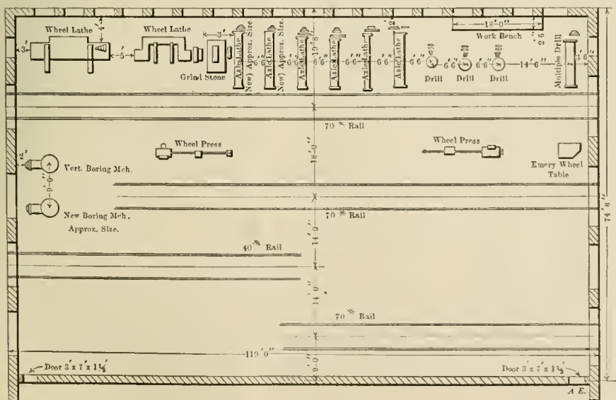
Plan and Side Elevation of New Car Shop.
