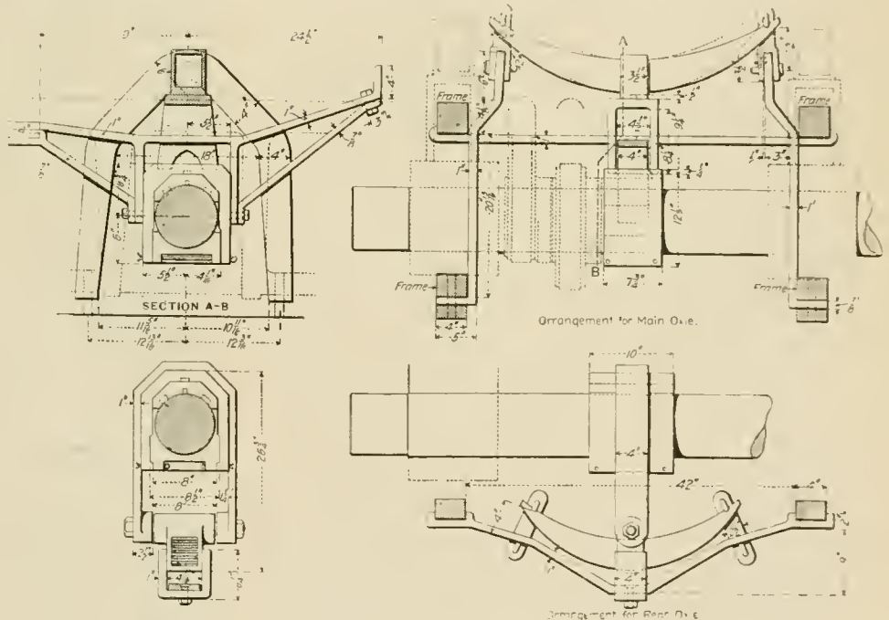
Third Bearing for Driving Wheel Axles—New York, Ontario & Western Railway.
