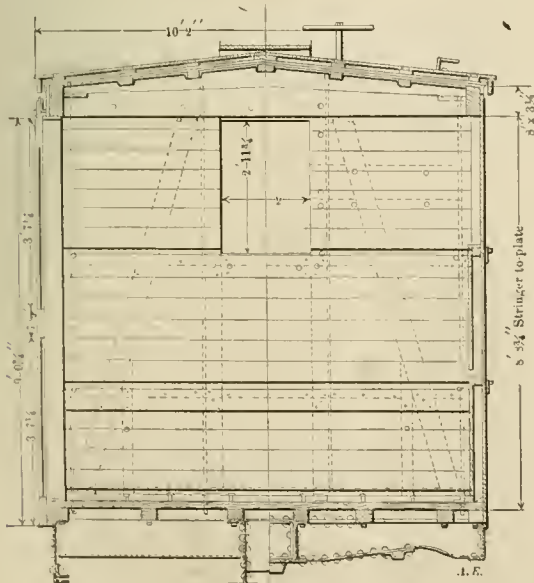
Transverse Section.
