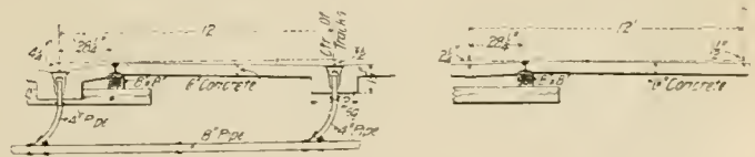
Floor Sections in Paint Shop.
