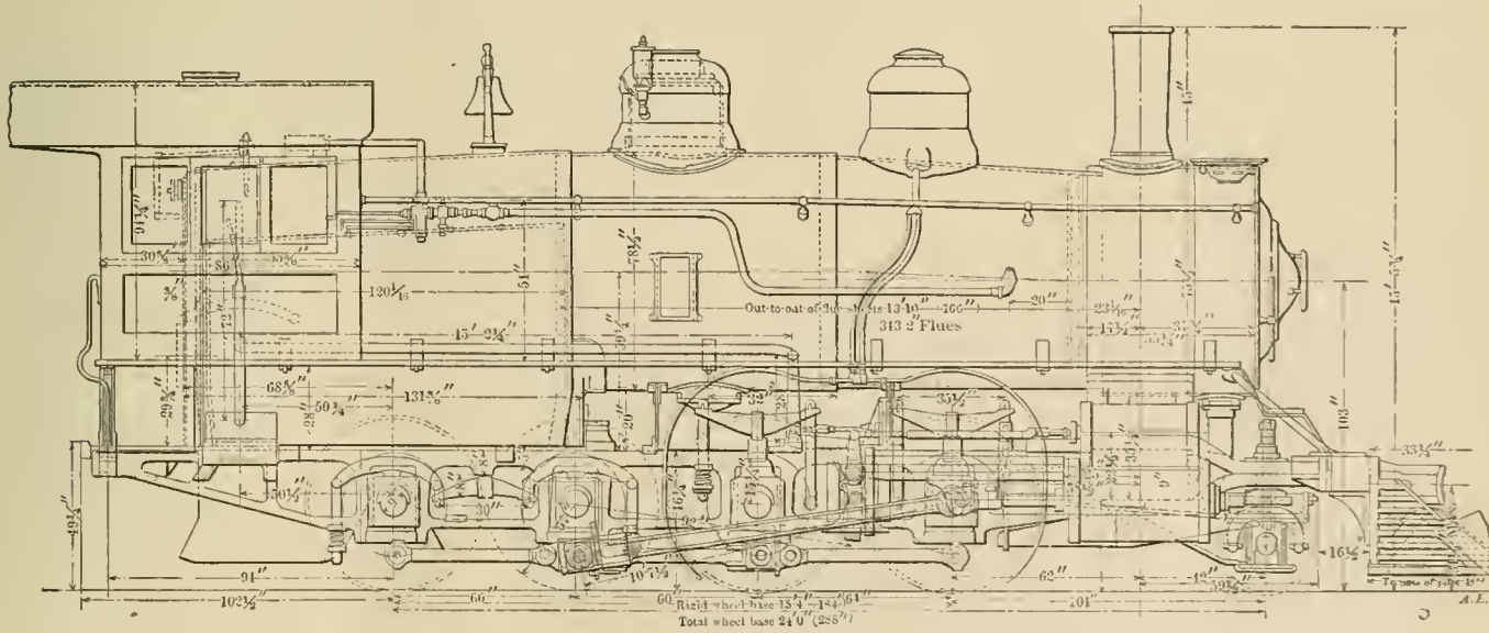
Consolidation Pushing Locomotive—Atchison, Topeka & Santa Fe Railway.
