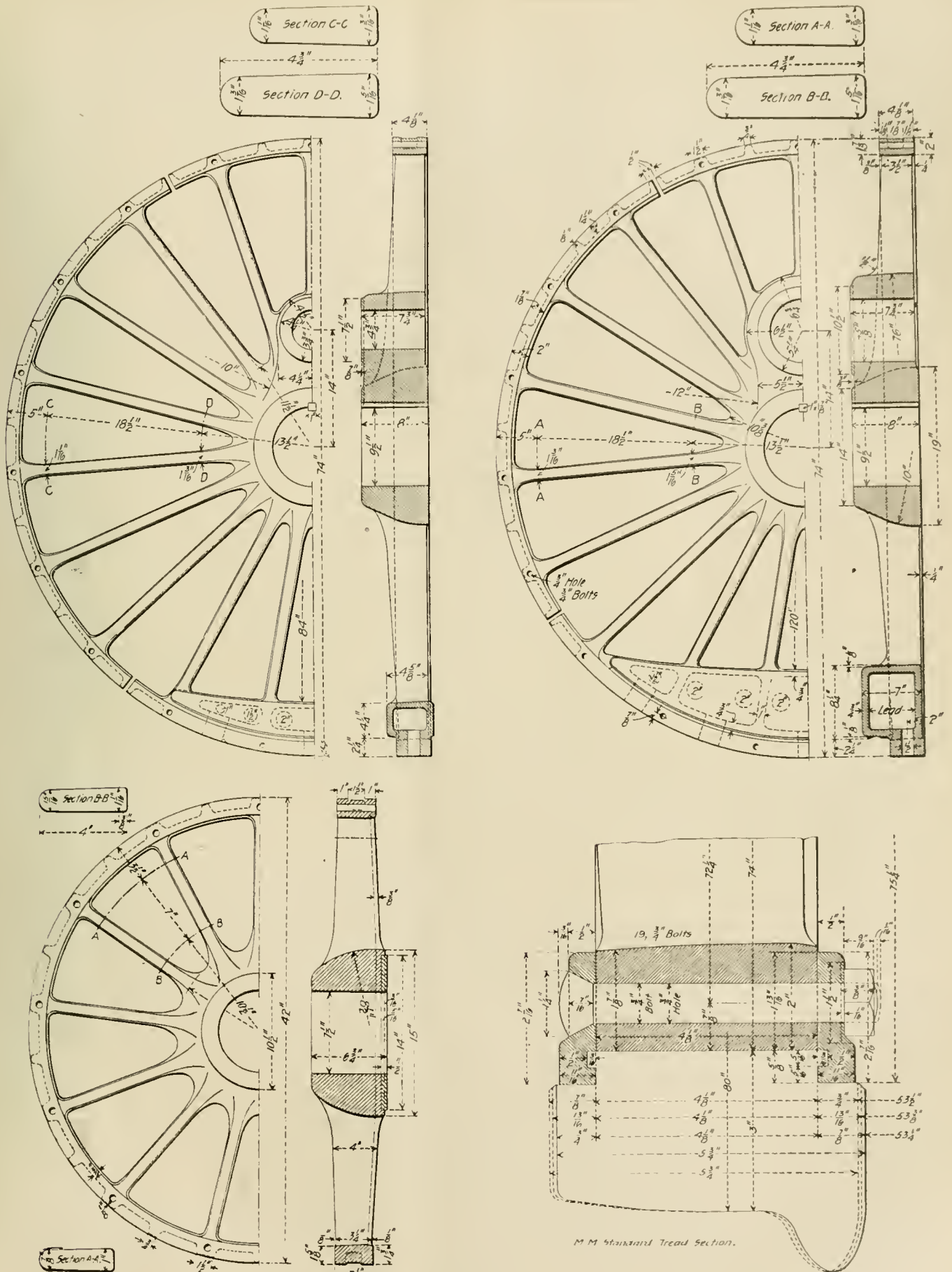
Cast Steel Driving and Truck Wheels.
