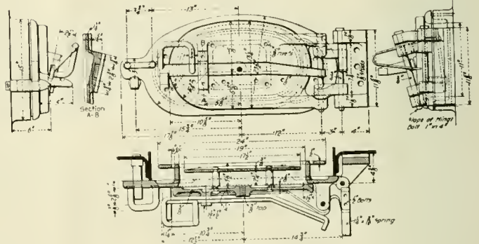
Fire Door.
