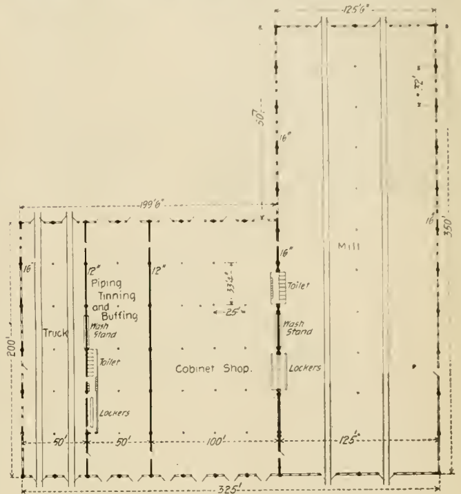
Mill, Cabinet, Pipe and Truck Shops.
