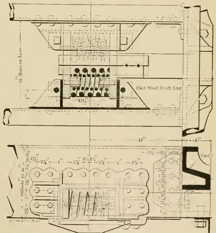
Twin Spring Standard Draft Gear. Draft Gear.
