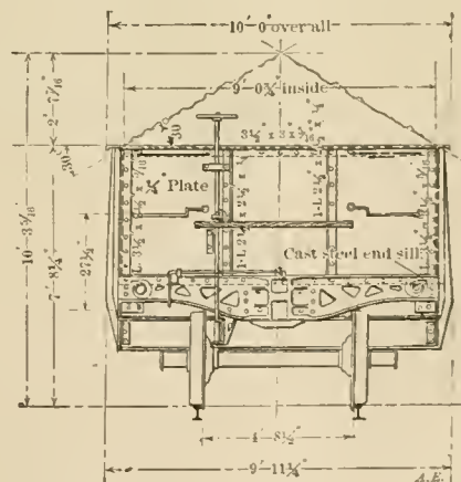
End Elevation.
