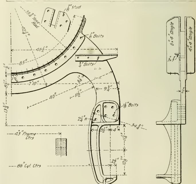
Guide Yoke. Independent of Frames.
