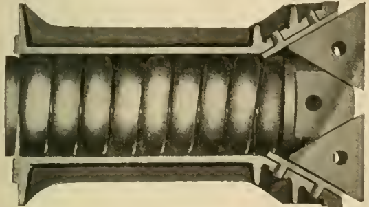
Sectional View, Showing Spring Barrel, and Wedges.
