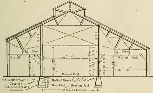
Plan and Section of Boiler Shop.
