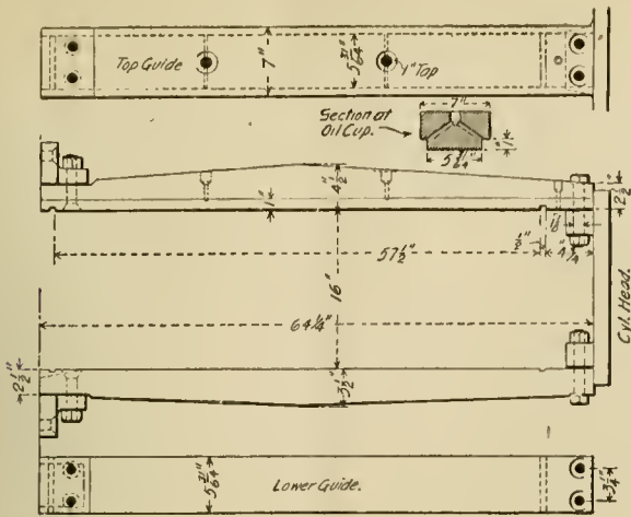
Upper and Lower Guides.
