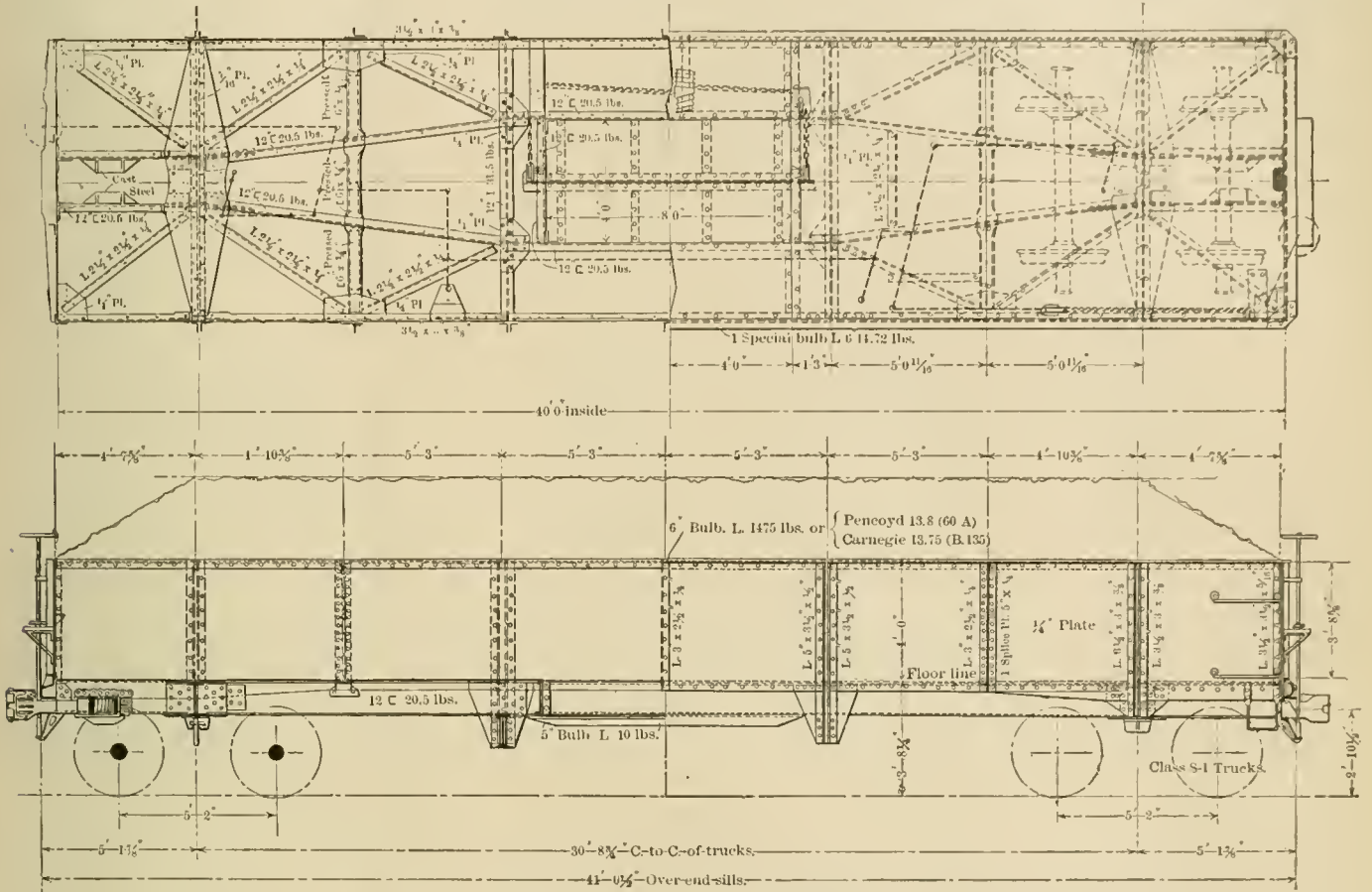
New Fifty-Ton Gondola Coal Car—Elgin, Joliet & Eastern Railroad.
