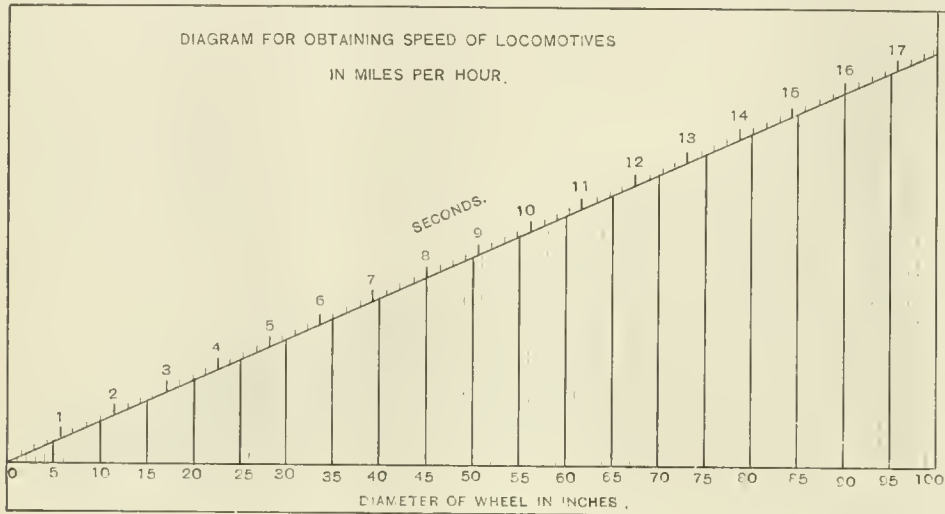
Diagram of Speed of Locomotives.
