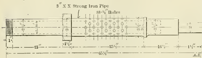
Perforated Pipe Valve Yoke.
