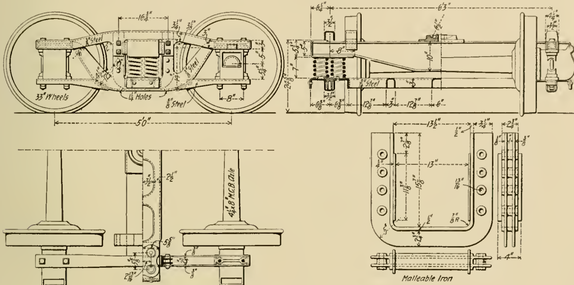
Pressed Steel Truck—Pere Marquette Railroad.
