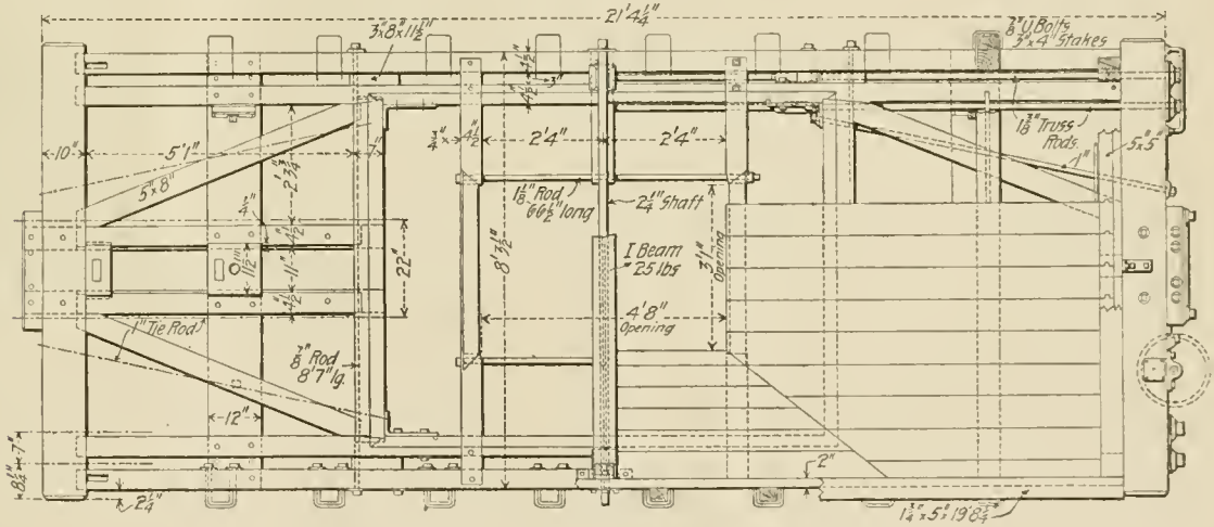
New Ore Cars, Chicago, Milwaukee & St. Paul Railway.
