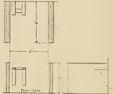
Fig. 2.—Molding Stall.
