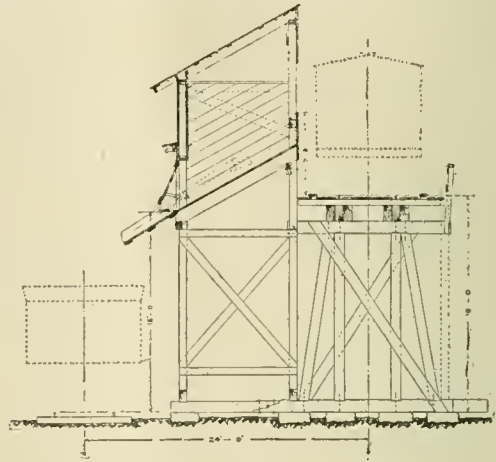
Chicago Great Western Railway Coaling Station.
