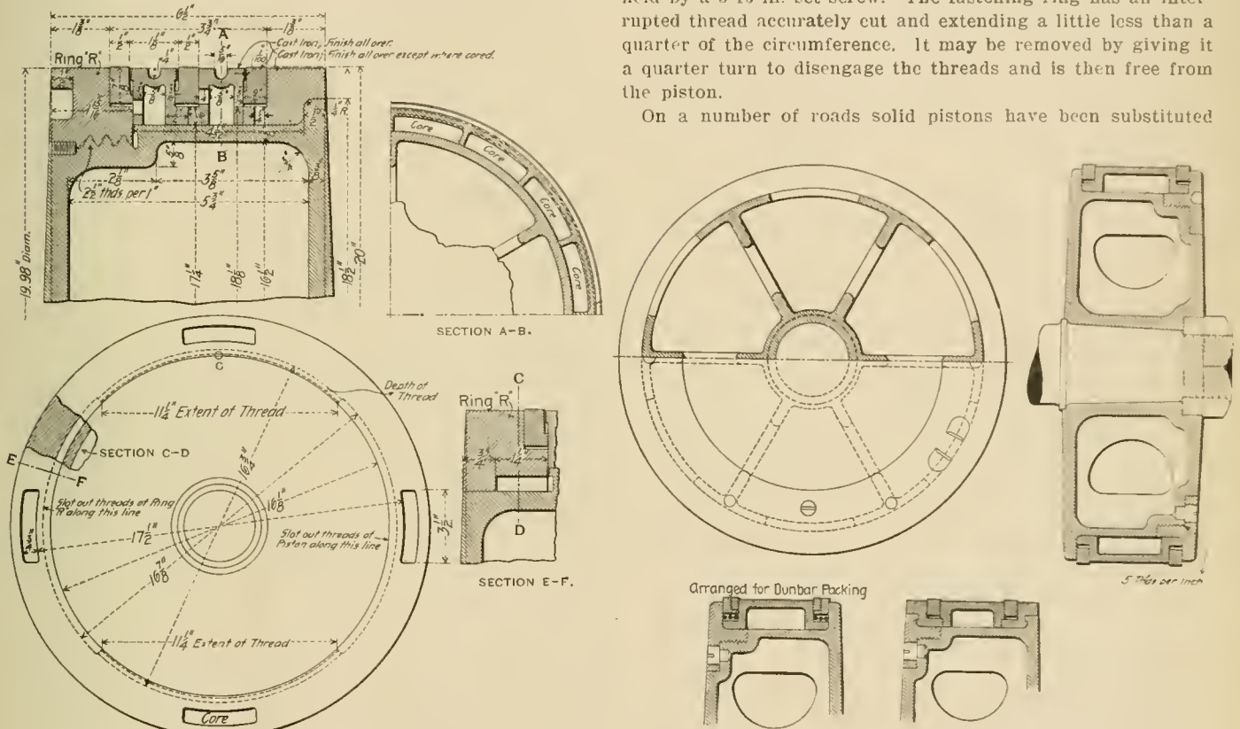
New Method of Constructing Pistons, Showing Preliminary and Completed Designs—Central Railroad of New Jersey.
