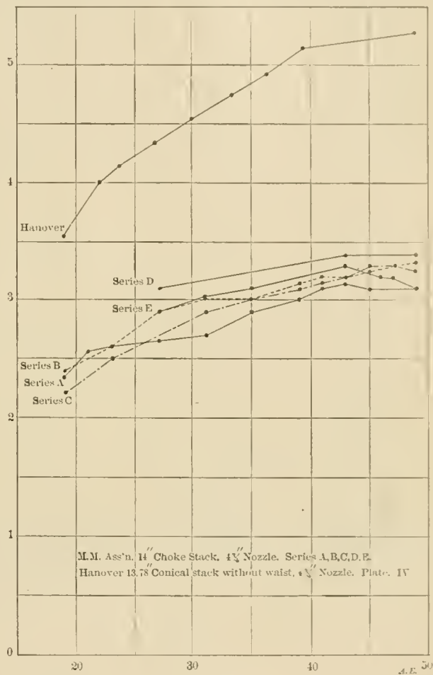
Fig. 5. American Engineer Tests of Locomotive Draft Appliances.
