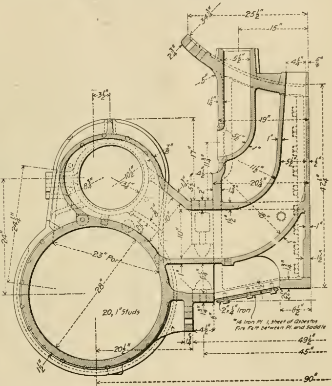
Low Pressure Cylinder.
