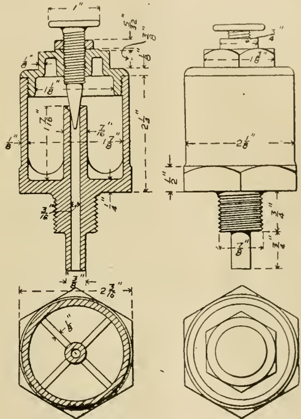
Malleable Iron Oil Cup.
