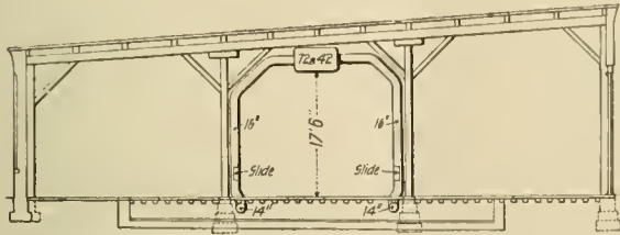
Arrangement of Air Outlets in the Pits. Section at A. B.
