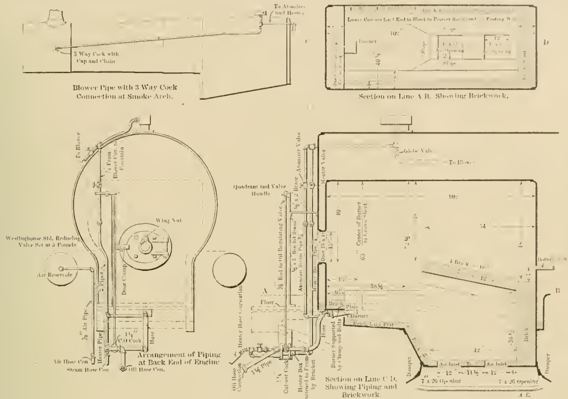
Fig. 1.—Firebox, Brick Work and Piping.
