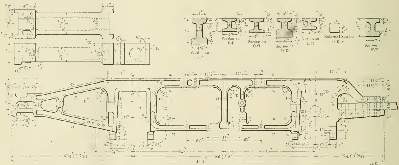
Cast-Steel Locomotive Frames—Delaware & Hudson Company.
