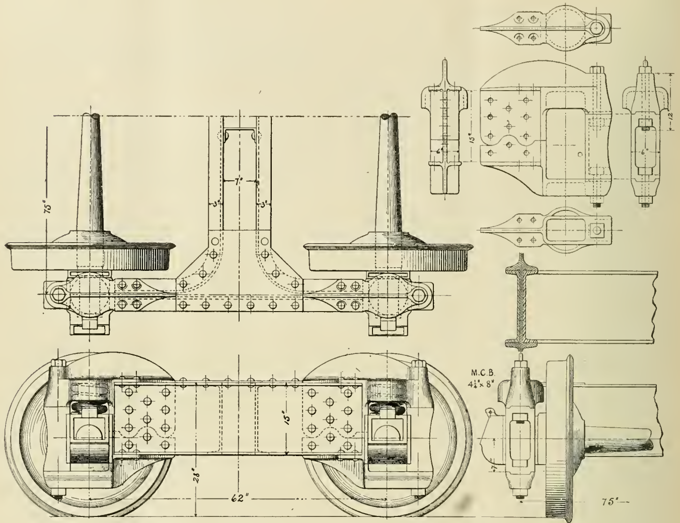
Steel Frame Pedestal Truck.
