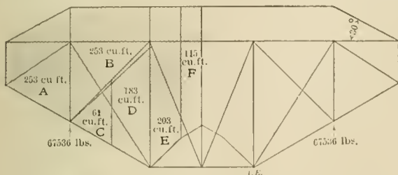
Stress Diagram.
