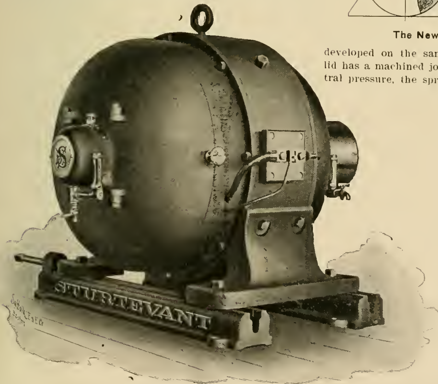
A Four-Pole Enclosed Motor.
