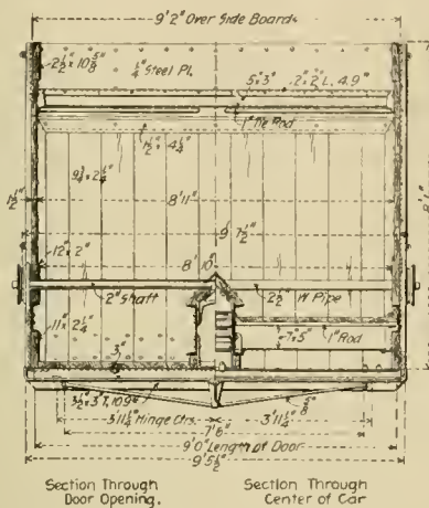
Transverse Section.
