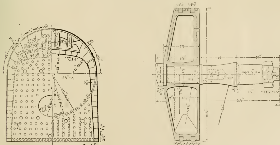
Transverse Section of Firebox.
