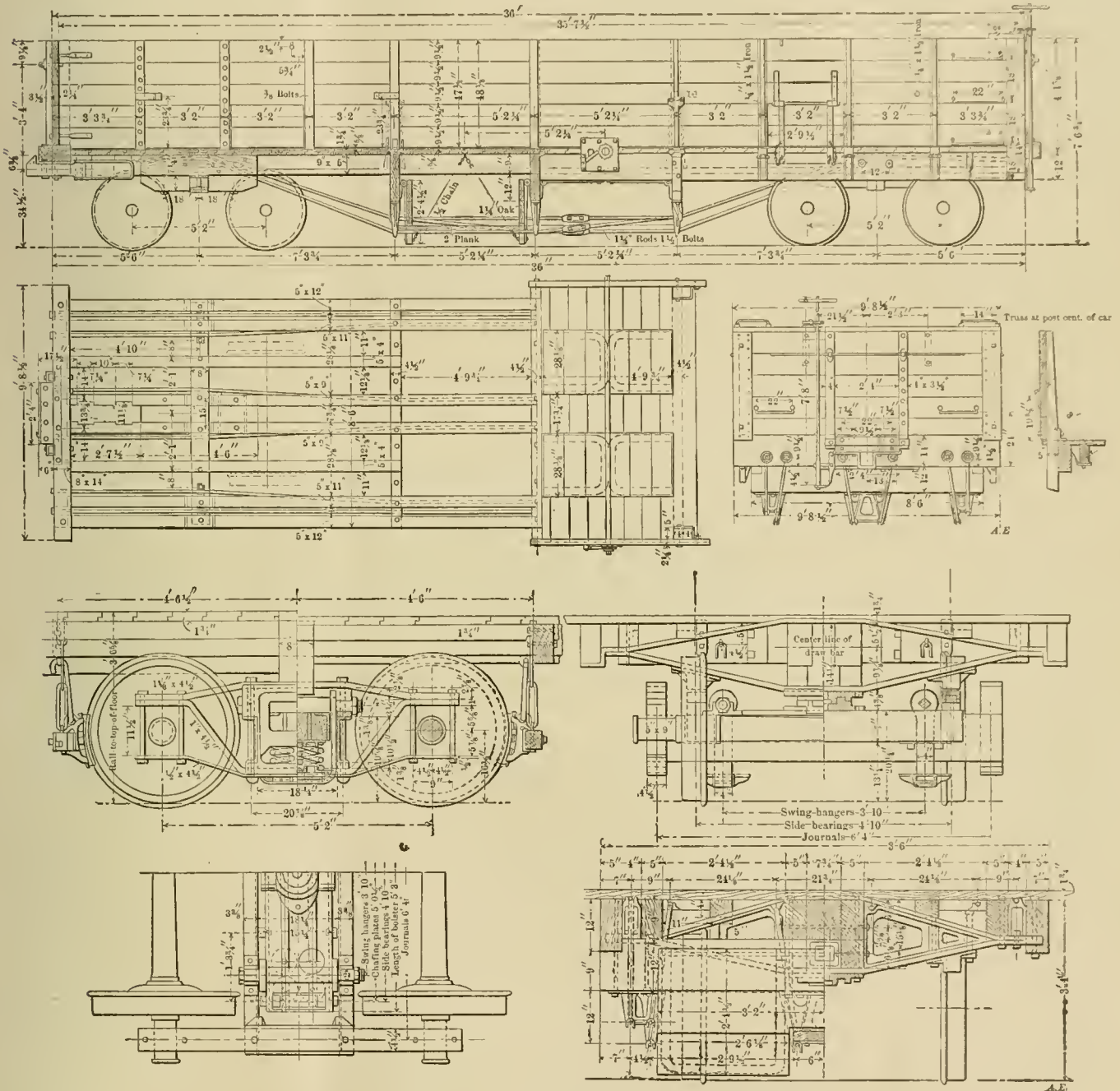
Low Drop-Bottom Gondola Cars, 80,000 Pounds Capacity.
