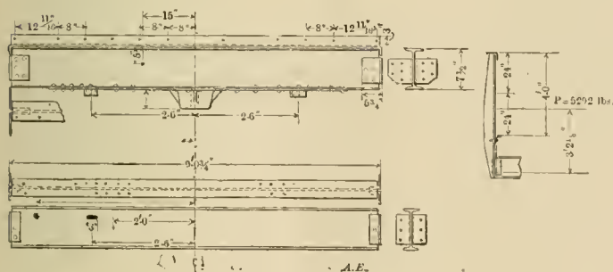
Transoms and Floor Beams.
