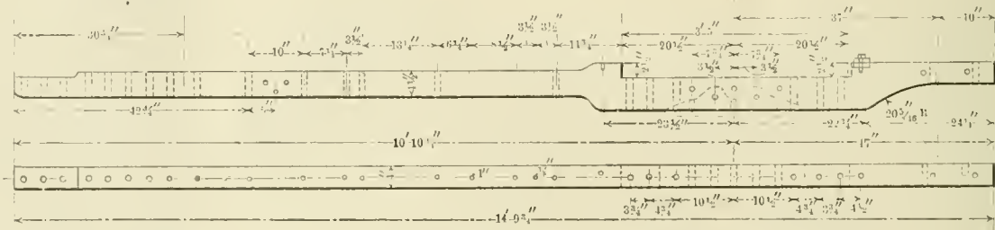
Cast-Steel Equalizer—Delaware Hudson Company.
