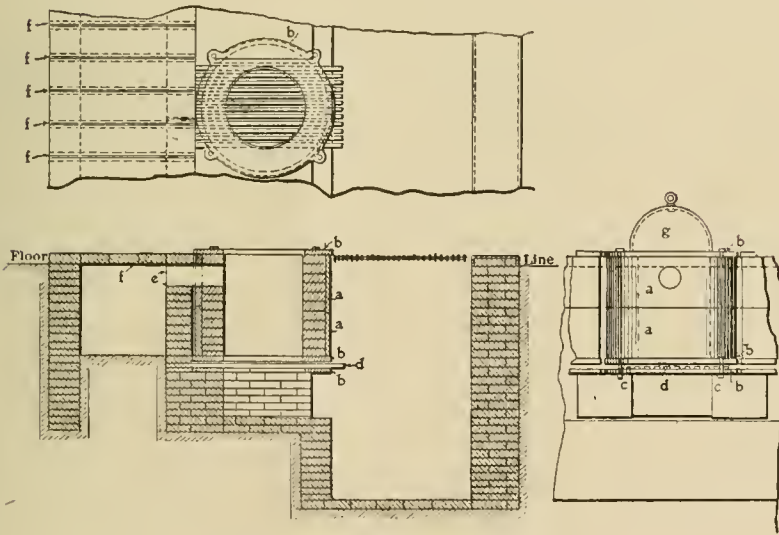
Fig. 3.—Brass Furnace.
