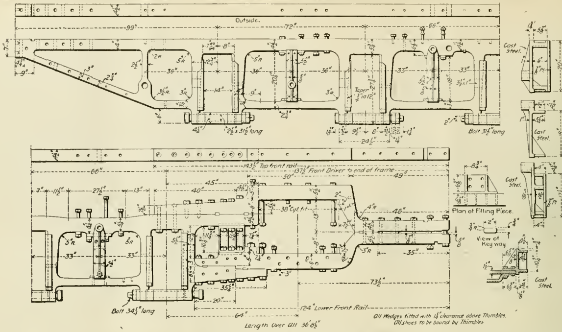
Views of Cast Steel Frames.
