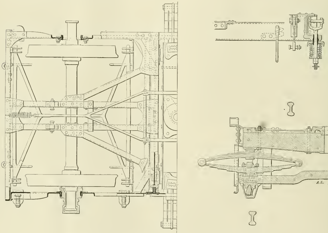
Steel Frame Passenger Truck with Leaf Springs Over the Journals.
