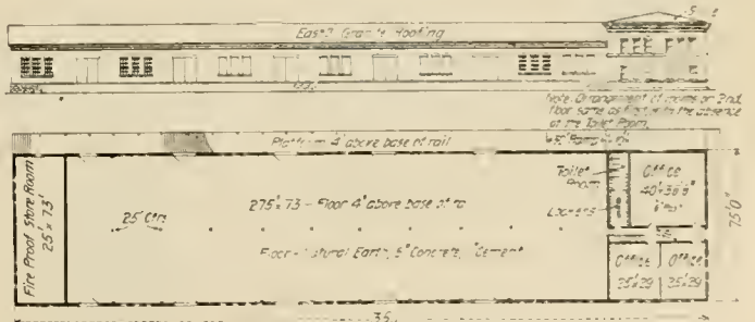
Storehouse and Offices.
