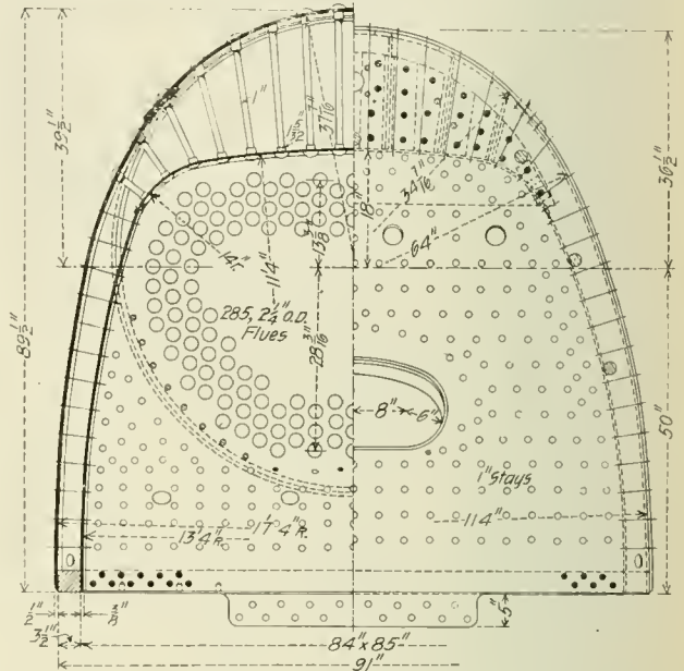
Section and Elevation of Firebox.
