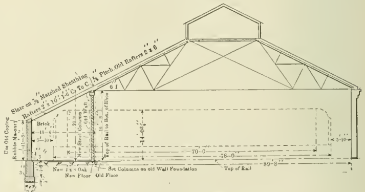
Section of Enlarged Passenger Car Shop.
