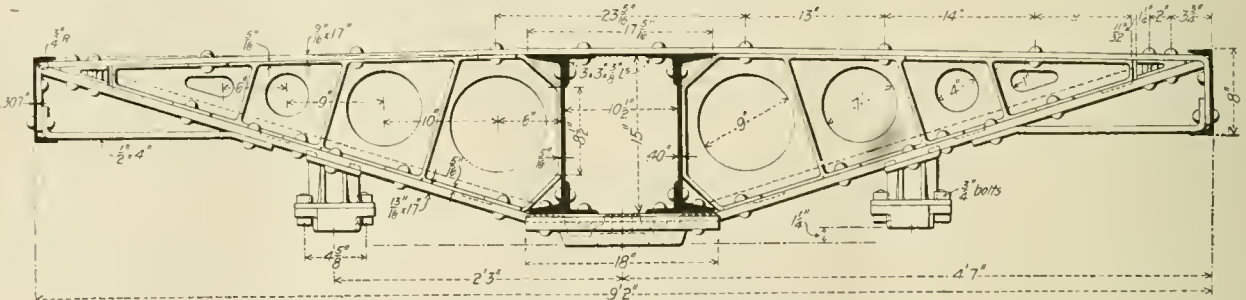
Showing Construction of Body Bolster.
