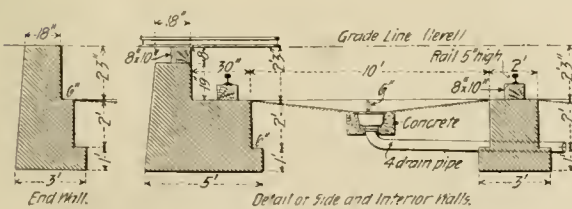
Transfer Table Pit, Drainage and Foundations.
