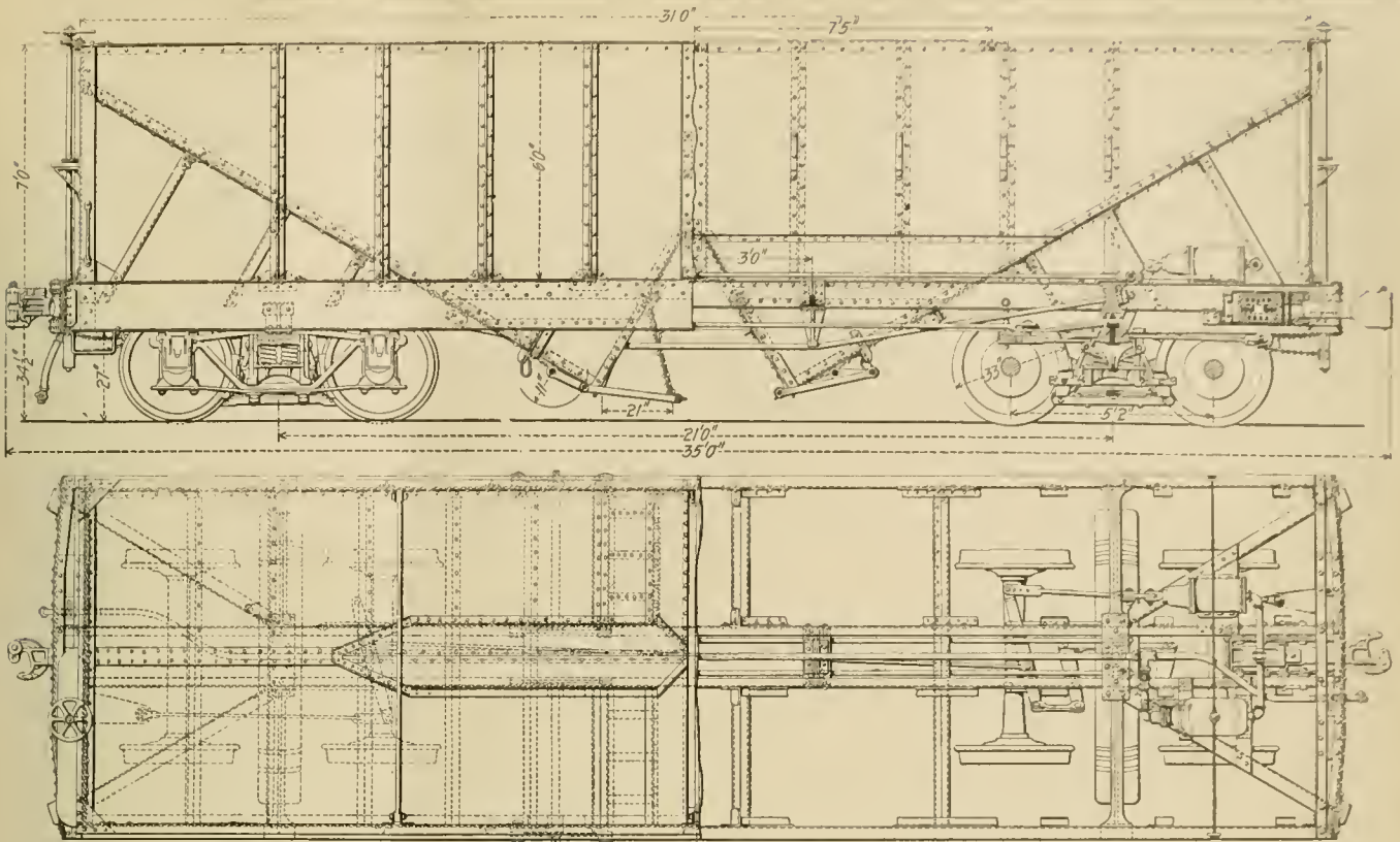
100,000 Pounds Capacity Hopper Cars, with Truss d Center Sills. The Structural Steel Car Company.
