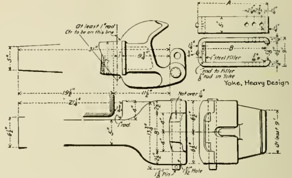
Automatic Coupler 5-in. x 7-in. Shank and Increased Head.
