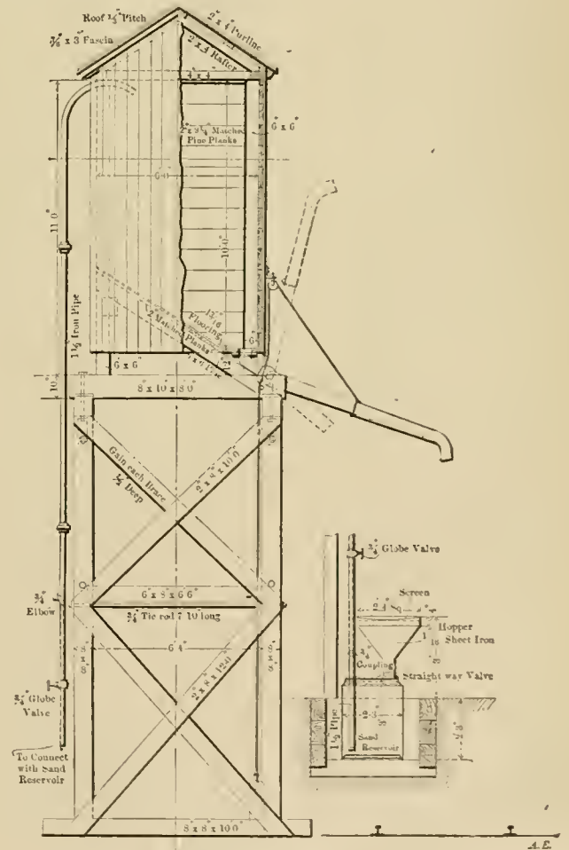
Sand Chute and Elevator.
