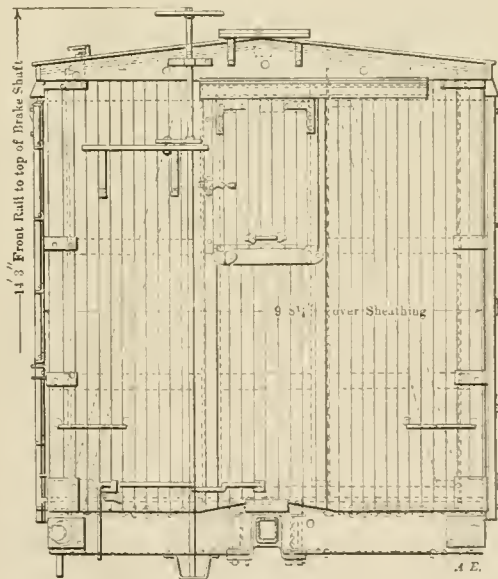
End Elevation.
