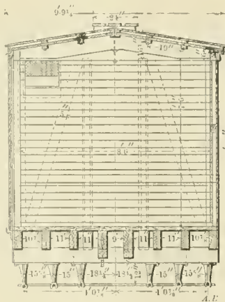
Transverse Section.
