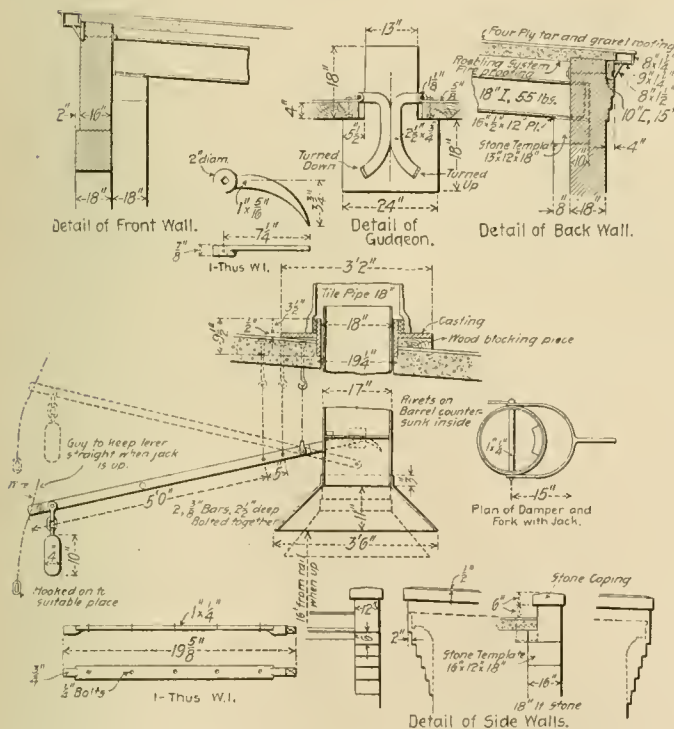
Showing Construction of Fireproof Roundhouse—Canadian Pacific Railway.
