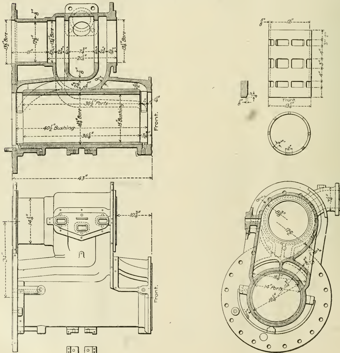
High Pressure Cylinder. Four-Cylinder Tandem Compound Locomotive—Northern Pacific Railway.
