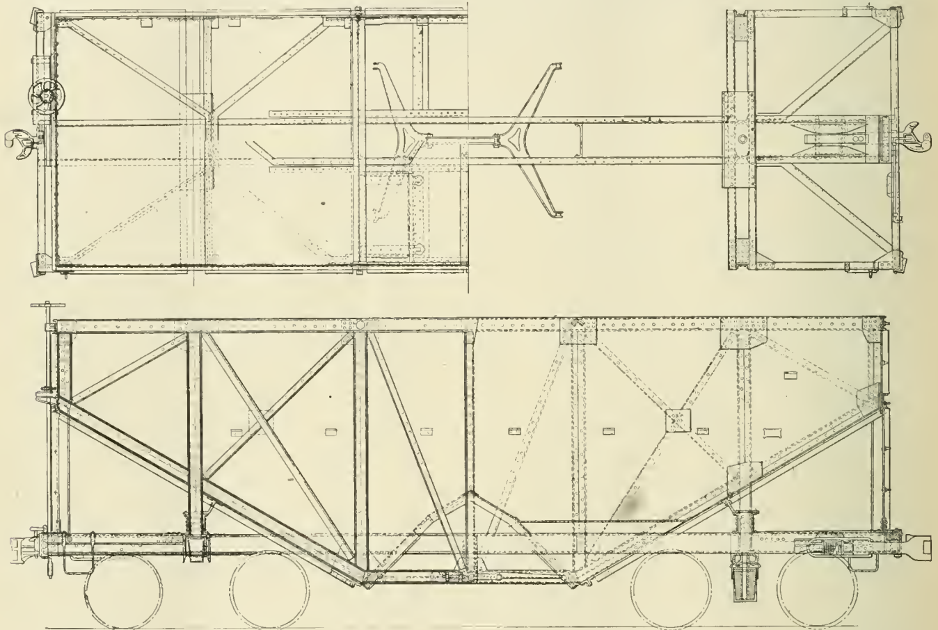
Vanderbilt Steel Hopper Coal Car—Lackawanna Iron & Steel Company.
