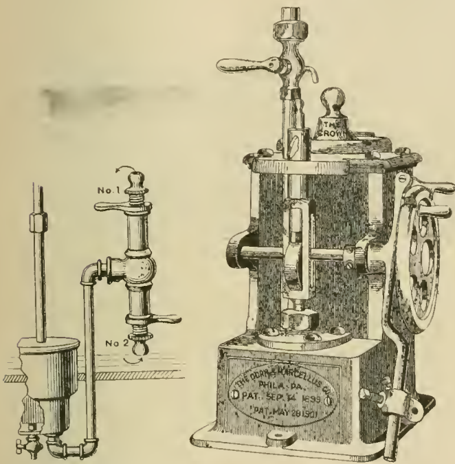
Dash Pot Valve. Automatic Lubricating Pump. Manufactured by Dorn & Marcellus Company.
