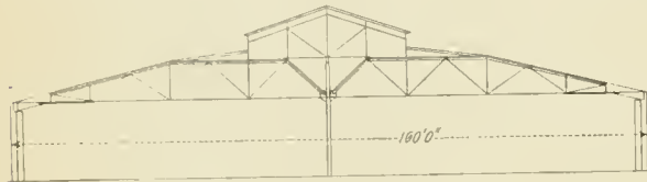
Section Through Car Repair Shop.
