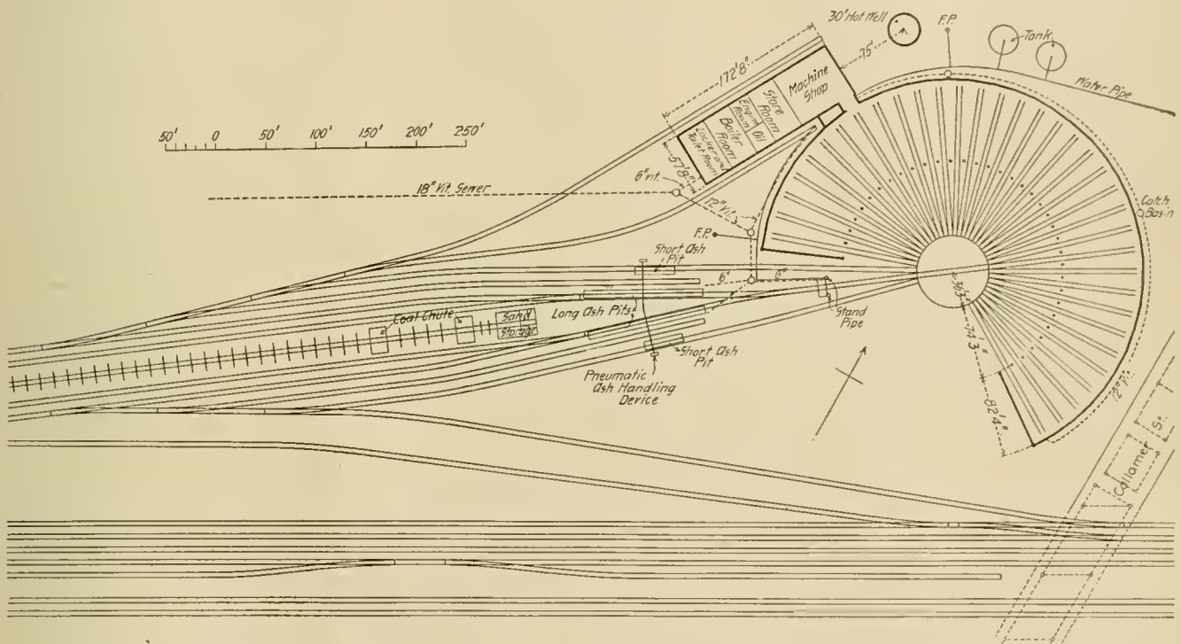
New Round House—Lake Shore & Michigan Southern Railway, at Collinwood, Ohio.
