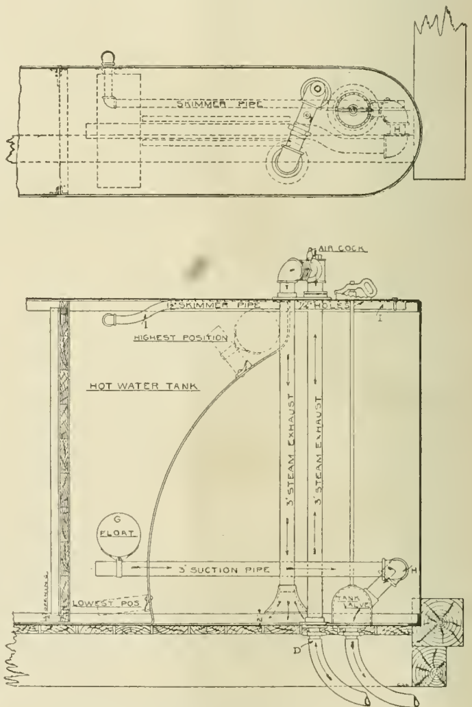
Fig. 2.—Arrangement for Exhaust Steam in Tank.
