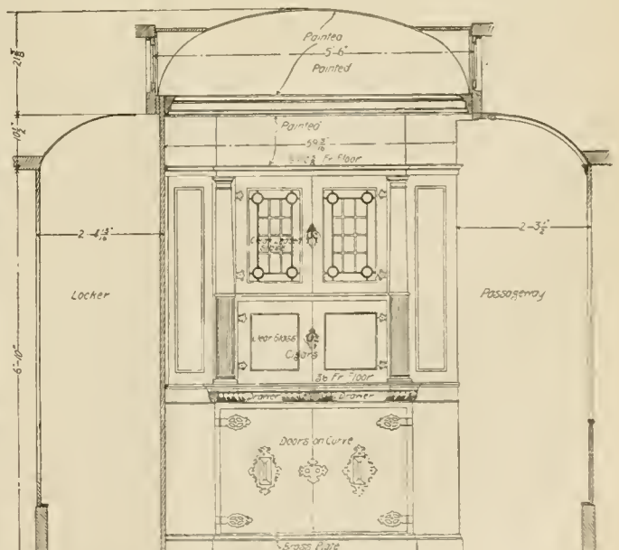
Sideboard Elevation.
