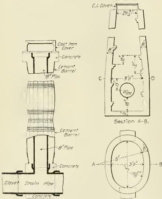
Sections of Man and Lamp Holes.
