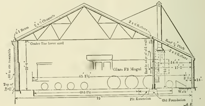
Section Through Roundhouse.
