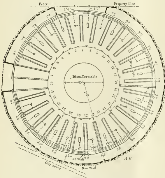
Plan of Enlarged Roundhouse.
