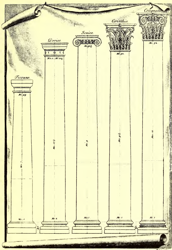
43. THE FIVE ORDERS OF ARCHITECTURE AFTER PALLADIO.
