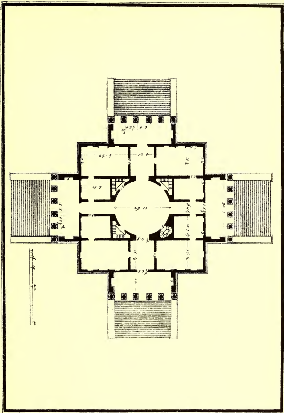
25. THE VILLA CAPRA (THE "ROTONDA"), NEAR VICENZA. PLAN.
