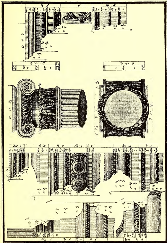
14. MONUMENT TO COUNT LEONARDO PORTO, VICENZA. DETAILS.
