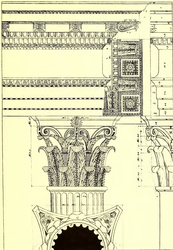
53. THE CORINTHIAN ORDER. DETAIL OF ENTABLATURE AND UPPER PART OF COLUMN.
