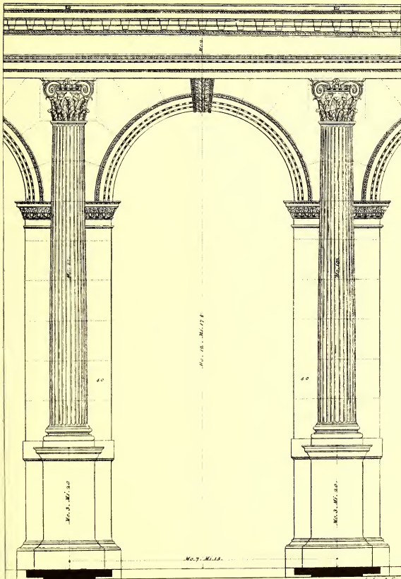
55. THE COMPOSITE ORDER. ARCADE WITH HALF COLUMNS ON PEDESTALS.
