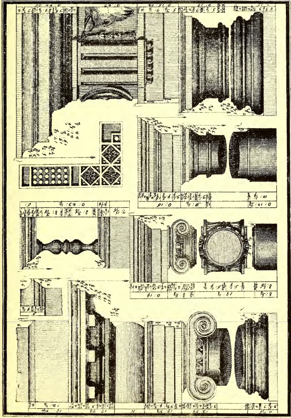
7. THE BASILICA, VICENZA. DETAILS OF DORIC AND IONIC ORDERS TO FACADE.
