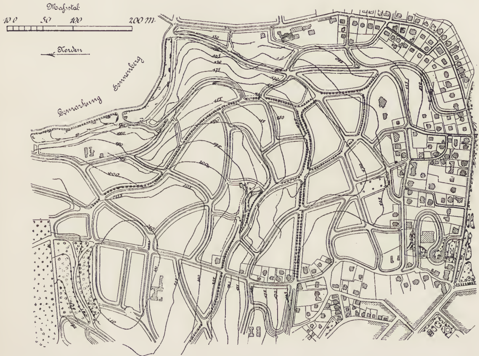
FIG. 29. PLAUEN IN VOIGTLAND: PLANNING FOR A VERY UNDULATING SITE WHERE GRADES EXIST AS HIGH AS 1 IN 4; IN THE NEW MAIN STREET LINES THESE HAVE BEEN MODIFIED TO SOMETHING LIKE 1 TO 10.
