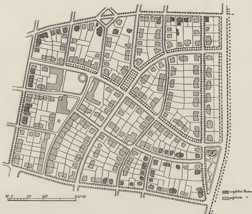
FIG. 28. DARMSTADT: PLANNING OF A CITY QUARTER PARTLY FOR SEPARATE BUILDINGS, PARTLY FOR BUILDINGS IN GROUPS, AND PARTLY IN BLOCKS, AS WELL AS FOR SEVERAL PUBLIC BUILDINGS. NOTE HOW SKILLFULLY THE LATTER HAVE BEEN DISPOSED AND BROUGHT INTO RELATIONS WITH THE OPEN SPACES.
