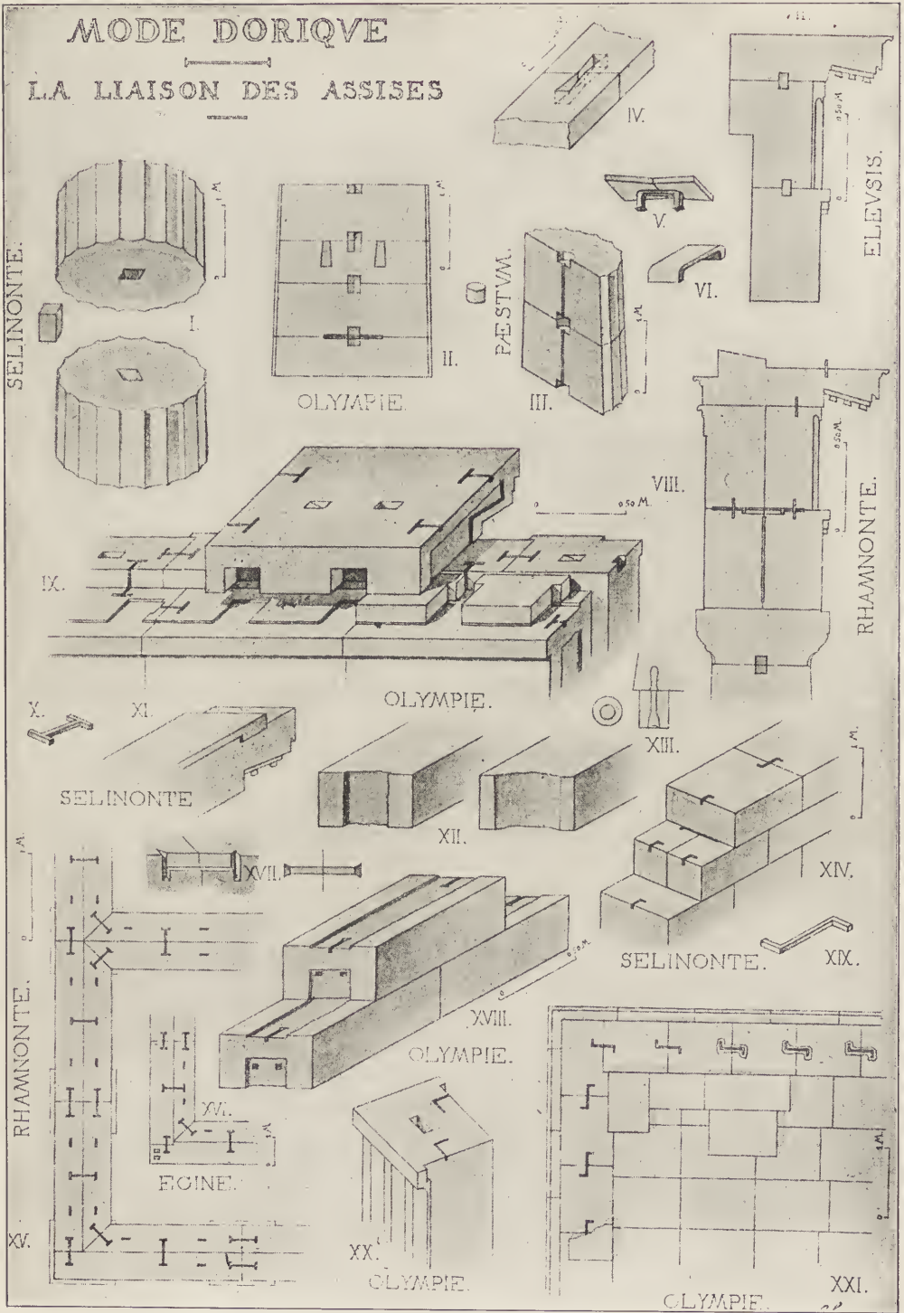
GREEK METHODS OF ATTACHING STONEMASONRY IN THE EARLY OR ARCHAIC AGE (VI-V CENTURIES B. C.).
