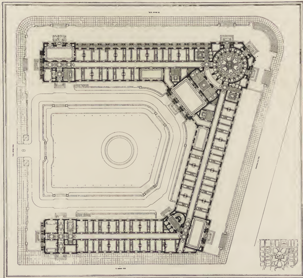
SENATE OFFICE BUILDING—PLAN OF PRINCIPAL (SECOND) FLOOR.
