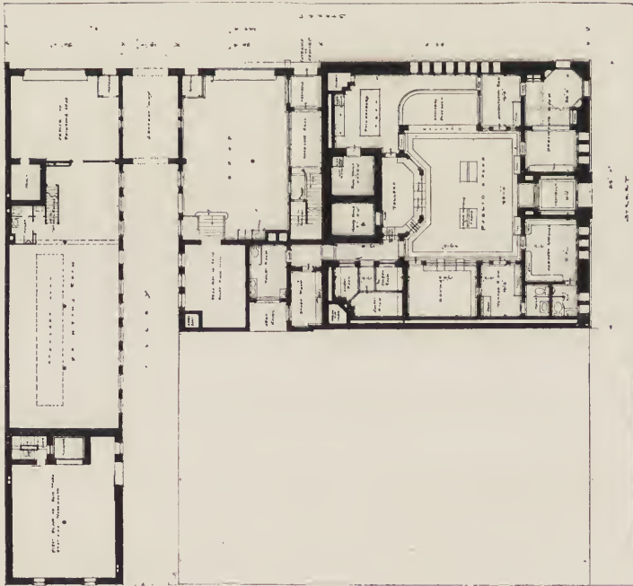
PLAN OF MAIN FLOOR.
