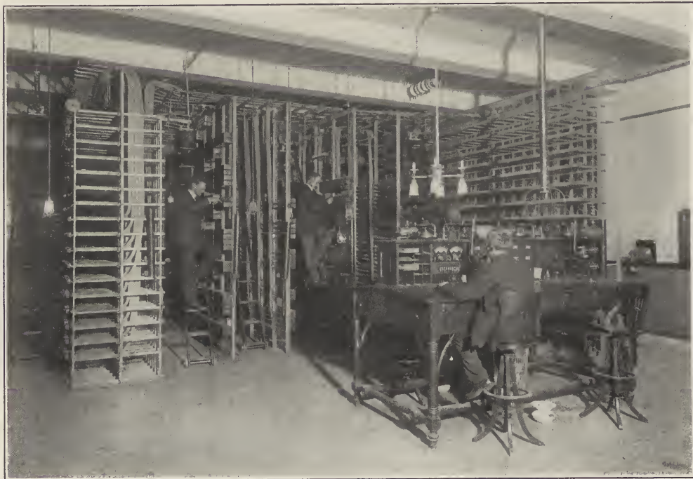
FRAME ROOM AT "EDGEWATER" EXCHANGE, CHICAGO TELEPHONE COMPANY.
