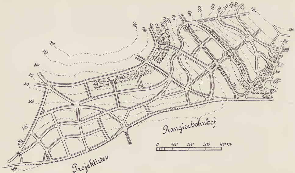
FIG. 27. ULM: PLANNING OF A STEEP SLOPE WITH STREETS OF DIVERSIFIED GRADES.
