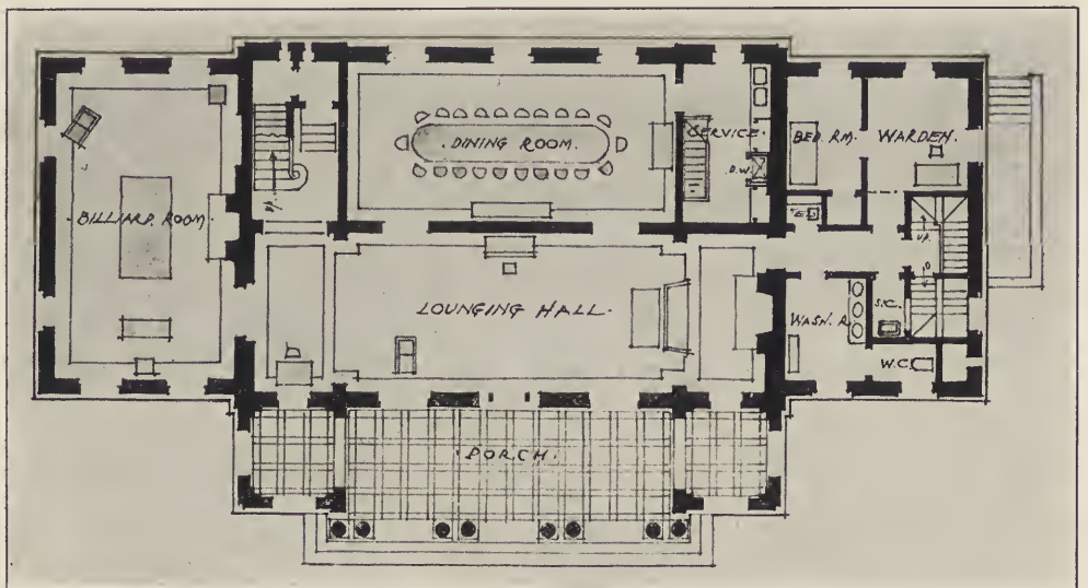
PLAN OF FIRST FLOOR—PHI DELTA THETA FRATERNITY HOUSE, WILLIAMS COLLEGE. Williamstown, Mass. Squires & Wynkoop, Architects.
