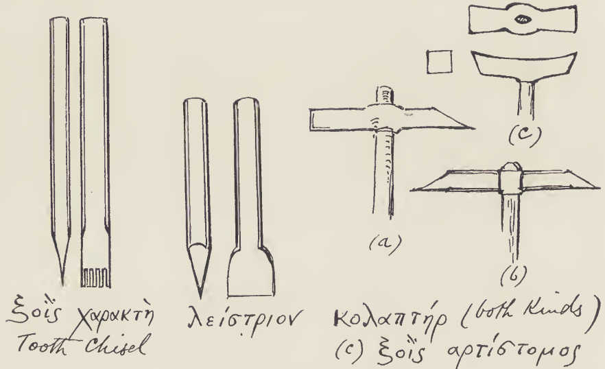
TOOLS OF GREEK STONECUTTERS USED AND MENTIONED IN LEBADEIA SPECIFICATIONS FOR PAVEMENT.
