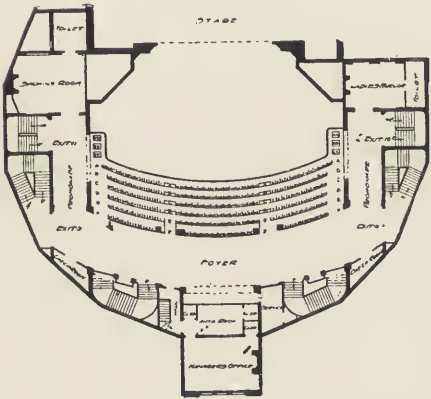
Balcony Plan.
