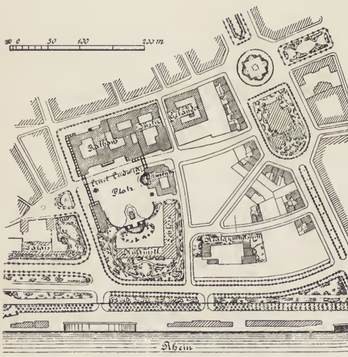
Fig. 22. Mainz: An open space design developed in relation to existing buildings, and on the free site of old fortifications. Note the way in which the structures in the midst of and about the enclosed space have been disposed. (The latter between the Rathaus and the Palace.)
