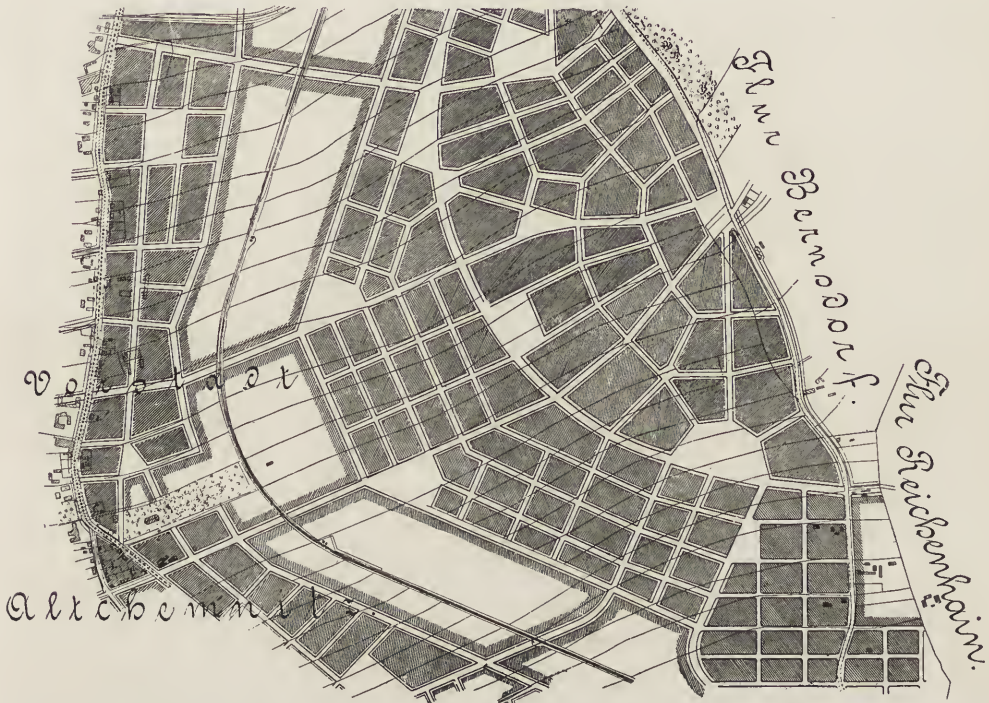
FIG. 17—CHEMNITZ—THE PLANNING OF A CITY QUARTER IN THE OPEN COUNTRY.
