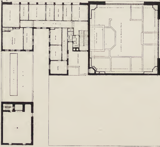
PLAN OF UPPER FLOOR.
