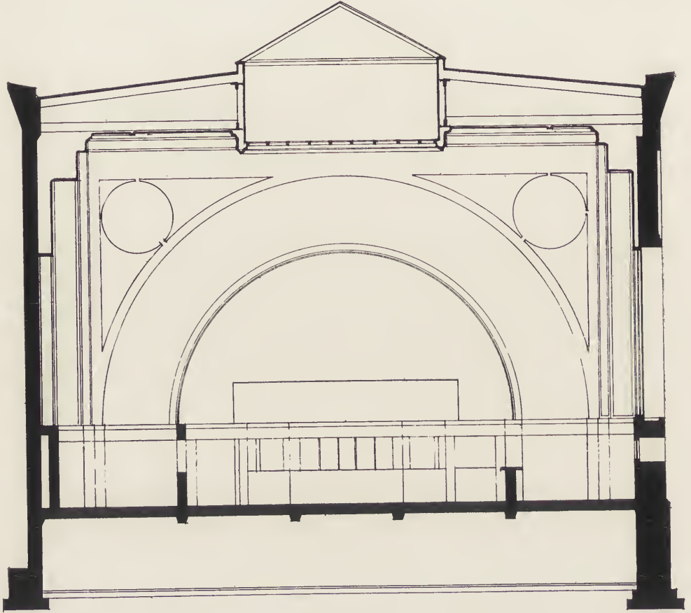
NATIONAL FARMERS' BANK OF OWATONNA, MINN.—CROSS-SECTION THROUGH BANKING ROOM.
