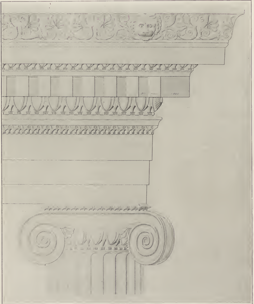
PRIENE, TEMPLE OF ATHENA; ORDER, UNIQUE DESIGN WITHOUT FRIEZE BY PYTHIUS (TIME ALEXANDER THE GREAT).
