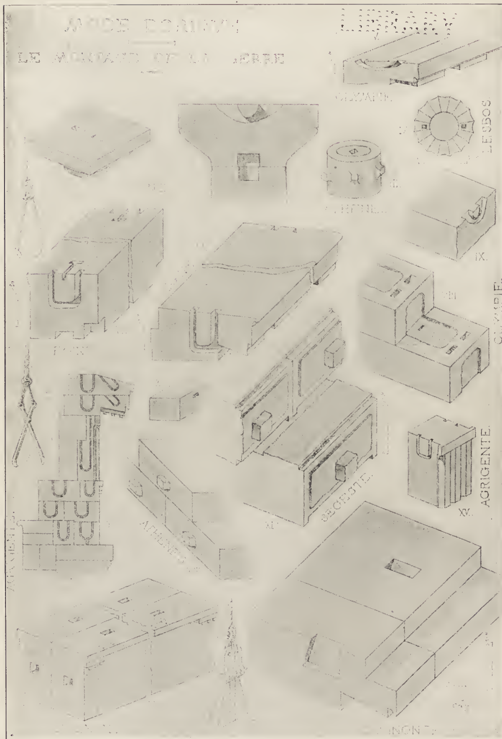
GREEK METHODS OF PREPARING, RAISING AND PLACING STONWORK IN THE EARLY ARCHAIC AGE (VI-V CENTURIES B. C.). (From Perrot: Hist. Anc., Art. VII.)
