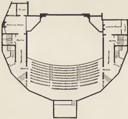
Gallery Plan.
