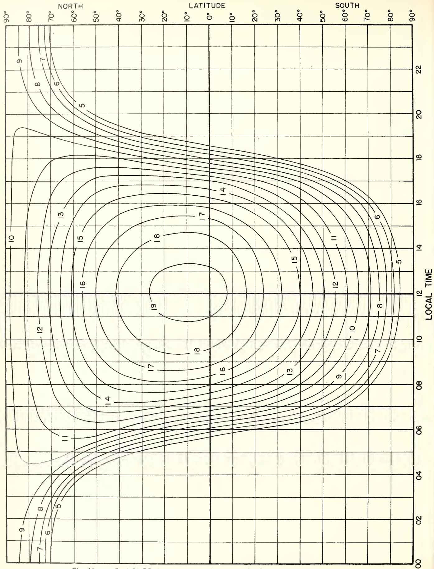
Fig. II. E-LAYER 2000-MUF, IN Mc, PREDICTED FOR AUGUST, 1946.
