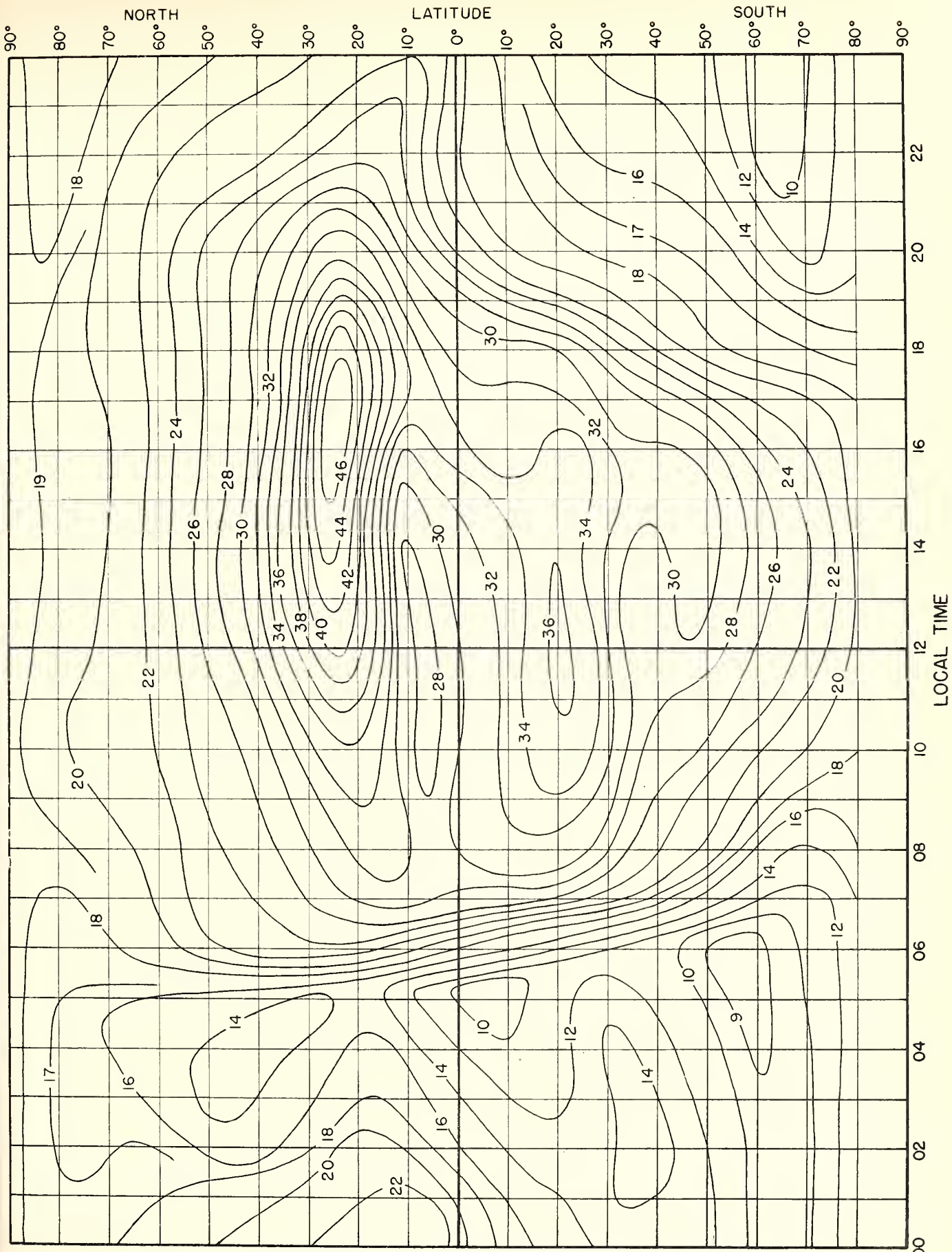
Fig. 10. F_2 4000-MUF, IN Mc, E ZONE, PREDICTED FOR AUGUST, 1946.
