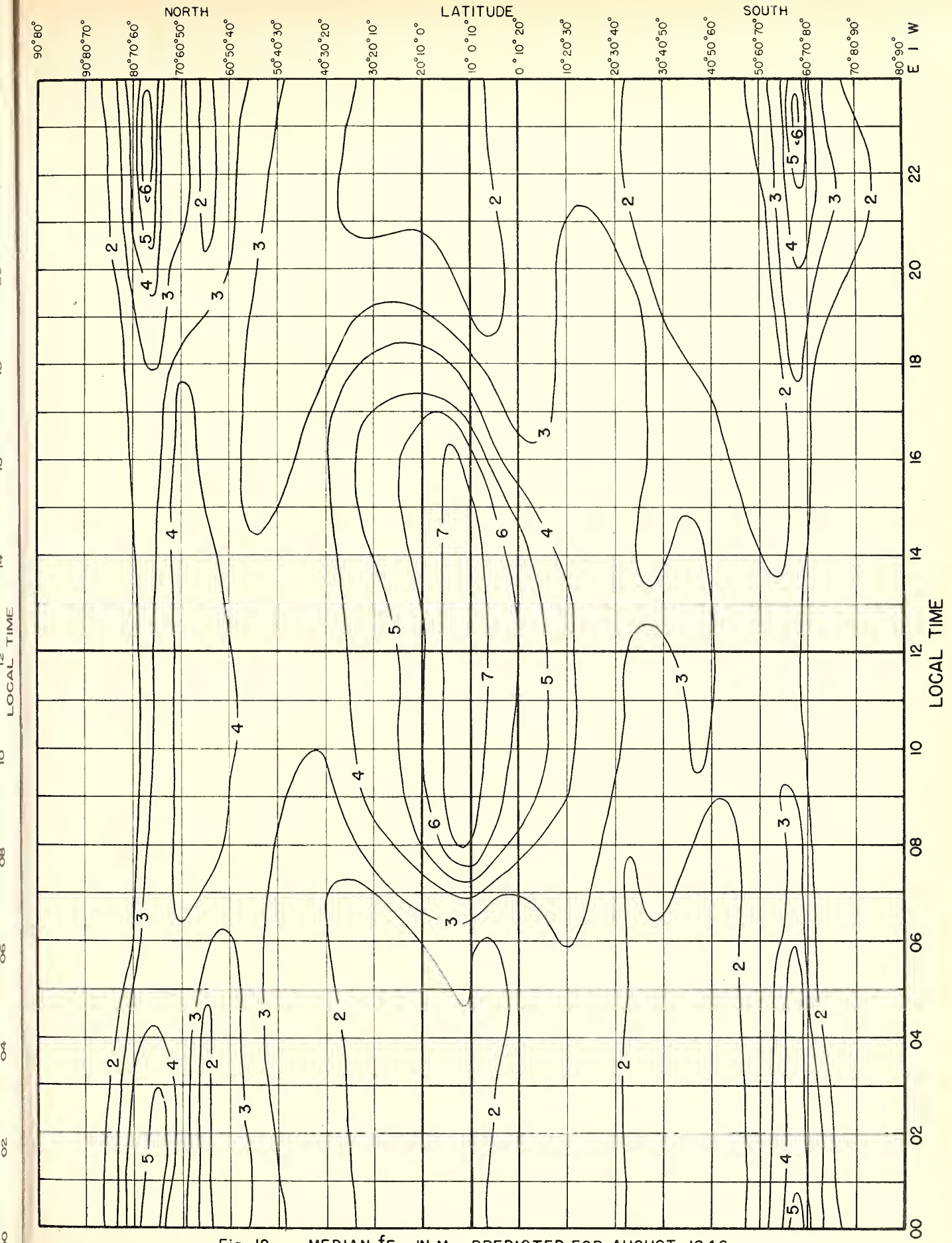
Fig. 12. MEDIAN fE_s , IN Mc, PREDICTED FOR AUGUST, 1946.
