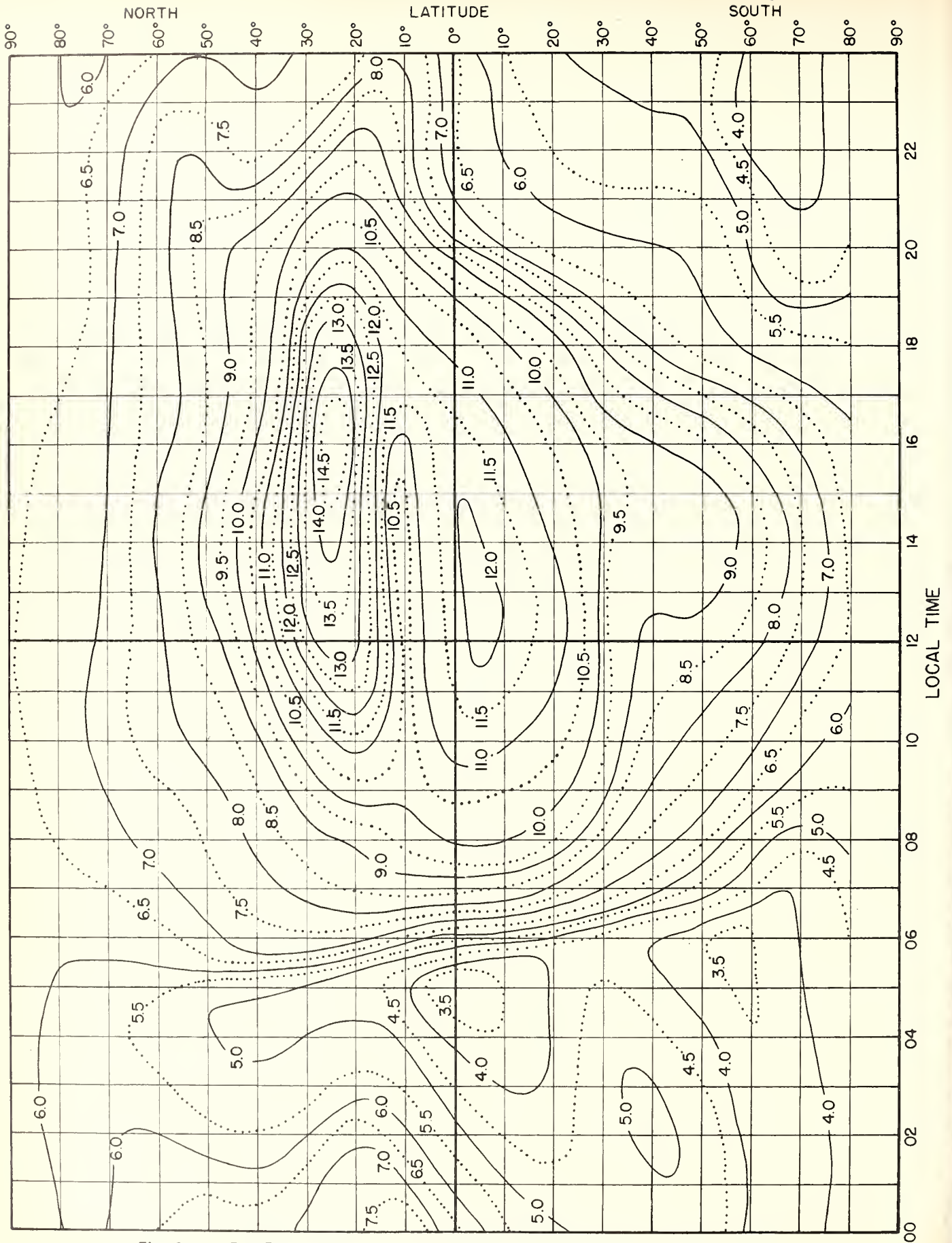
Fig. 9. F_2 ZERO-MUF, IN Mc, E ZONE, PREDICTED FOR, AUGUST, 1946.
