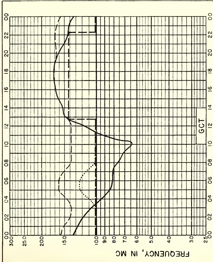
Fig. 16. SAMPLE SOLUTION OF TRANSMISSION PROBLEM FOR SHORT PATH, AUGUST, 1946.
