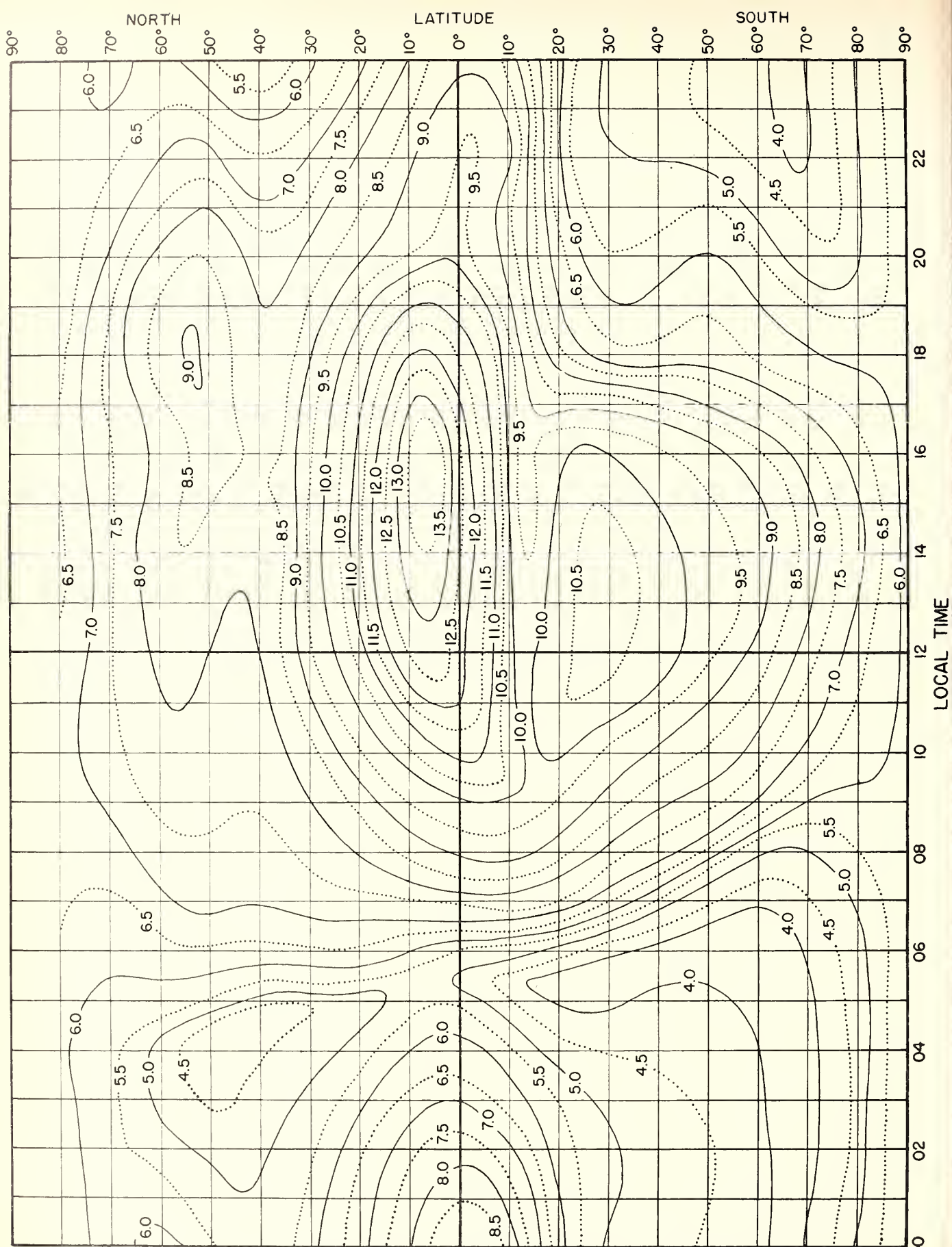
Fig. 5. F_2 ZERO-MUF, IN Mc, W ZONE, PREDICTED FOR AUGUST, 1946.
