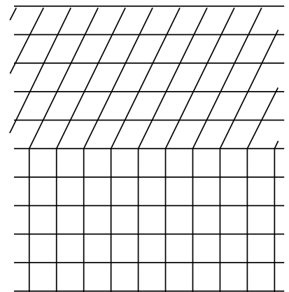
f / "Bob, your manifold isn't smooth!"
