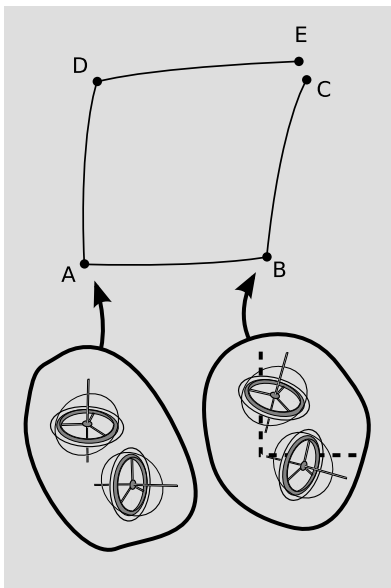
b / The gyroscopes both rotate when transported from A to B, causing Helen to navigate along BC, which does not form a right angle with AB. The angle between the two gyroscopes' axes is always the same, so the rotation is not locally observable, but it does produce an observable gap between C and E.
