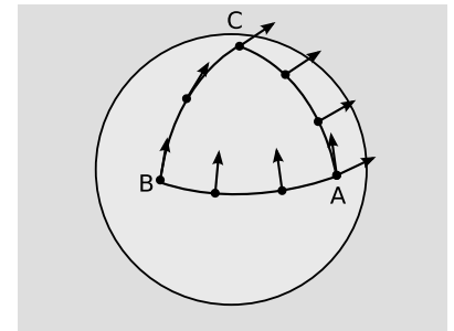
b / The change in the vector due to parallel transport around the octant equals the integral of the Riemann tensor over the interior.
