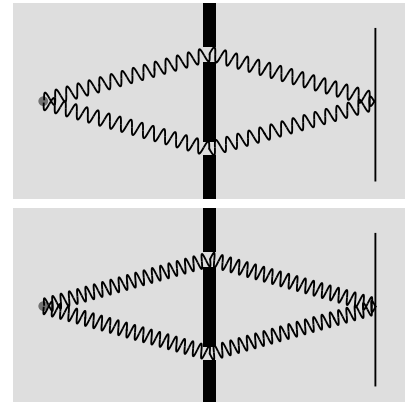
a / A double-slit experiment with electrons. If we add an arbitrary constant to the potential, no observable changes result. The wavelength is shortened, but the relative phase of the two parts of the waves stays the same.
