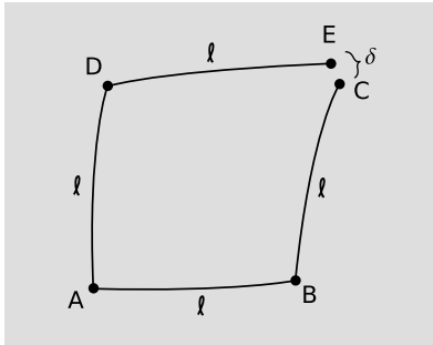
a / Measuring \partial^2 T / \partial x \partial y for a scalar T .
