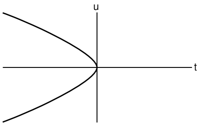
a / The change of coordinates is degenerate at t = 0 .
