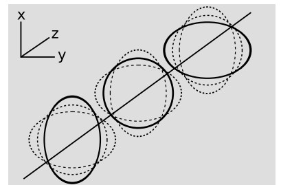
f / As the gravitational wave propagates in the z direction, the metric oscillates in the x and y directions, preserving volume.
