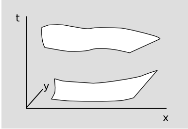
a / Two spacelike surfaces.
