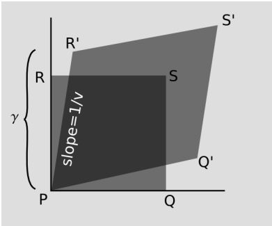
c / Unit square PQRS is Lorentz-boosted to the parallelogram P'Q'R'S'.
