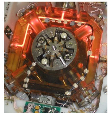
c / A ring laser gyroscope built for use in inertial guidance of aircraft.
