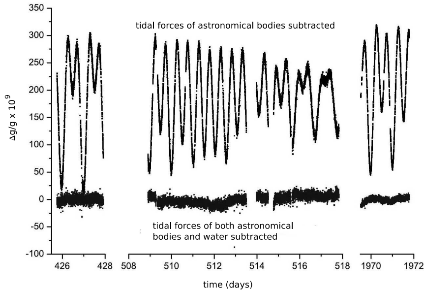
d / The results of the measurement of g by Chung et al., section 2.4.3. The experiment was done on the Stanford University campus, surrounded by the Pacific ocean and San Francisco Bay, so it was subject to varying gravitational from both astronomical bodies and the rising and falling ocean tides. Once both of these effects are subtracted out of the data, there is no Lorentz-violating variation in g due to the earth's motion through space. Note that the data are broken up into three periods, with gaps of three months and four years separating them. (c) APS, used under the U.S. fair use exception to copyright.
