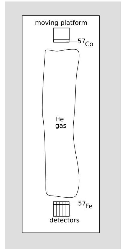
p / The Pound-Rebka experiment.
