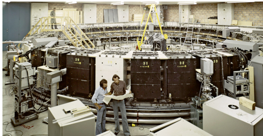
f / Apparatus used for the test of relativistic time dilation described in example 12. The prominent black and white blocks are large magnets surrounding a circular pipe with a vacuum inside. (c) 1974 by CERN.
