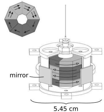
d / The University of Washington torsion pendulum used to search for torsion. The light gray wedges are Alnico, the darker ones \text{SmCo}_5 . The arrows with the filled heads represent the directions of the electron spins, with denser arrows indicating higher polarization. The arrows with the open heads show the direction of the \mathbf{B} field.
