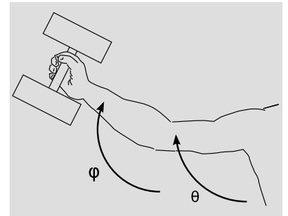
j/ There is no natural metric on the space (\theta, \phi) .
