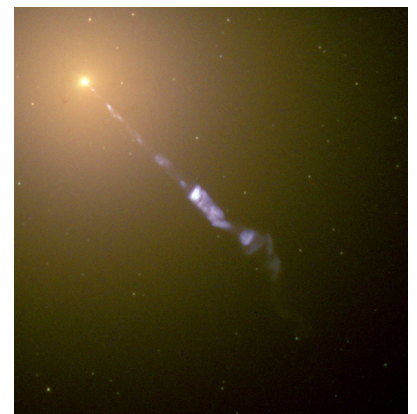
d / A relativistic jet.
