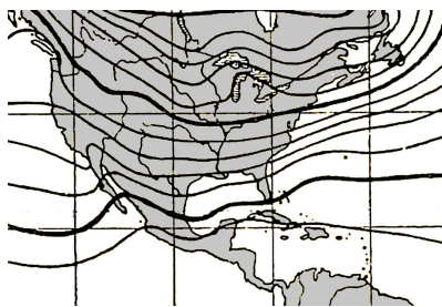
i / Constant-temperature curves for January in North America, at intervals of 4^\circ\text{C} . The temperature gradient at a given point is a dual vector.
