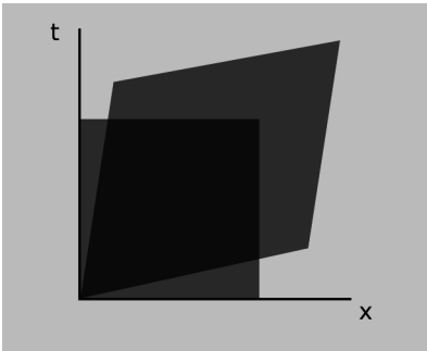
a / Two objects at rest have world-lines that define a rectangle. In a second frame of reference in motion relative to the first one, the rectangle becomes a parallelogram.
