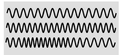
b / Two wavefunctions with constant wavelengths, and a third with a varying wavelength. None of these are physically distinguishable, provided that the same variation in wavelength is applied to all electrons in the universe at any given point in spacetime. There is not even any unambiguous way to pick out the third one as the one with a varying wavelength. We could choose a different gauge in which the third wave was the only one with a constant wavelength.
