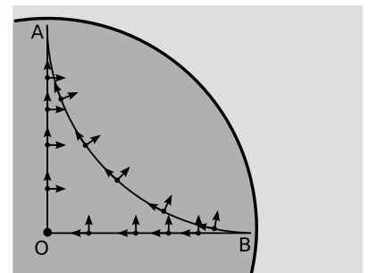
i / In the limit where A and B are ultrarelativistic velocities, leg AB is perpendicular to the edge of the velocity disk. The result is that the x - y frame determined by the ship's gyroscopes has rotated by 90 degrees by the time it gets home.
