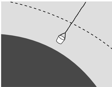
d / Example 14. Matter is lifted out of a Newtonian black hole with a bucket. The dashed line represents the point at which the escape velocity equals the speed of light.
