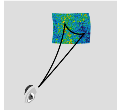
f / The angular scale of fluctuations in the cosmic microwave background can be used to infer the curvature of the universe.
