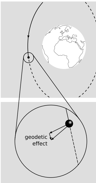
a / The geodetic effect as measured by Gravity Probe B.
