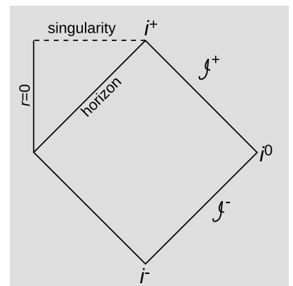
b / Penrose diagram for Schwarzschild spacetime: a black hole that didn't form by gravitational collapse.
