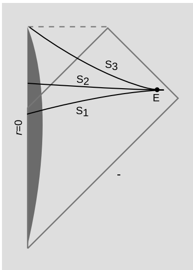
d / According to the distant observer, does the infalling matter ever reach the singularity?
