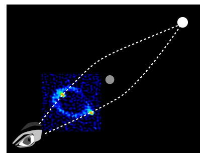
b / An Einstein’s ring is formed when there is a chance alignment of a distant source with a closer gravitating body. Here, a quasar, MG1131+0456, is seen as a ring due to focusing of light by an unknown object, possibly a supermassive black hole. Because the entire arrangement lacks perfect axial symmetry, the ring is nonuniform; most of its brightness is concentrated in two lumps on opposite sides. This type of gravitational lensing is direct evidence for the curvature of space predicted by gravitational lensing. The two geodesics form a lune, which is a figure that cannot exist in Euclidean geometry.
