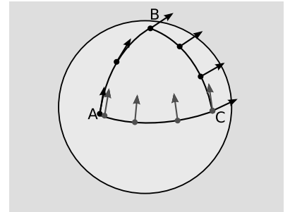
b / Parallel transport is path-dependent. On the surface of this sphere, parallel-transporting a vector along ABC gives a different answer than transporting it along AC.
