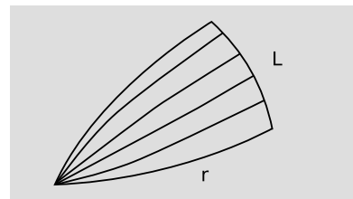
i / 2. Gaussian curvature as L \neq r\theta .
