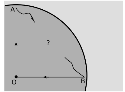
h / A round-trip involving ultrarelativistic velocities. All three legs are at constant acceleration.
