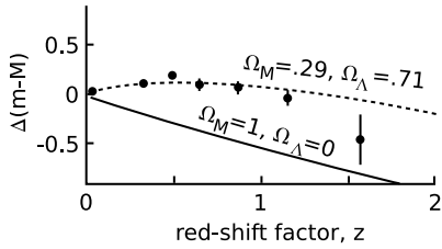
g / A Hubble plot for distant supernovae. Each data point represents an average over several different supernovae with nearly the same z .
