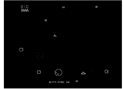
a / In Asteroids, space "wraps around."
