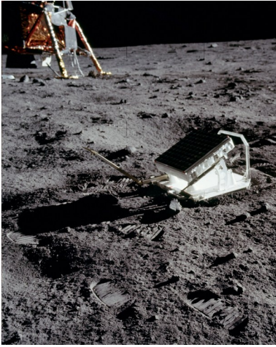
d/The Apollo 11 mission left behind this mirror, which in this photo shows the reflection of the black sky. The mirror is used for lunar laser ranging measurements, which have an accuracy of about a centimeter.
