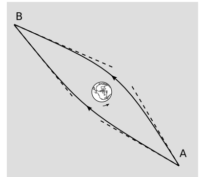
e / Two light rays travel in the earth’s equatorial plane from A to B. Due to frame-dragging, the ray moving with the earth’s rotation is deflected by a greater amount than the one moving contrary to it. As a result, the figure has an asymmetric banana shape. Both the deflection and its asymmetry are greatly exaggerated.
