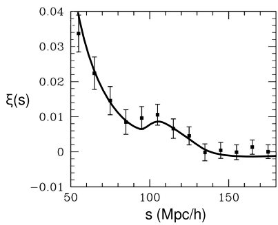
h / The acoustic peak in the BAO correlation function. Redrawn from Eisenstein, New Astronomy Reviews . 49 (2005) 360, as reproduced in Bassett and Hlozek, 2009, arxiv.org/abs/0910.5224 .
