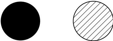
g / The black sphere is made of ordinary matter. The crosshatched sphere has positive gravitational mass and negative inertial mass. If the two of them are placed side by side in empty space, they will both accelerate steadily to the right, gradually approaching the speed of light. Conservation of momentum is preserved, because the exotic sphere has leftward momentum when it moves to the right, so the total momentum is always zero.
