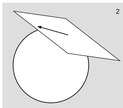
g/1. 1. A tangent vector can be thought of as an infinitesimal displacement. 2. For a sphere embedded in three-space, the space of tangent vectors is visualized as a plane tangent to the sphere at a certain point.
