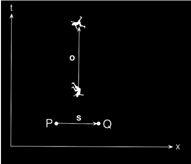
k / The free-falling observer considers P and Q to be simultaneous.
