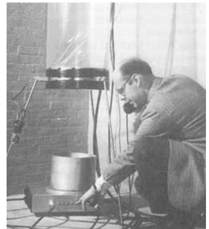
s / Pound and Rebka at the top and bottom of the tower.
