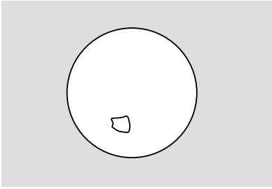
b / We define a boundary around a region whose charge we want to measure.
