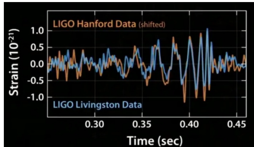
b / The gravitational waveform observed in 2016 by Advanced Ligo.
