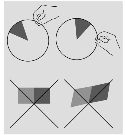
b / The circle plays a privileged role in Euclidean geometry. When rotated, it stays the same. The pie slice is not invariant as the circle is. A similar privileged place is occupied by the light cone in Lorentz geometry. Under a Lorentz boost, the spacetime parallelograms change, but the light cone doesn't.
