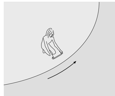
d / Observer A, rotating with the carousel, measures an azimuthal distance with a ruler.
