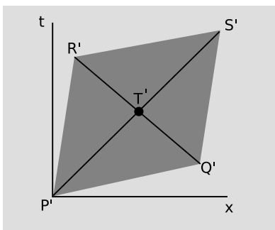
e / Example 8. Flashes of light travel along P'T' and Q'T' . The observer in this frame of reference judges them to have been emitted at different times, and to have traveled different distances.
