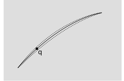
c / The charged particle follows a trajectory that extremizes \int f_b dx^b compared to other nearby trajectories. Relativistically, the trajectory should be understood as a world-line in 3+1-dimensional spacetime.
