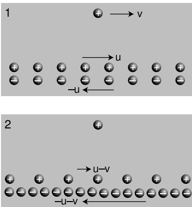
b / Magnetism is a purely relativistic effect.
