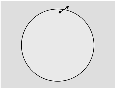
a / A vector can be thought of as lying in the plane tangent to a certain point.
