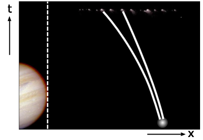
b / Tidal forces cause the initially parallel world-lines of the fragments to diverge. The spacetime occupied by the comet has intrinsic curvature, but it is not caused by any local mass; it is caused by the distant mass of Jupiter.
