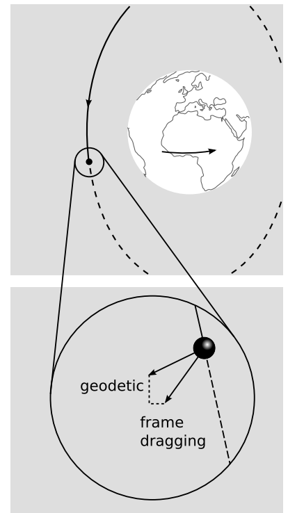
f / Gravity Probe B verified the existence of frame-dragging. The rotational axis of the gyroscope precesses in two perpendicular planes due to the two separate effects: geodetic and frame-dragging.
