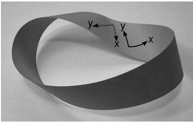
a / A Möbius strip is not an orientable surface.
