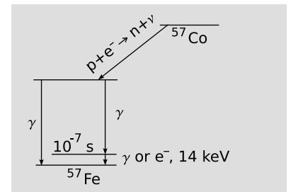
q / Emission of 14 keV gamma-rays by ^{57}\text{Fe} . The parent nucleus ^{57}\text{Co} absorbs an electron and undergoes a weak-force decay process that converts it into ^{57}\text{Fe} , in an excited state. With 85% probability, this state decays to a state just above the ground state, with an excitation energy of 14 keV and a half-life of 10^{-7} s. This state finally decays, either by gamma emission or emission of an internal conversion electron, to the ground state.
