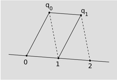
d / Construction of an affine parameter.
