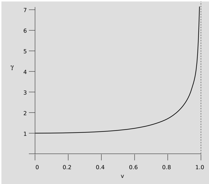
d / The behavior of the \gamma factor.
