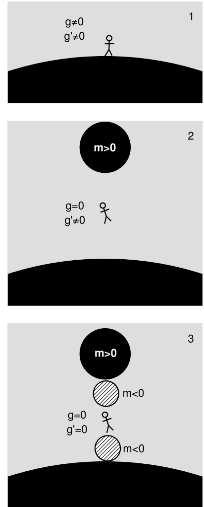
h / Nulling out a gravitational field is impossible in one dimension without exotic matter. 1. The planet imposes a nonvanishing gravitational field with a nonvanishing gradient. 2. We can null the field at one point in space, by placing a sphere of very dense, but otherwise normal, matter overhead. The stick figure still experiences a tidal force, g' \neq 0 . 3. To change the field’s derivative without changing the field, we can place two additional masses above and below the given point. But to change its derivative in the desired direction — toward zero — we would have to make these masses negative.
