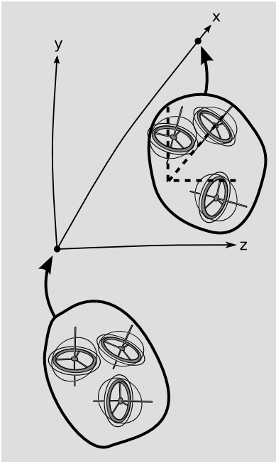
c / Three gyroscopes are initially aligned with the x , y , and z axes. After parallel transport along the geodesic x axis, the x gyro is still aligned with the x axis, but the y and z gyros have rotated.
