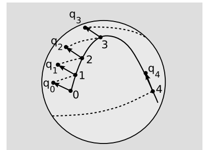
c / Bad things happen if we try to construct an affine parameter along a curve that isn't a geodesic. This curve is similar to path ABC in figure b. Parallel transport doesn't preserve the vectors' angle relative to the curve, as it would with a geodesic. The errors in the construction blow up in a way that wouldn't happen if the curve had been a geodesic. The fourth dashed parallel flies off wildly around the back of the sphere, wrapping around and meeting the curve at a point, 4, that is essentially random.
