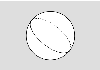
c / This boundary cuts the sphere into equal parts.
