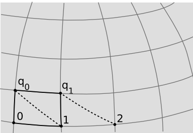
a / Construction of an affine parameter in curved spacetime.
