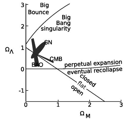
i / The cosmological parameters of our universe, after Perlmutter, 1998, arxiv.org/abs/astro-ph/9812133 and Kowalski, 2008, arxiv.org/abs/0804.4142 . The three shaded regions represent the 95% confidence regions for the three types of observations.
