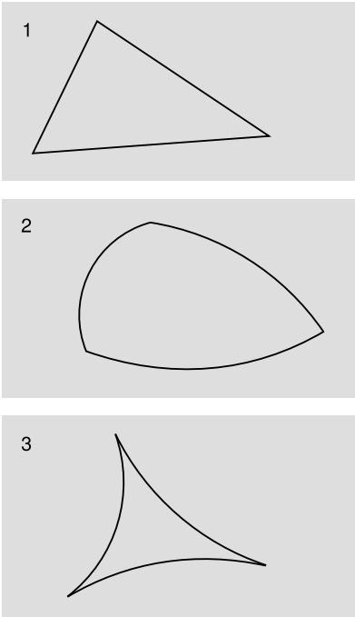
b / 1. In the Euclidean plane, this triangle can be scaled by any factor while remaining similar to itself. 2. In a plane with positive curvature, geometrical figures have a maximum area and maximum linear dimensions. This triangle has almost the maximum area, because the sum of its angles is nearly 3\pi . 3. In a plane with negative curvature, figures have a maximum area but no maximum linear dimensions. This triangle has almost the maximum area, because the sum of its angles is nearly zero. Its vertices, however, can still be separated from one another without limit.
