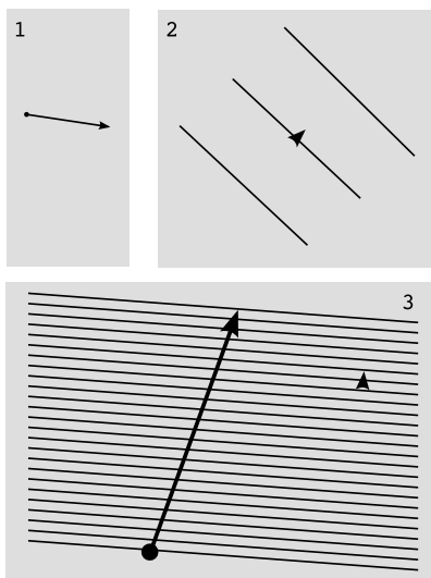
h / 1. A displacement vector. 2. A vector from the space dual to the space of displacements. 3. Measurement is reduced to counting. The cuckoo clock chimes 24 times in one rotation of the earth.
