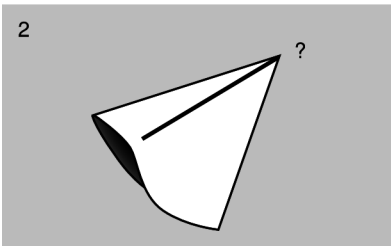
b / A conical singularity. The cone has zero intrinsic curvature everywhere except at its tip. Geodesic 1 can be extended infinitely far, but geodesic 2 cannot; since the metric is undefined at the tip, there is no sensible way to define how geodesic 2 should be extended.
