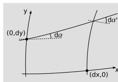
h / 1. Gaussian curvature can be interpreted as the failure of parallelism represented by d^2 \alpha/dx dy .
