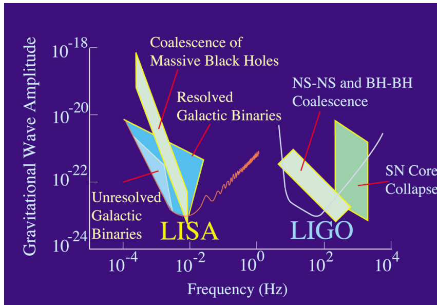
c / Predicted sensitivities of LISA and LIGO to gravitational waves of various frequencies.
