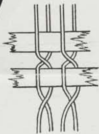
Scheringsdraden by de verdelingslatten
