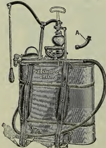
"Success" Sprayer.
