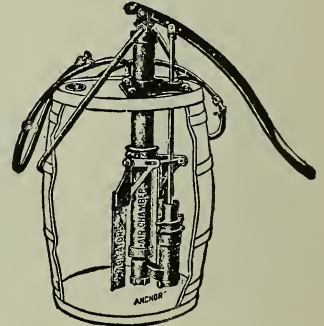
"POMONA" BARREL SPRAY PUMP
