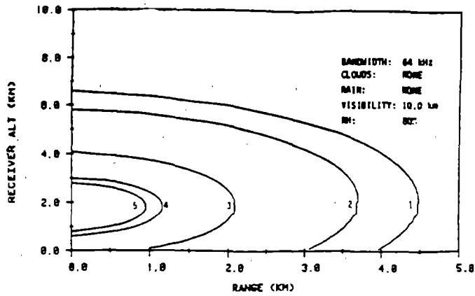
Figure A. Effective Communications range for receiver altitudes 0-10 km at various frequencies in clear air.
