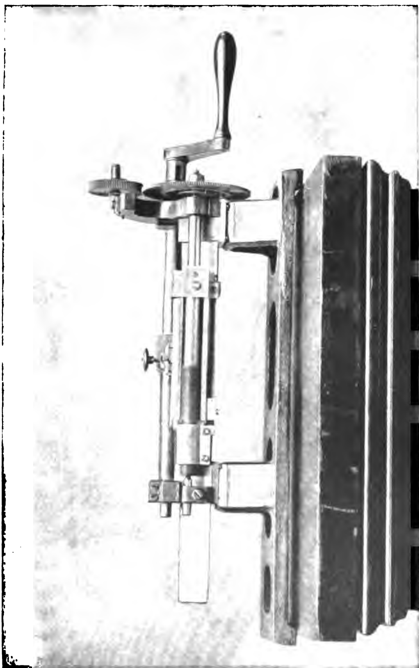
MACHINE BY WHICH THE ENDLESS SCREW AND THE TEETH ON THE PLATE OF THE RAMSDEN DIVIDING ENGINE WERE CUT.
