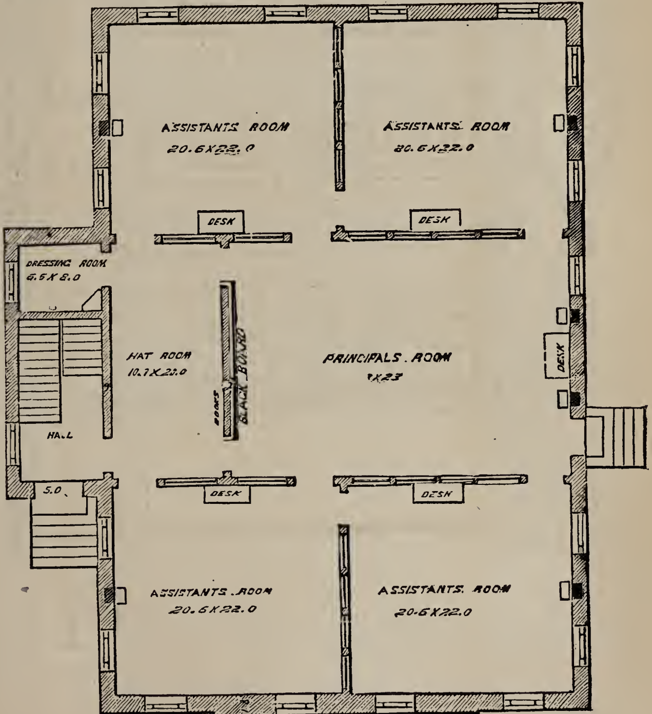
FIRST STORY—PRIMARY SCHOOL.
