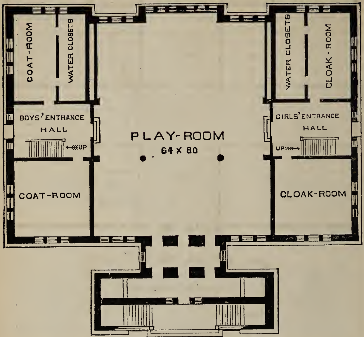
PLAN OF BASEMENT
