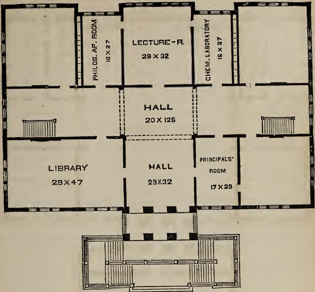
PLAN OF FIRST STORY
