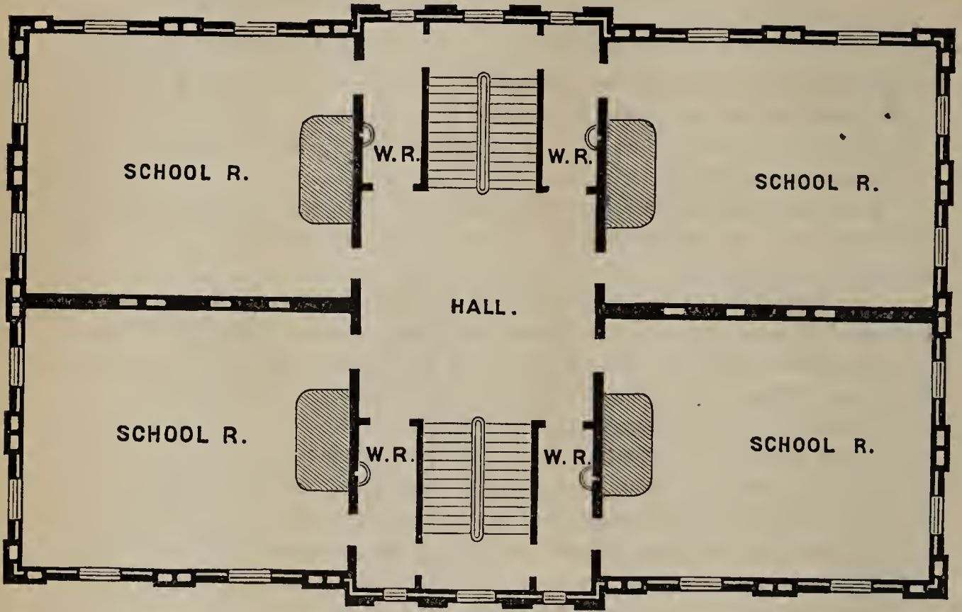
FIRST AND SECOND FLOORS.
