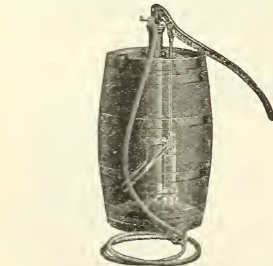
DEMING'S "CENTURY" BARREL SPRAY PUMP
