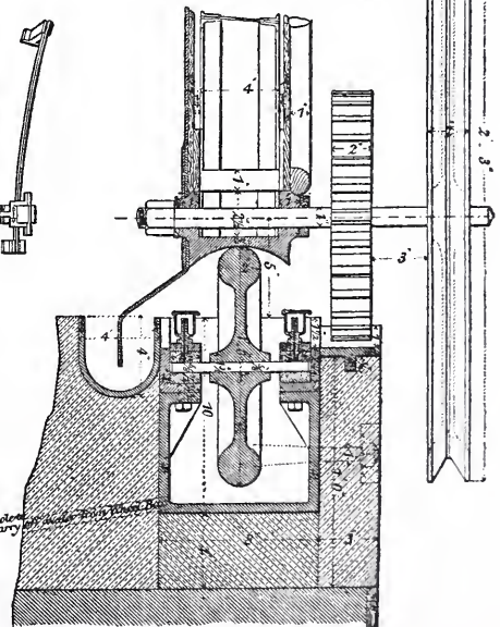
Fig. 4. Section thro' Wheel Box & Showing V Wheel and Pinions.
