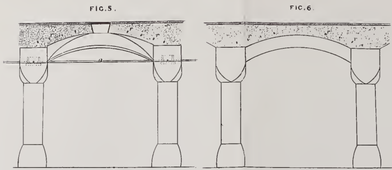
Section on A B Groined Vaulting
