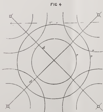
Plan a. a. 2" Diagonal ties. r. r. r. concentric ring ties.
