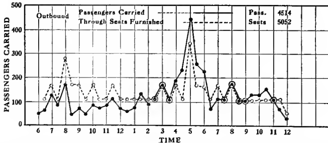
FIG. 21.—Pittsburgh suburban line. At top, traffic graph of suburban line showing results with seven cars; at center and bottom, half-hourly load graphs for same route, inbound and outbound.
