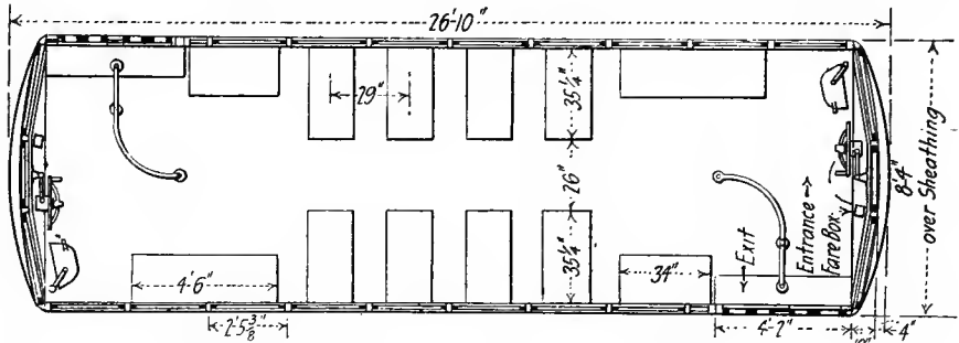
Fig. 52.—One-man car for double-end operation (Albuquerque, N. M.).
