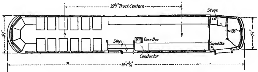
FIG. 50.—Front-entrance, center-exit car (Cleveland).
