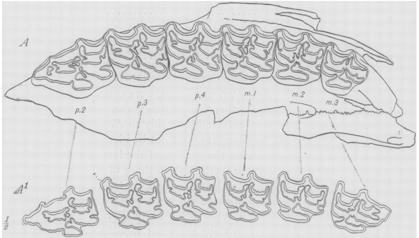
Fig. 22. E. complicatus . (Tule Cañon, Texas.) Superior molar-premolar series of right side sectioned to show change in teeth due to wear. A , tritulating surfaces; A¹ , sections cut parallel to the tritulating surface about the middle of the crowns. (No. 10611, Coll. A. M. N. H.).
