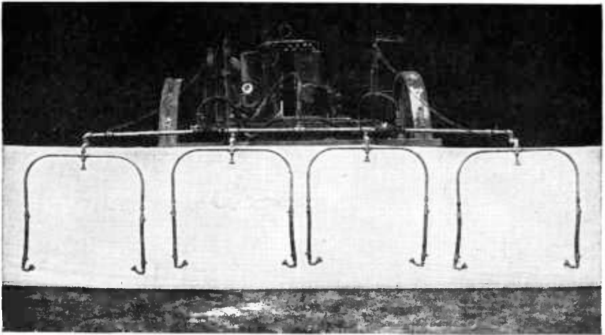
Figure 7. —A series of nozzles attached to a rigid boom.
