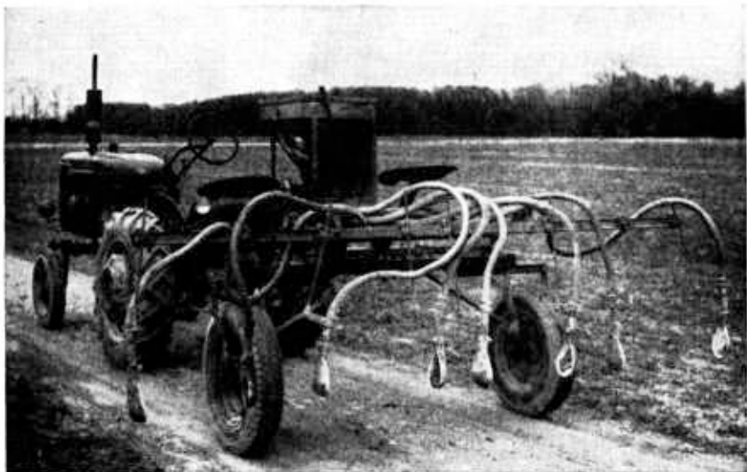
Figure 10. —A four-row tractor-drawn power duster.
