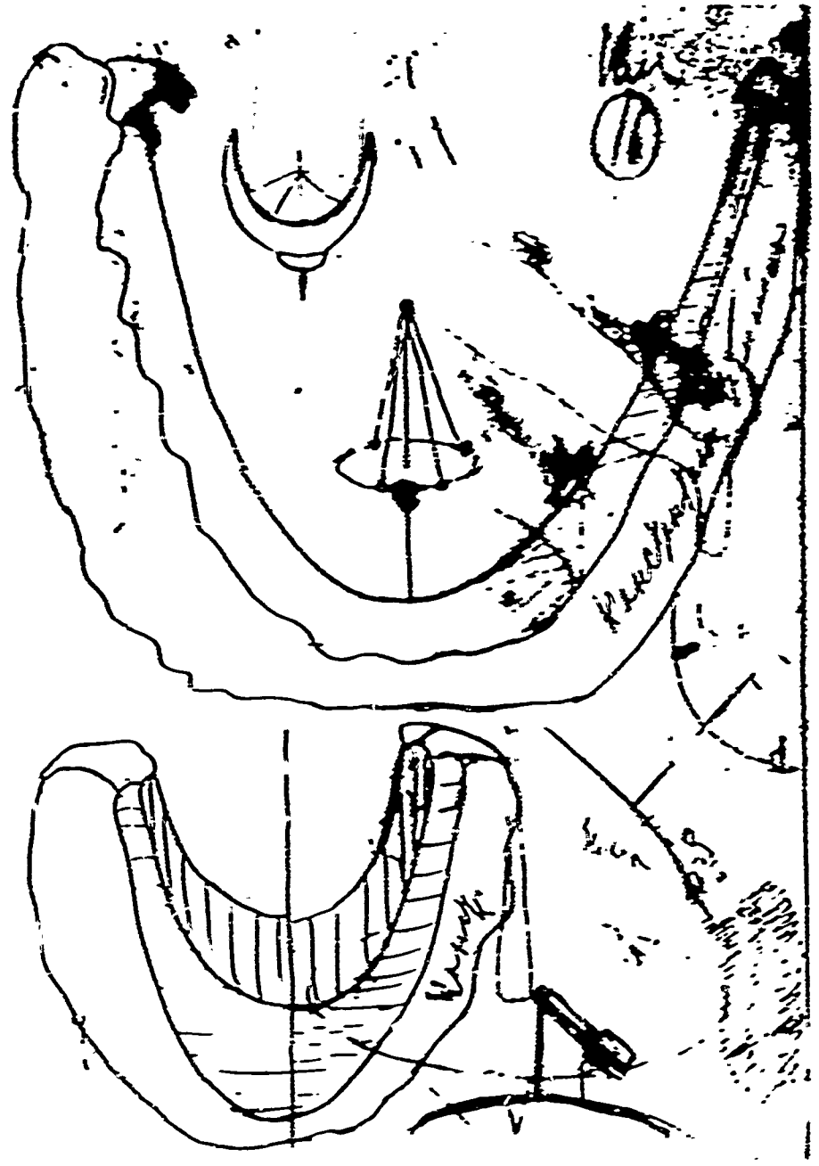
Liquid takes a shape (body) of revolution.
