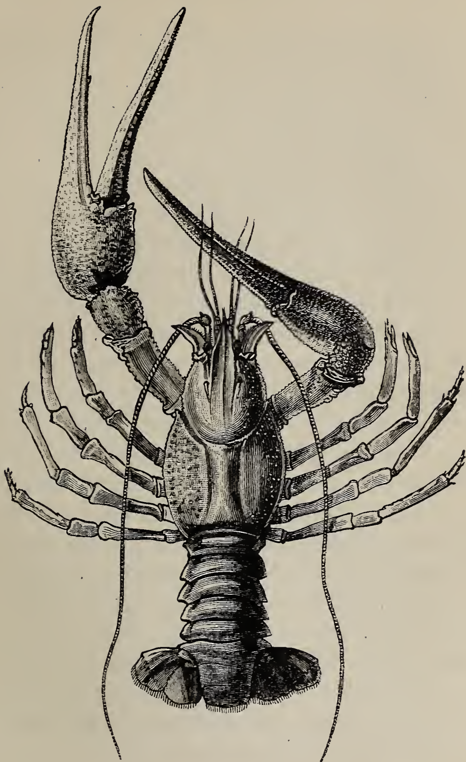
FIG. 75.— Astacus leptodactylus (after Rathke, \frac{1}{3} nat. size).
