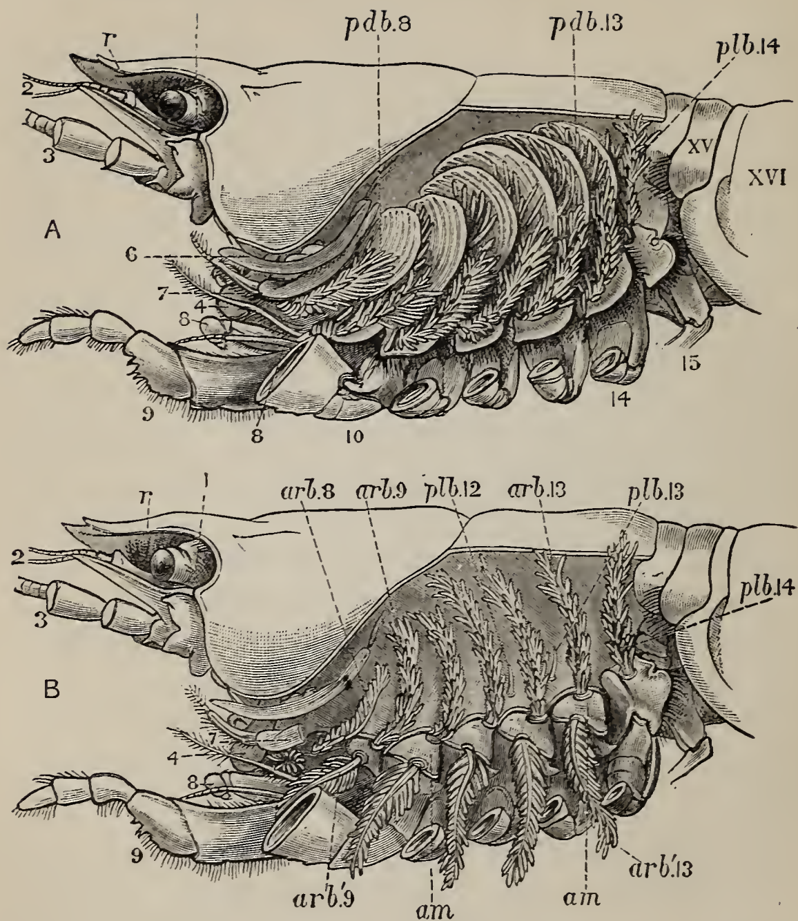
FIG. 4.— Astacus fluviatilis .—In A, the gills, exposed by the removal of the branchio-stegite, are seen in their natural position ; in B, the podobranchiæ (see p. 75) are removed, and the anterior set of arthrobranchiæ turned downwards ( \times 2 ): 1, eye-stalk ; 2, antennule ; 3, antenna ; 4, mandible ; c, scaphognathite ; 7, first maxillipede, in B the epipodite, to which the line points, is partly removed ; 8, second maxillipede ; 9, third maxillipede ; 10, forceps ; 14, fourth ambulatory leg ; 15, first abdominal appendage ; xv., first, and xvi., second abdominal somite ; arb. 8, arb. 9, arb. 13, the posterior arthrobranchiæ of the second and third maxillipedes and of the third ambulatory leg ; arb'. 9, arb'. 13, the anterior arthrobranchiæ of the third maxillipede and of the third ambulatory leg ; pbd. 8, podobranchiæ of the second maxillipede ; pbd. 13, that of the third ambulatory leg ; plb. 12, plb. 13, the two rudimentary pleurobranchiæ ; plb. 14, the functional pleurobranchia ; r, rostrum.
