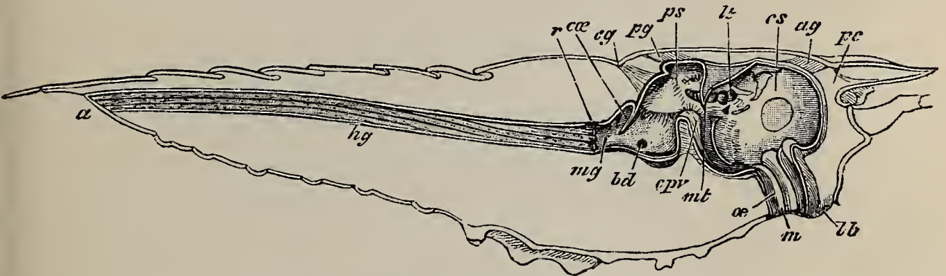
FIG. 6.— Astacus fluviatilis .—A longitudinal vertical section of the alimentary canal, with the outline of the body (nat. size):— a , vent; ag , anterior gastric muscle; bd , entrance of left bile duct; cg , cervical groove; cæ , cæcum; cpv , cardio-pyloric valve; cs , cardiac portion of stomach; the circular area immediately below the end of the line from cs marks the position of the gastrolith of the left side; hg , hind-gut; lb , labrum; lt , lateral tooth of stomach; m , mouth; mg , mid-gut; mt , median tooth; œ , œsophagus; pc , procephalic process; pg , posterior gastric muscle; ps , pyloric portion of stomach; r , annular ridge, marking the commencement of the hind-gut.
