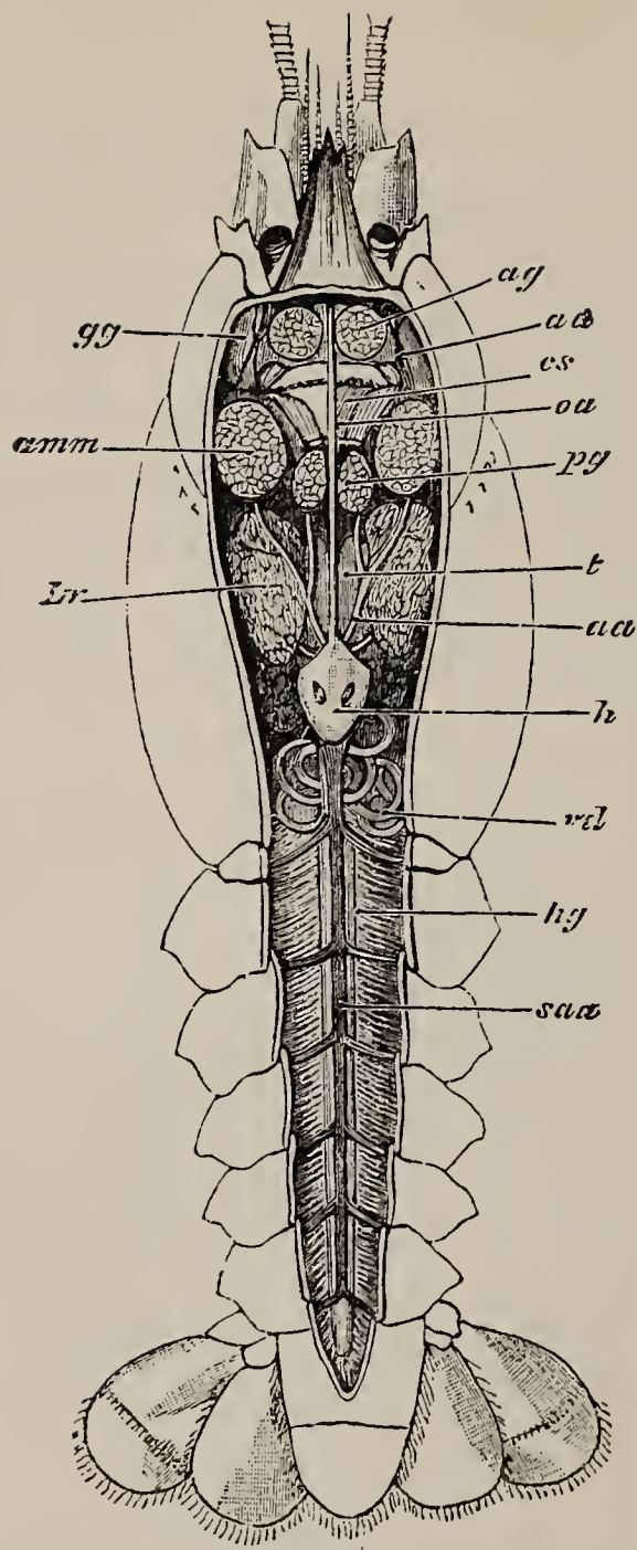
FIG. 5.— Astacus fluviatilis .—A male specimen, with the roof of the carapace and the terga of the abdominal somites removed to show the viscera (nat. size) :— aa , antennary artery ; ag , anterior gastric muscles ; amm , adductor muscles of the mandibles ; cs , cardiac portion of the stomach ; gg , green glands ; h , heart ; hg , hind gut, or large intestine ; Lr , liver ; oa , ophthalmic artery ; pg posterior gastric muscles ; saa , superior abdominal artery ; t , testis ; vd , vas deferens.
