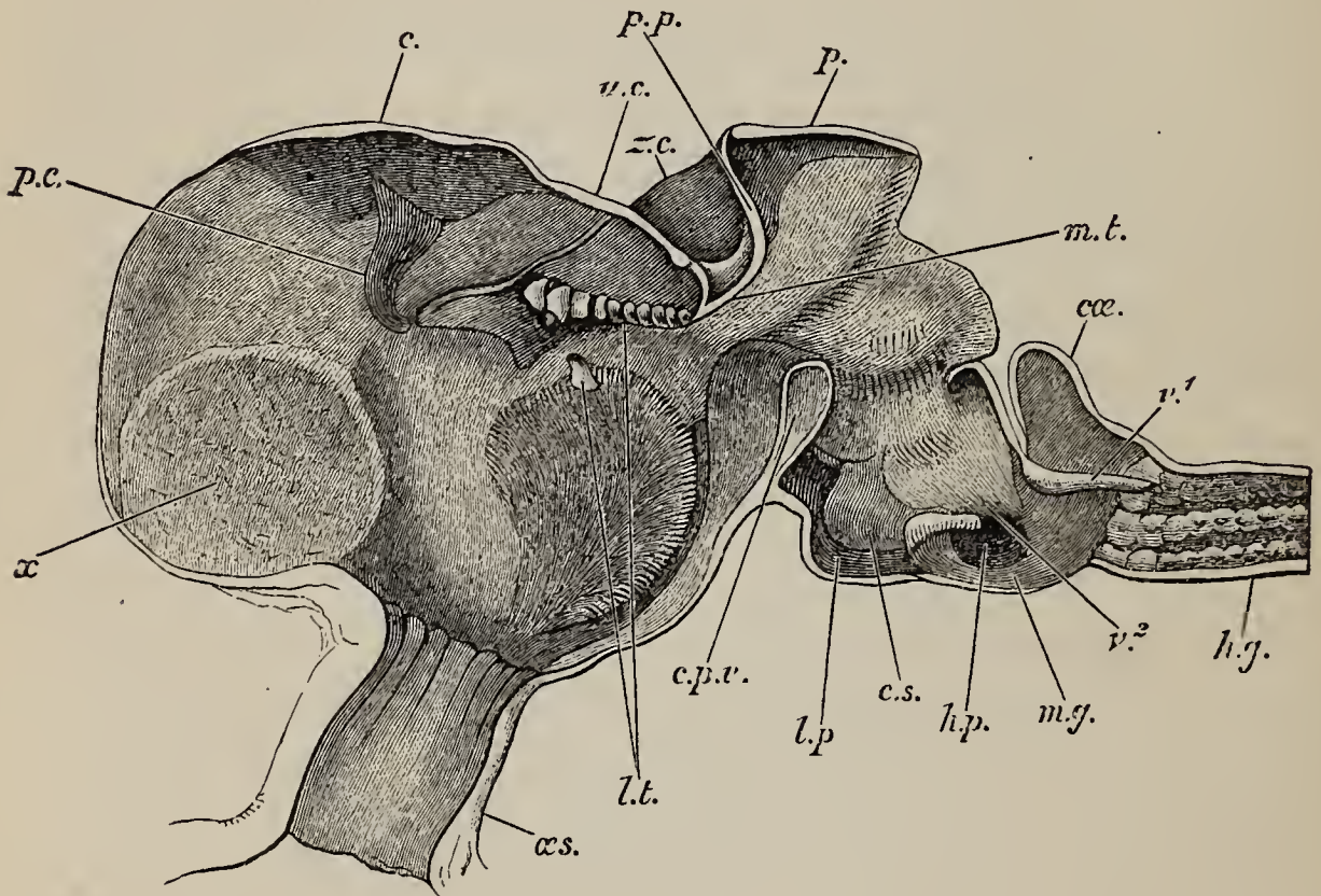
FIG. 10.— Astacus fluviatilis .—Longitudinal section of the stomach ( \times 4 ). c , cardiac ossicle; cae , caecum; c.p.v. , cardio-pyloric valve; cs , cushion-shaped surface; hg , hind-gut; hp , aperture of right bile duct; lp , lateral pouch; lt , lateral teeth; mg , mid-gut; mt , median tooth; as , oesophagus; p , pyloric ossicle; pc , pterocardiac ossicles; pp , prepyloric ossicle; uc , urocardiac process; v 1 , median pyloric valve; v 2 , lateral pyloric valve; x , position of gastrolith; zc , zygocardiac ossicle.
