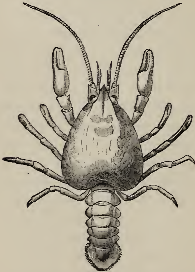
FIG. 60.— Astacus fluviatilis .—Newly-hatched young ( \times 6 ).
