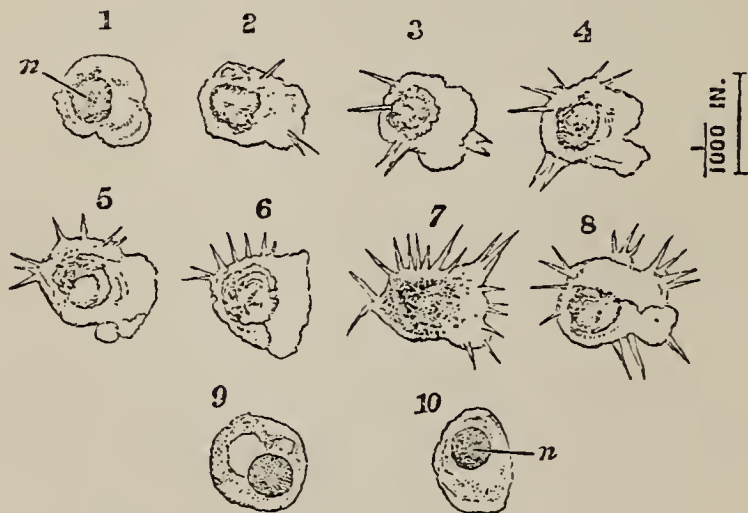
FIG. 14.— Astacus fluviatilis .—The corpuscles of the blood (highly magnified). 1-8 show the changes undergone by a single corpuscle during a quarter of an hour; 9 and 10 are corpuscles killed by magenta, and having the nucleus deeply stained by the colouring matter. n , nucleus.
