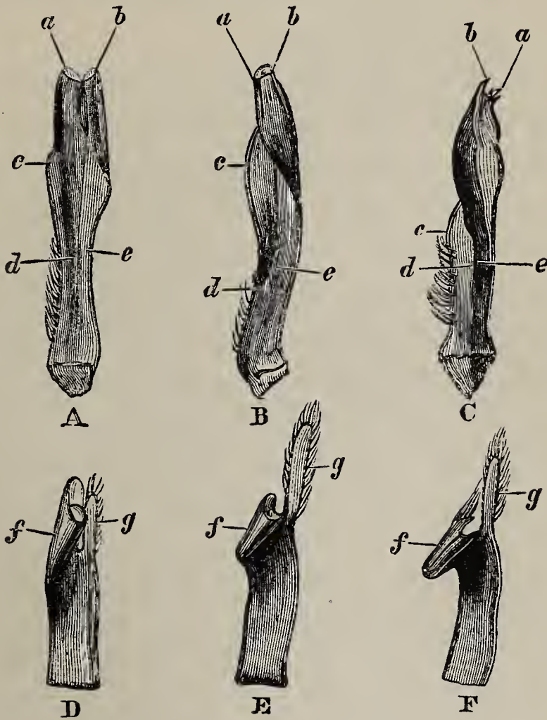
FIG. 62. A & D, Astacus torrentium ; B & E, A. nooilis ; C & F, A. nigrescens . A—C, 1st abdominal appendage of the male; D—F, endopodite of second appendage ( \times 3 ). a , anterior, and b , posterior rolled edge; c , d , e , corresponding parts of the appendages in each species; f , rolled plate of endopodite; g , terminal division of endopodite.
