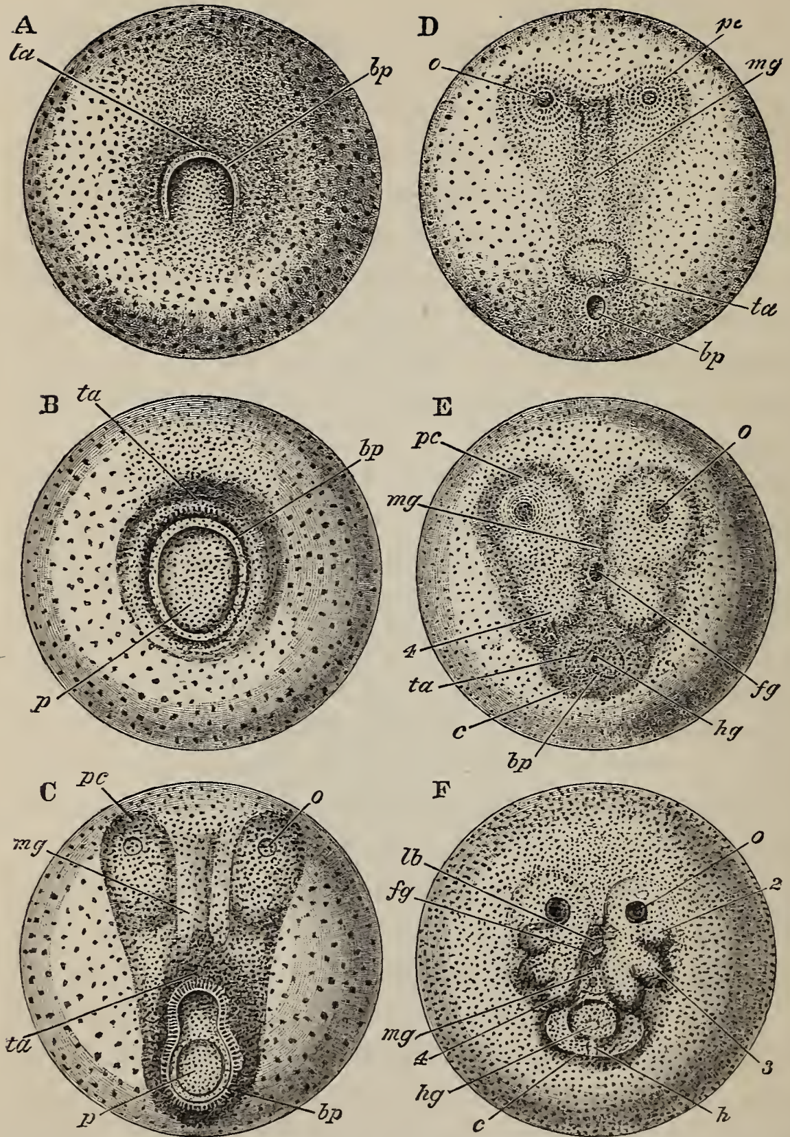
FIG. 58.— Astacus fluviatilis .—Surface views of the earlier stages in the development of the embryo, from the appearance of the blastopore (A) to the assumption of the nauplius form (F) (after Reichenbach, \times about 23). bp , blastopore; c , carapace; fg , fore-gut involution; h , heart; hg , hind-gut involution; lb , labrum; mg , medullary groove; o , optic pit; p , endodermal plug partly filling up the blastopore; pc , procephalic processes; ta , abdominal elevation; 2, antennules; 3, antennæ 4, mandibles.
