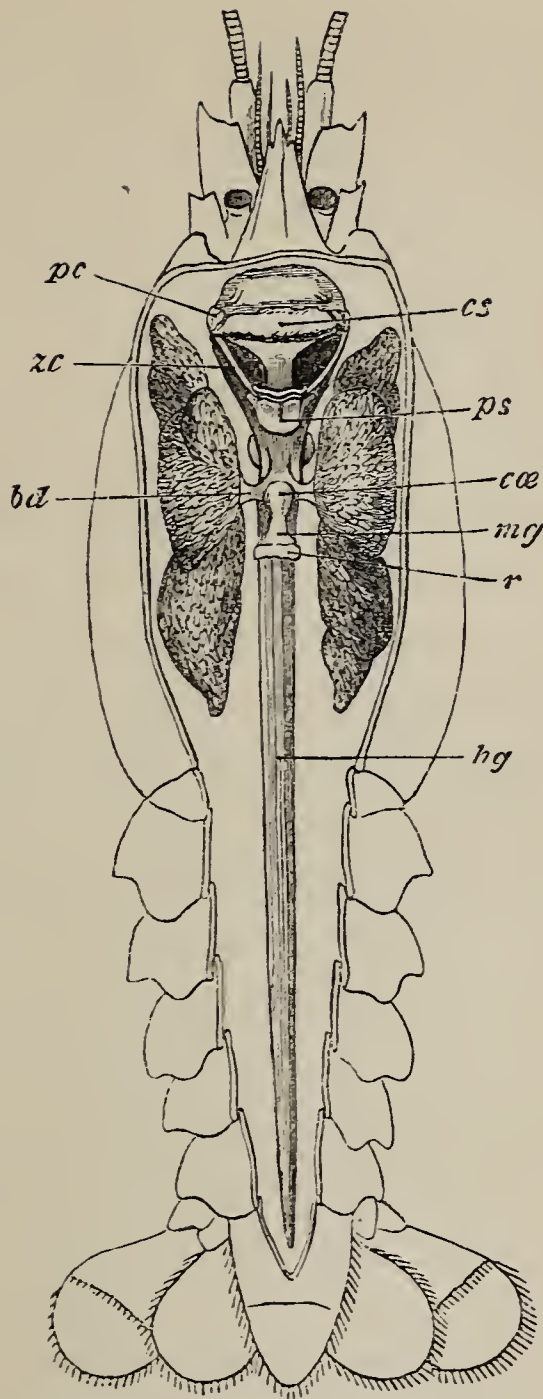
FIG. 13.— Astacus fluviatilis .—The alimentary canal and livers seen from above (nat. size). bd , bile-duct ; cae , caecum ; cs , cardiac portion of stomach, the line pointing to the cardiac ossicle ; hg , hind-gut ; mg , mid-gut ; pc , ptero-cardiac ossicle ; ps , pyloric portion of stomach, the line pointing to the pyloric ossicle ; r , ridge separating mid-gut from hind-gut ; zc , zygo-cardiac ossicle.
