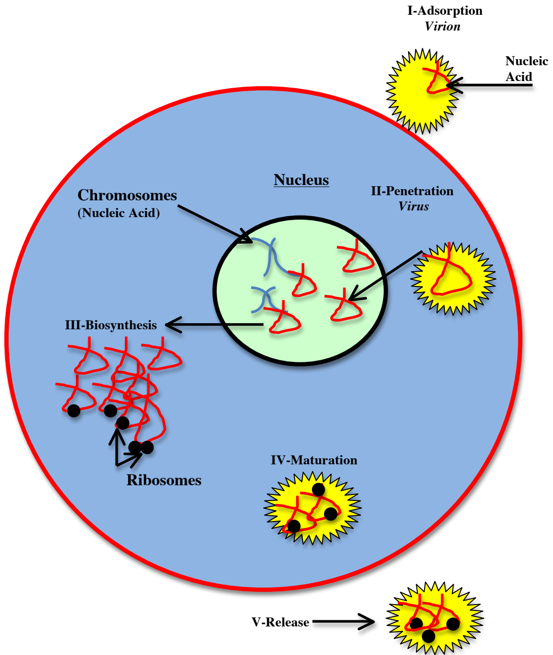
Figure 23.1: Viral Reproduction
