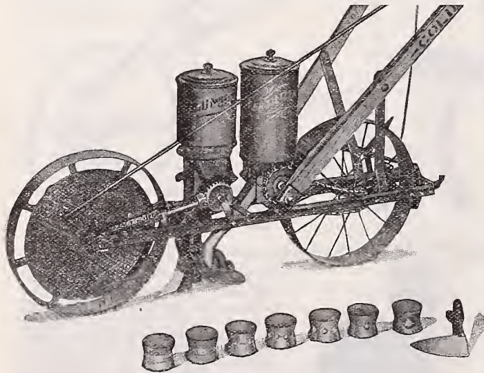
Columbia No. 11 Garden Seed Drill
