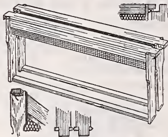
Self-Spacing Hoffman Frame.
