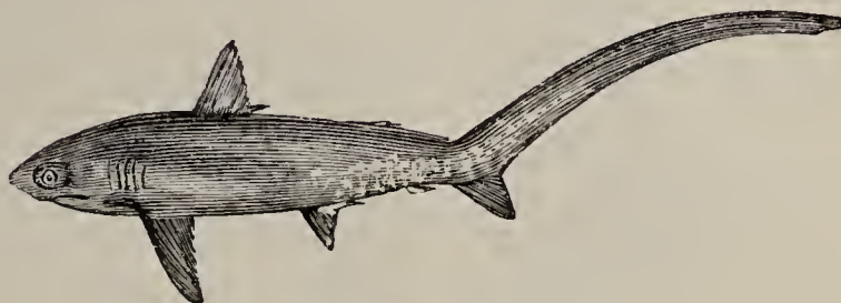
FIG. 198.—Thresher shark.
