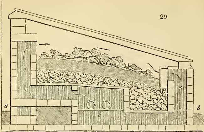
Section of proposed Pit on the line a b of fig. 30.
