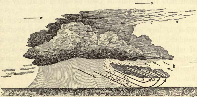
FIG. 7.—SECTIONAL DIAGRAM OF A SQUALL. AFTER MÜLLER.
