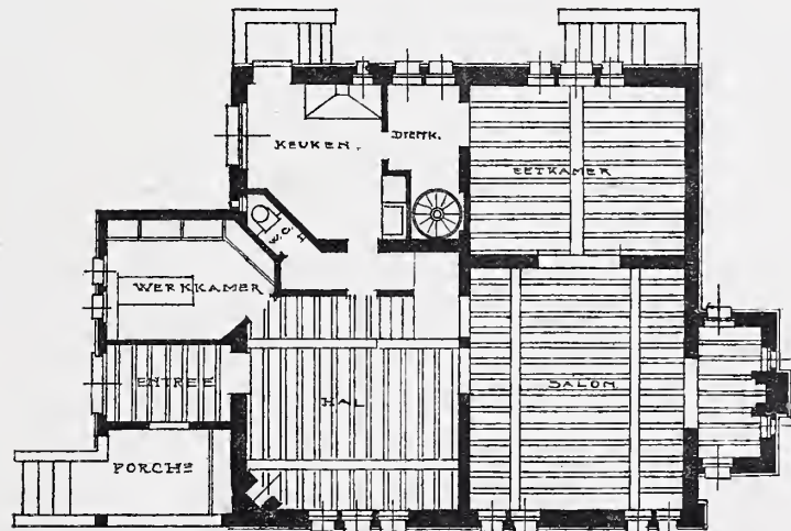
BEGANE-GROND
