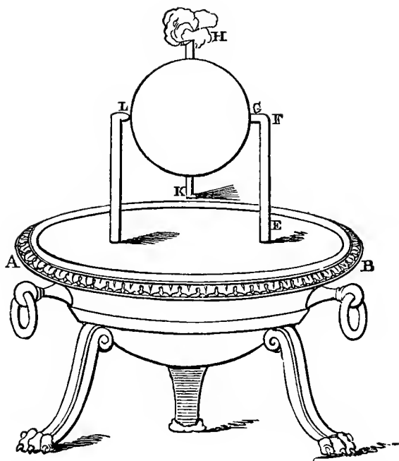
THE STEAM-ENGINE OF HERO
