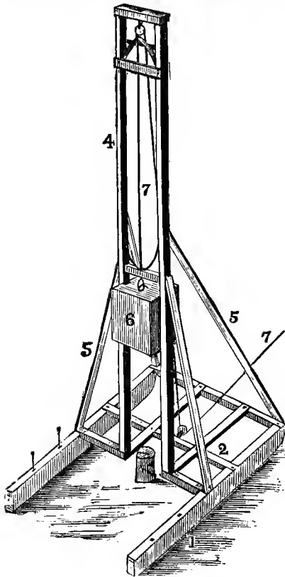
SPILE OR POST DRIVER.
