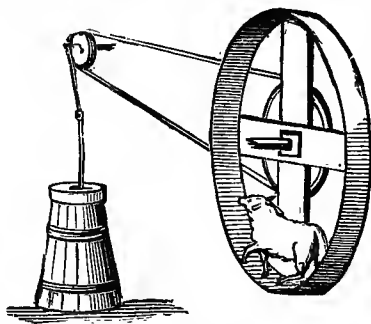
POWER FOR CHURNING.—FIG. 2.
