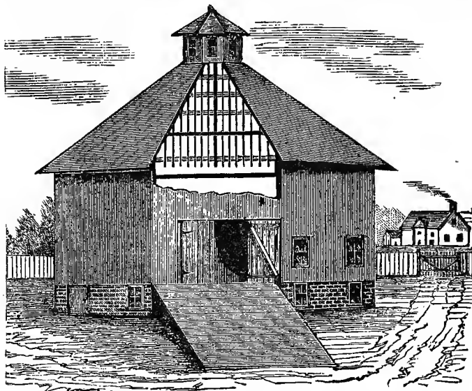
FIG. 1.—ELEVATION OF AN OCTAGONAL BARN.
