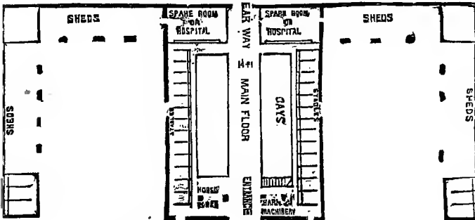
A COMPLETE STOCK BARN.—GROUND PLAN.
