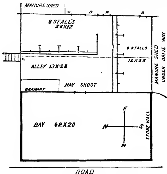
AN OLD BARN IMPROVED.—PLAN OF BASEMENT.
