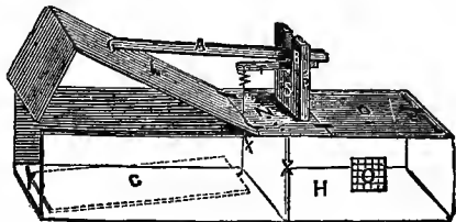
A MINK TRAP.
