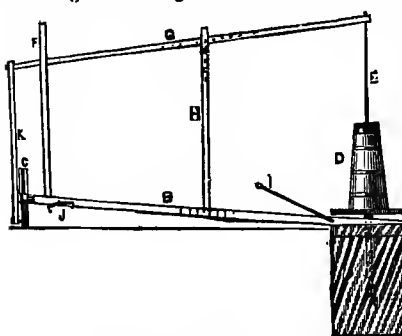
POWER FOR CHURNING.—FIG. 4.
