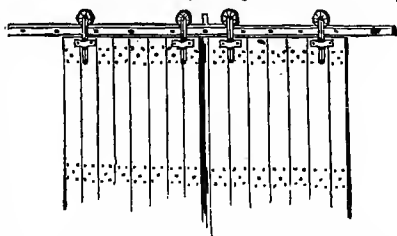
FIG. 2.—MANNER OF APPLYING THE ROLLERS.
