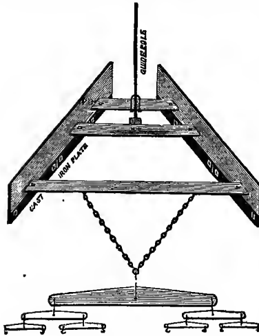
A GOOD ROAD SCRAPER.
