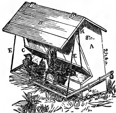
FIG. 2.—A PERFECT FEEDING HOPPER.
