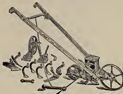
PLANET JR. No. 25 COMBINED SEEDER AND DOUBLE WHEEL HOE Price $21.00
