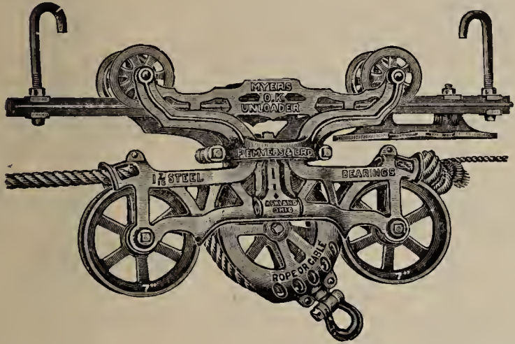
Reversible and Swivel
