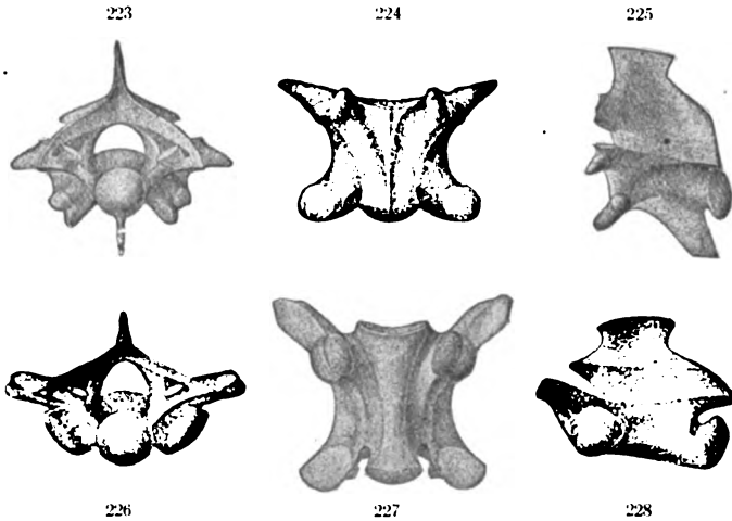
FIGS. 223-228. - POSTERIOR DORSAL VERTEBRÆ OF SNAKES. 223, BACK VIEW; 224, LOWER VIEW; 225, SIDE VIEW OF VERTEBRA WITH HYPAPOPHYSIS; 226, BACK VIEW; 227, LOWER VIEW; 228, SIDE VIEW OF VERTEBRA WITHOUT HYPAPOPHYSIS (COPIED FROM BOULENGER, CAT. SNAKES BRIT. MUS., I 1893, p. 171.)
