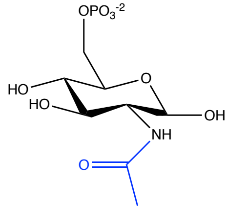
N-acetyl-D-glucosamine-6-phosphate
