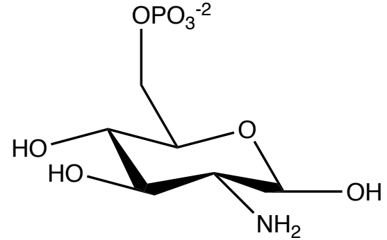
D-Glucosamine 6-phosphate
