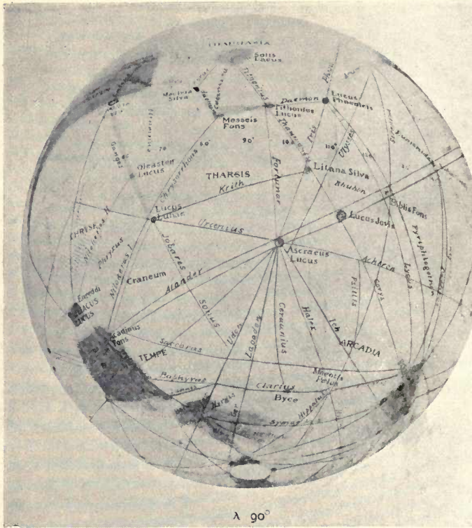
LOWELL'S MAP OF MARS, at the opposition of 1903, showing Solis Lacus near the T (From "Nature," Oct. 11th, 1906.)
