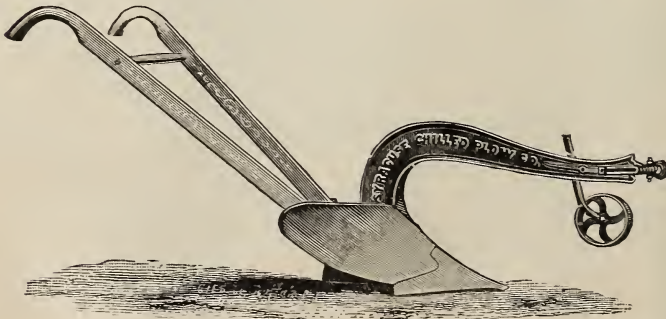
Iron Beam and set over Clevis.
