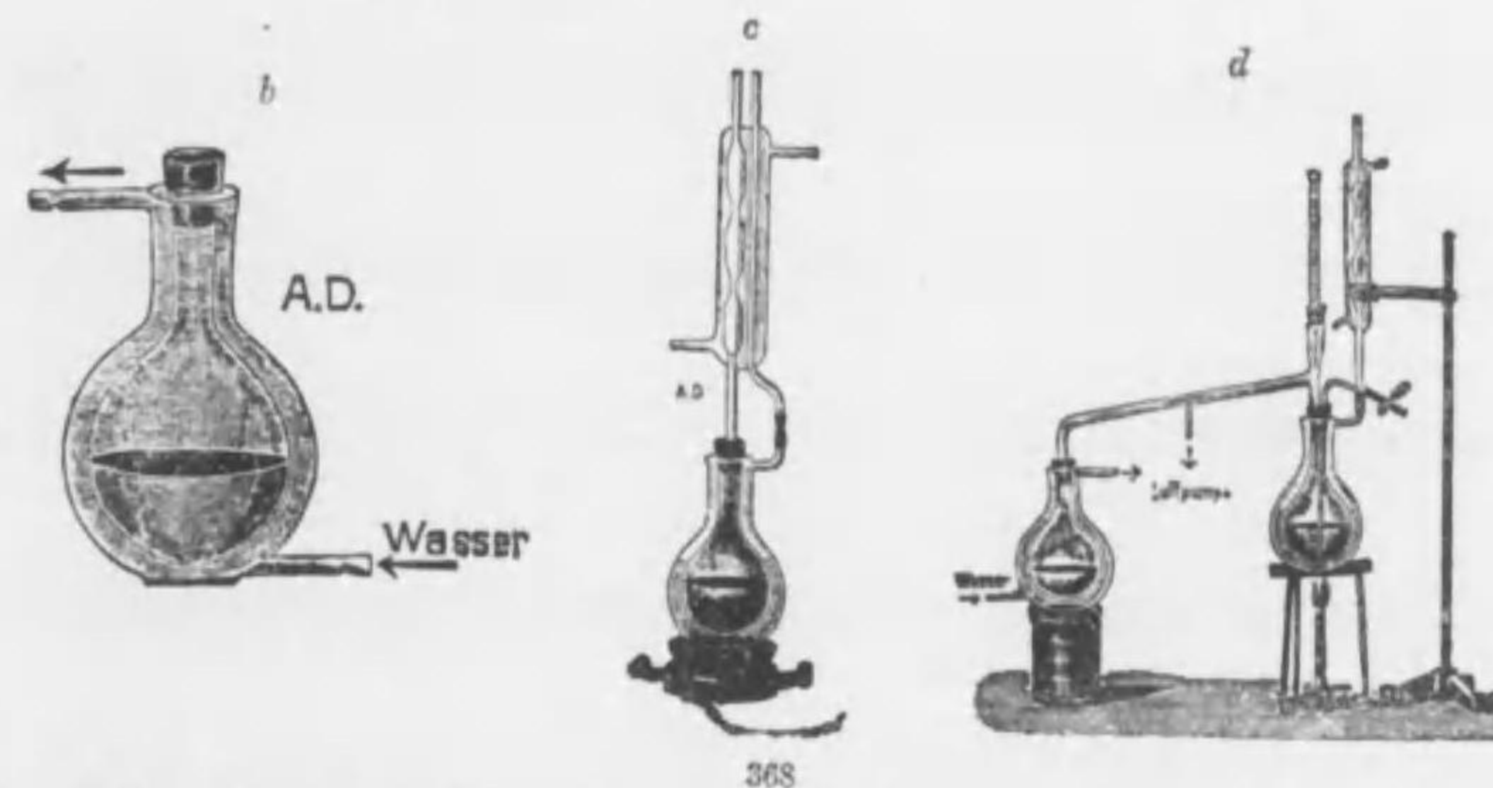
*368 二重フラスコ (ツエルマノウイツチ氏) Double Flasks, advantageous for the experiment of organic matters.
