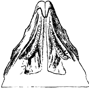
Fig. 6.—Skull of Sphenodon , under view.
