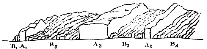
Fig. 4.— At Roscoff. (Length about 7 feet.)
