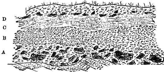
Fig. 2.—Section at Stopham Bridge .
