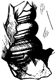
Fig. 1. — Murchisonia zonata , Donald. Nat. size.
