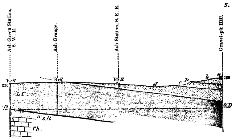
Fig. 2.—Section from Gravel-pit Hill to Ash Green, S. W. R.
