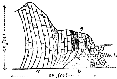
Fig. 2.—Section in Railway-cutting north of Moutier Station.
