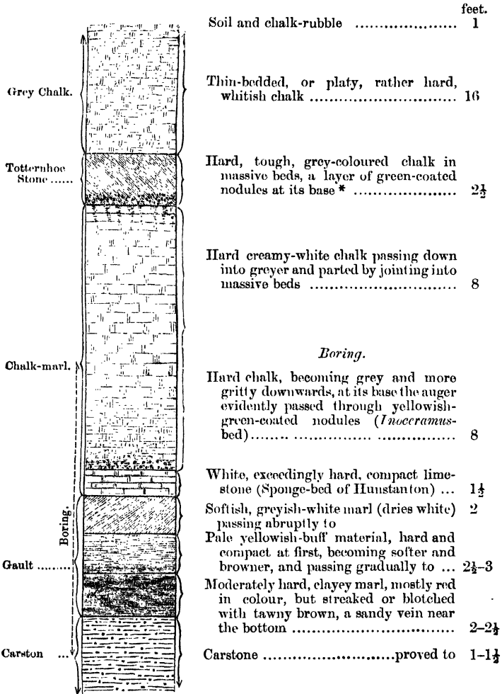
Fig. 4.—Diagram of the section shown and obtained by boring in the Dersingham Parish Chalk-pit. (Scale \frac{1}{8} inch to 1 foot.)
