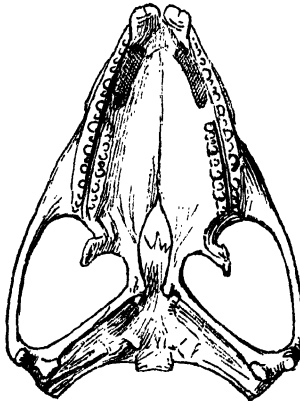
Fig. 6.—Skull of Sphenodon , under view.
