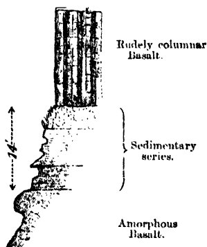
Fig. 4.— Exposure in Second Ravine, Ardtun Head.
