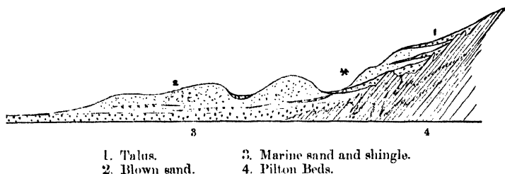
Fig. 2.—Diagram showing Succession of Deposits West of Saunton Court.
