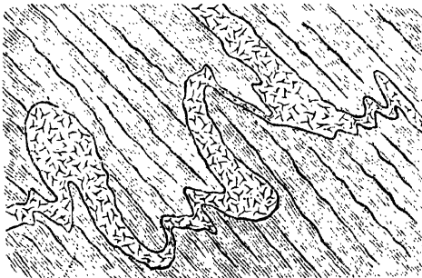
Fig. 1.— Contorted Granite-vein in Gneiss.
