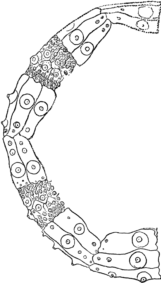
Fig. 6.— Half the Aboral Surface of Pelanechinus corallinus. \times 1\frac{1}{8} .
