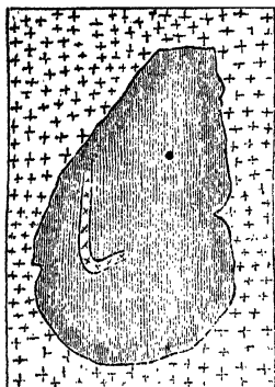
Fig. 5.—Phonolite-inclusion in Foyaité, one sixth natural size.
