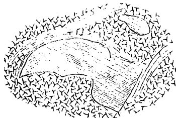
Fig. 3.—Section of Diorite in foliated Granite.
