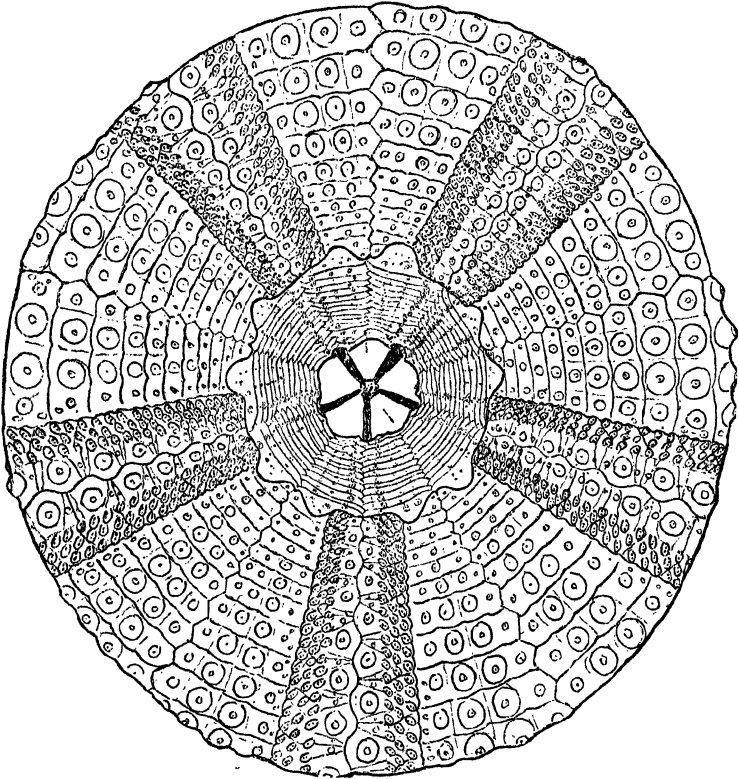
Fig. 5.— Oral Surface of Pelanechinus corallinus (restored). Nat. size.
