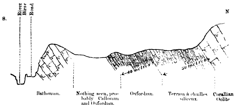
Fig. 1.—Section in Quarry near Roadside, south-east of Liesberg.
