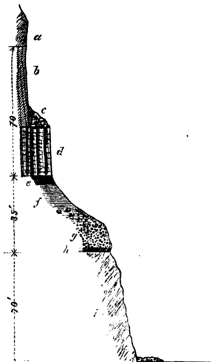
Fig. 7.—Section of lower part of Cliff at Malcolm's Point, near Carsnij. (Scale about 50 feet to 1 inch.)
