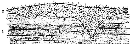
Fig. 8.—Section at Selmeston Church.
