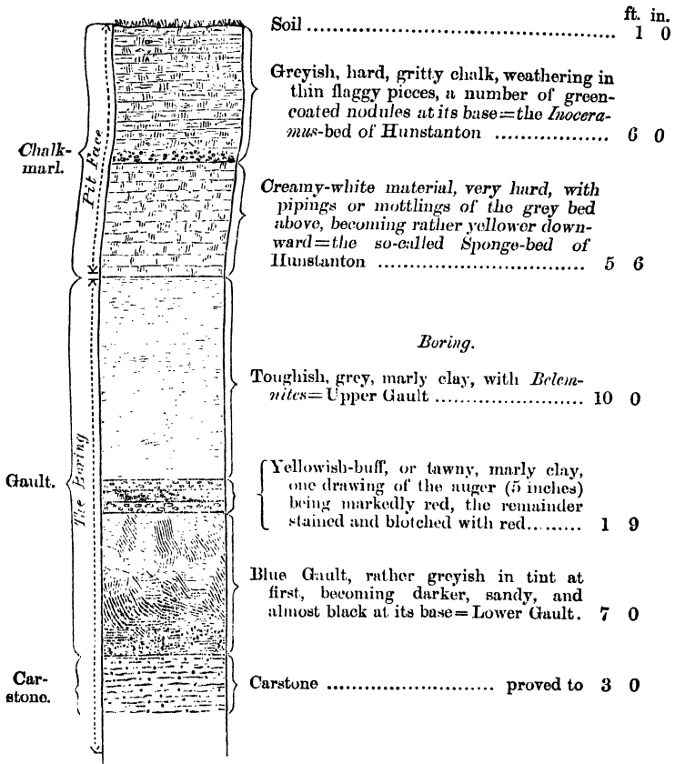
Fig. 2.—Diagram of Section shown and obtained by boring in the Pit about \frac{1}{2} mile N.N.E. of Roydon Church. (Scale \frac{1}{8} inch to 1 foot.)
