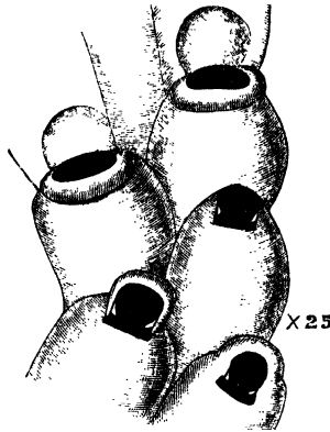
Fig. 1.— Lepralia bistata , Waters, from Waipukurau, New Zealand.
