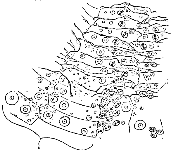
Fig. 4.—One of the Rows of Imbricating Actinal Plates in Pelanechinus corallinus , with the adjacent interambulacral (i) and ambulacral (a) areas. ×3.
