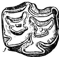
Equus , sp. A right upper cheek-tooth (? m.1 ), from the Upper Tertiary of the Nile valley at Wadi Halfa. †. e anterior, and f posterior inner pillar.
