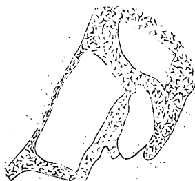
Fig. 1.— Section of Granite in Jointed Diorite.
