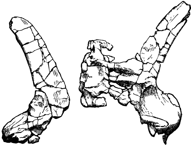
Fig. 2.— Pelvis of Omosaurus durobrivensis , Hulke , from the Kimmeridge Clay of Northamptonshire . One-tenth natural size.
