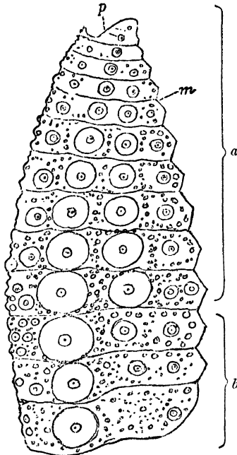
Fig. 1.—Portion of an Interambulacral Area of Pelanechinus corallinus . \times 2 .
