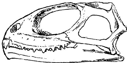
Fig. 3.—Skull of Sphenodon , side view.
