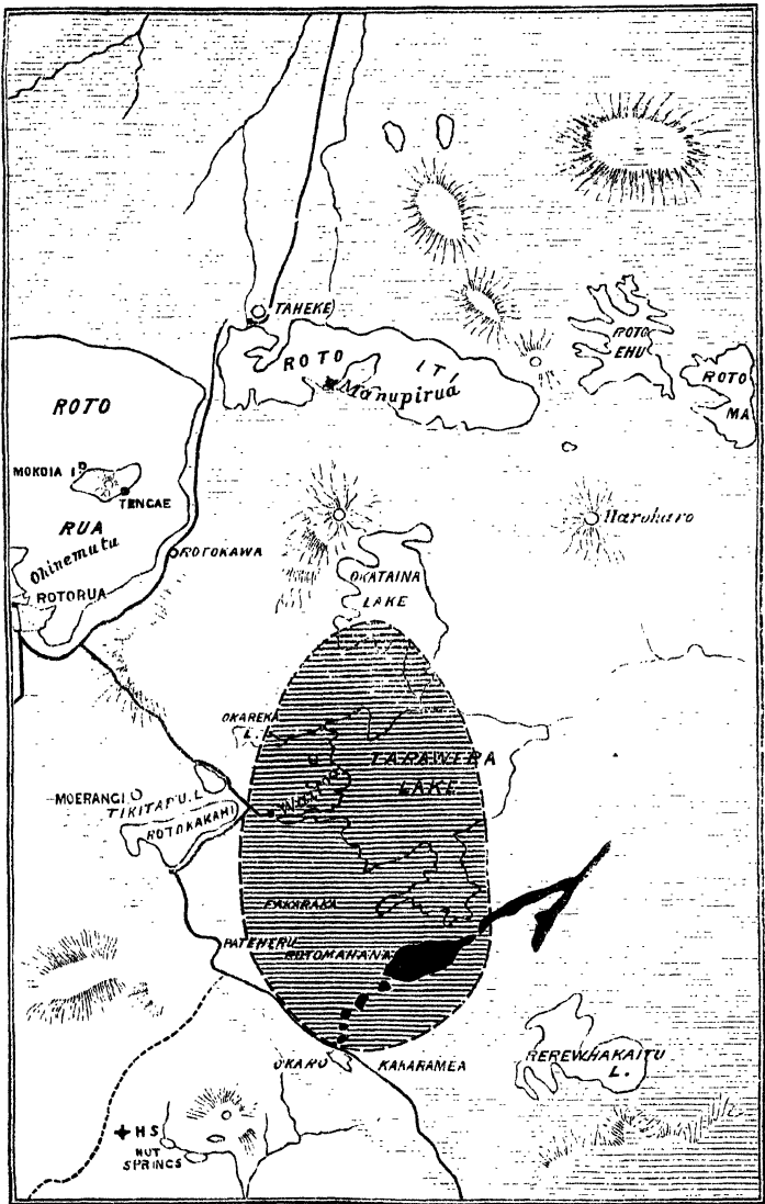
Fig. 2.—Map of the country around Tarawera Volcano after the Eruption of 10th June, 1886. (Scale 5 miles to 1 inch.)
