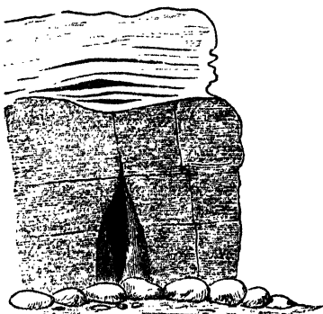
Fig. 4.— Hornblende-schists overlying Gneiss, Creux Harbour, Sark.
