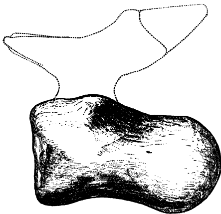
Caudal vertebra of a Dinosaur, with the neural arch restored; from the Wealden of Brook, Isle of Wight. \frac{1}{3} nat. size. British Museum (No. R. 151).
