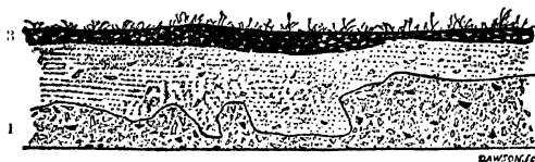
Fig. 4.—Section on Sullington Common.
