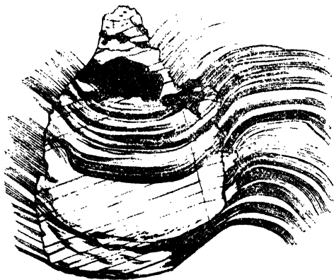
Fig. 2.— Crystal of Kyanite in Mica-Schist near Bolt Head. (Enlarged 70 diameters.)
