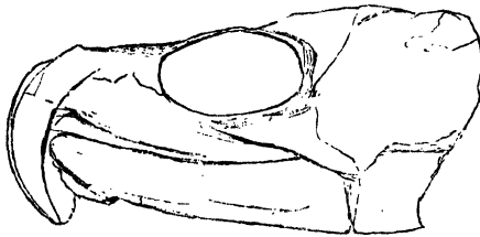
Fig. 2.—Incomplete Skull of Rhynchosaurus , side view.
