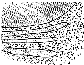
Fig. 4.—Section of Diorite (? exfoliated) in Granite.
