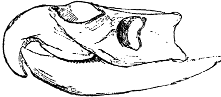
Fig. 1.—Skull of Hyperodapedon , side view.
