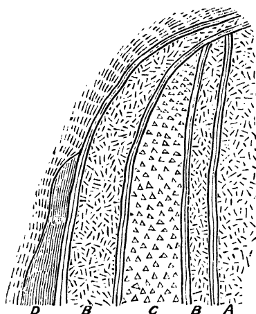
Fig. 3.— Plan of Vein-structure in Schistose Rocks.
