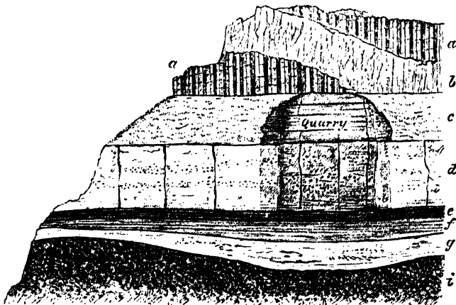
Fig. 3.—Quarry in east side of Ravine, Ardtun Head.
