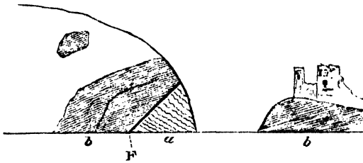
Fig. 3.—Cliff opposite the Old Castle near Salcombe.
