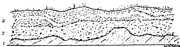
Fig. 5.—Section at Uootham Firs.
