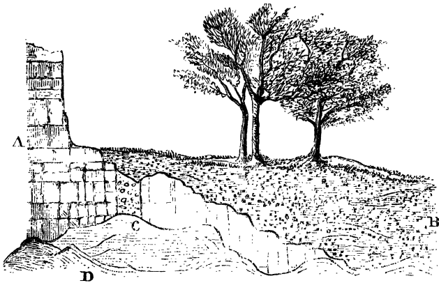
Fig. 4.—Section in Quarry near the Village of St. George. (Scale 30 feet to 1 inch.)
