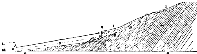
Fig. 1.— Diagram Section showing the Mode of Formation of some of the High-level Beaches of Devonshire.
