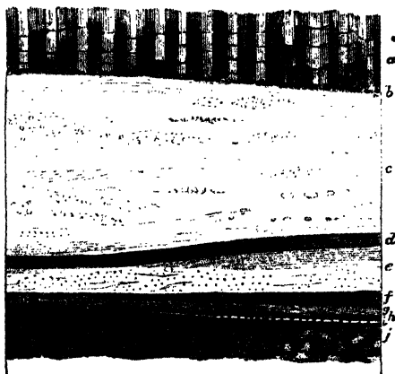
Fig. 6.— Leaf-bed and Gravels at Ariltun. (Scale about 30 feet to 1 inch.)
