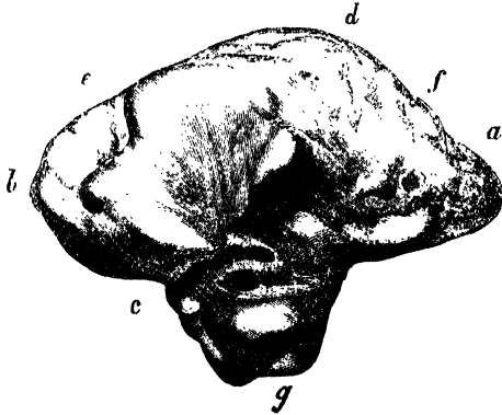
Fig. 2.— Eucetus amblyodon , Du Bus. The left periotic; from the Red Crag. Two thirds nat. size. British Museum (No. 27854). Letters as in Plate II.
