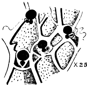
Fig. 2.— Schizoporella obliqua (?), MacG., from Waipukurau, New Zealand.
