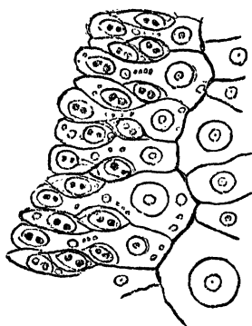
Fig. 3.— Ambulacral Plates from above the Equator of Pelanechinus corallinus. \times 4 .
