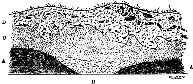
Fig. 1.—Section on Fittleworth Common .
