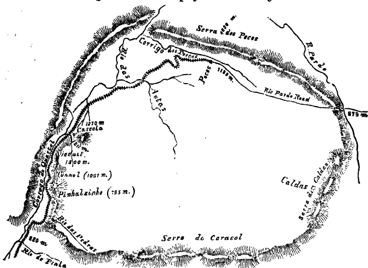
Fig. 7.—Sketch Map of the Caldas region.
