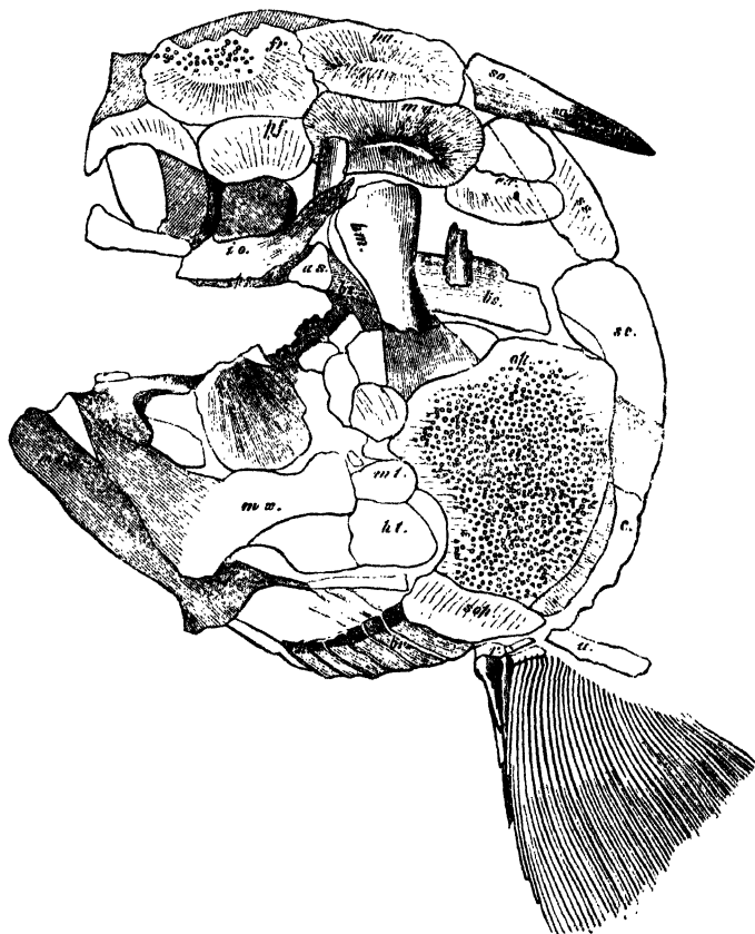
Diagram of the Bones of the Head of Chondrosteus acipenseroides (One third natural size.)
