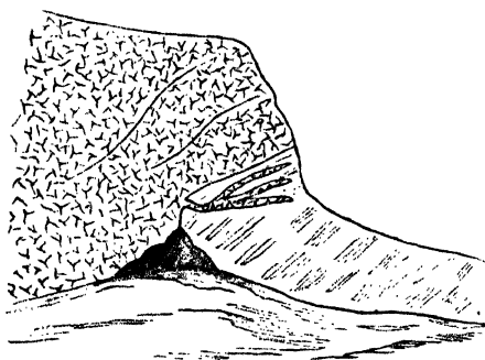
Fig. 5.— Rough sketch of Granite overlying Hornblende-schists at south-east junction on Little Sark. Schists perfectly bedded, dipping S.W.
