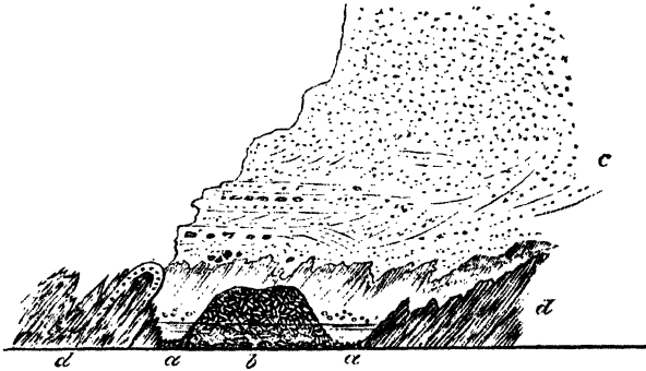
Fig. 5.— Boulder of Grey Porphyry at base of Cliff South of Saunton Down, North end of Barustaple Bay (April 11, 1887). (Scale 7½ feet to 1 inch.)
