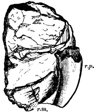
Fig. 8.— Hyperodapedon Gordoni . Mr. Grant's specimen. Right side.
