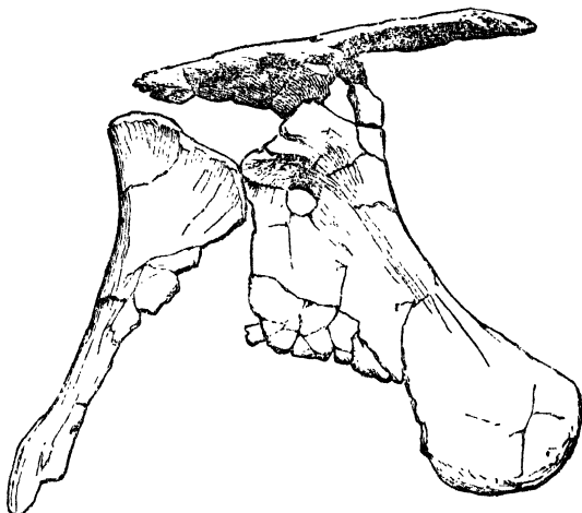
Fig. 1.— Pelvis of Ornithopsis Leedsii, from the Kimmeridge Clay of Northamptonshire. About one-twentieth natural size.
