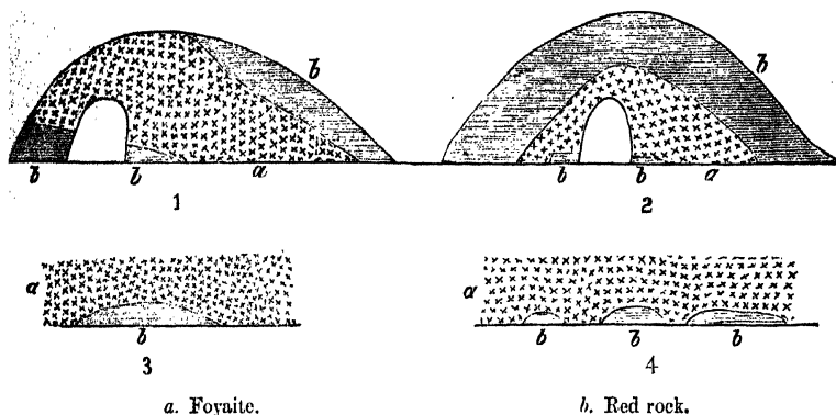
Fig. 4.—Sections across and on the sides of the tunnel near Pinhalzinho.
