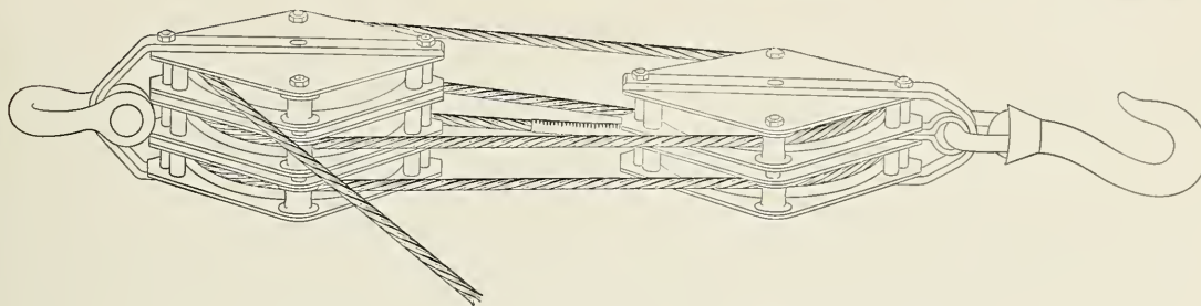
Fig. 5 Stress on Rope is one-fifth the Load
