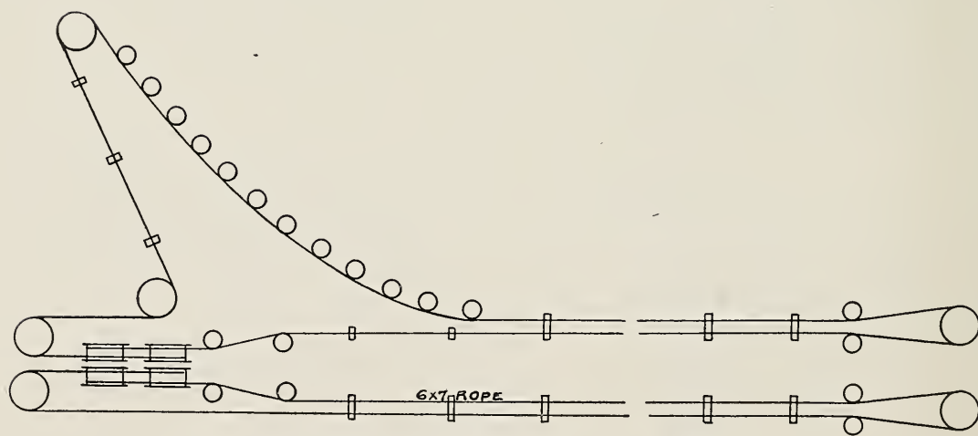
ORE DOCK HAULAGE ROAD FOR BROAD GAUGE CARS
