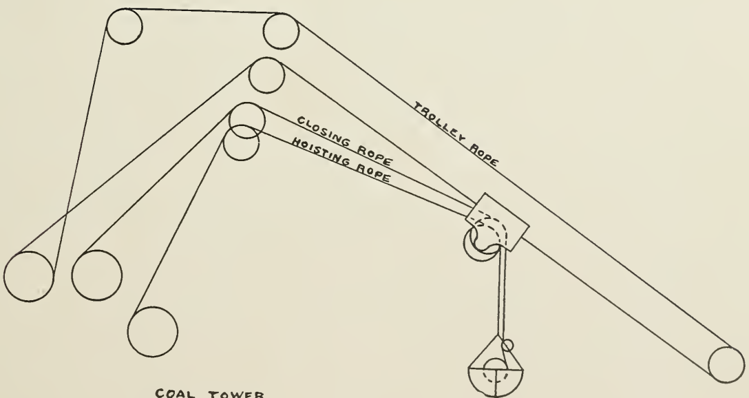
COAL TOWER
