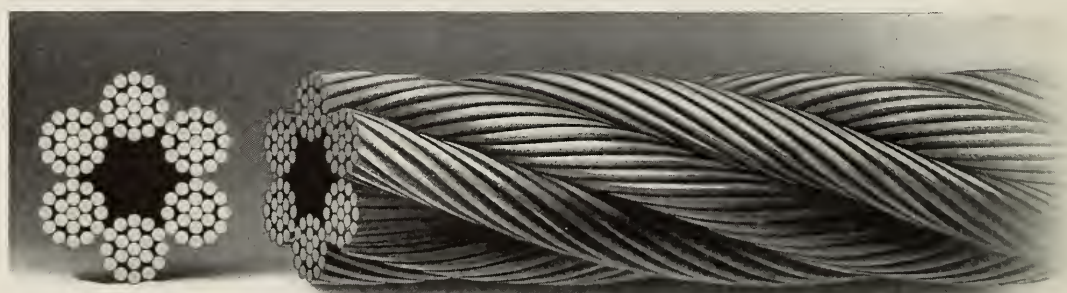
Reverse lay rope, also known as right and left lay rope
