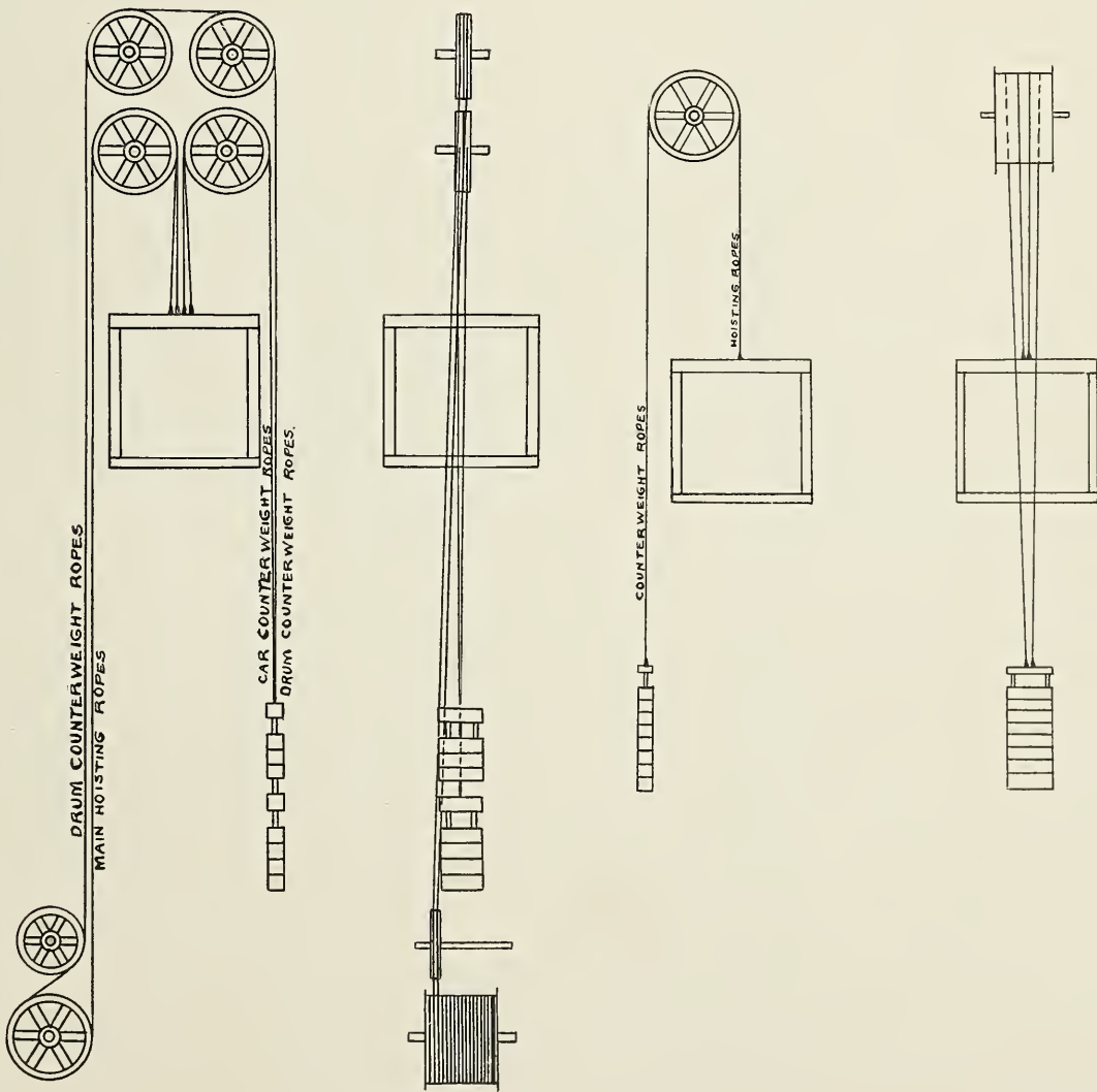
ELECTRIC OR BELT DRIVEN ELEVATOR
