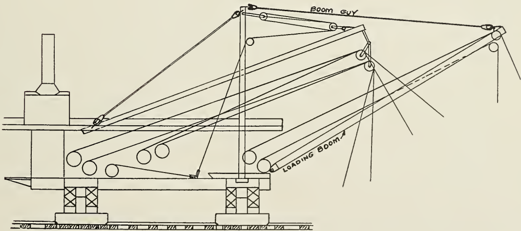
COMBINED SKIDDER AND LOADER
