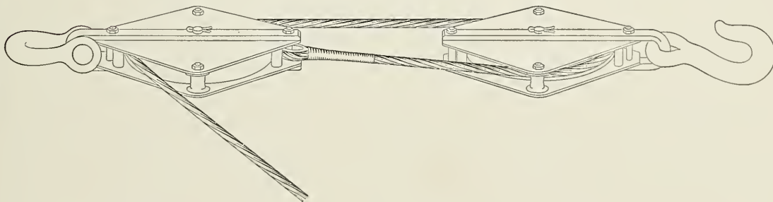
Fig. 2 Stress on Rope is one-half the Load
