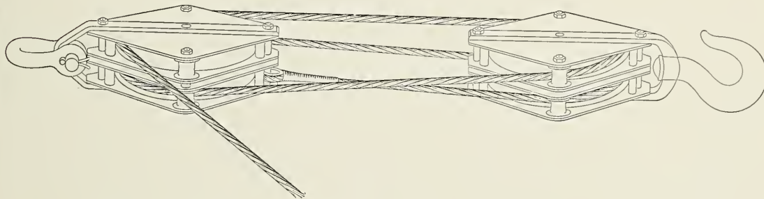
Fig. 4 Stress on Rope is one-fourth the Load
