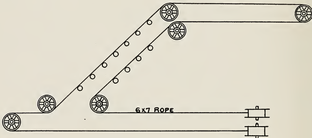
TAIL ROPE HAULAGE SYSTEM
