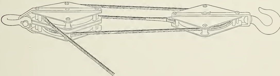
Fig. 3 Stress on Rope is one-third the Load
