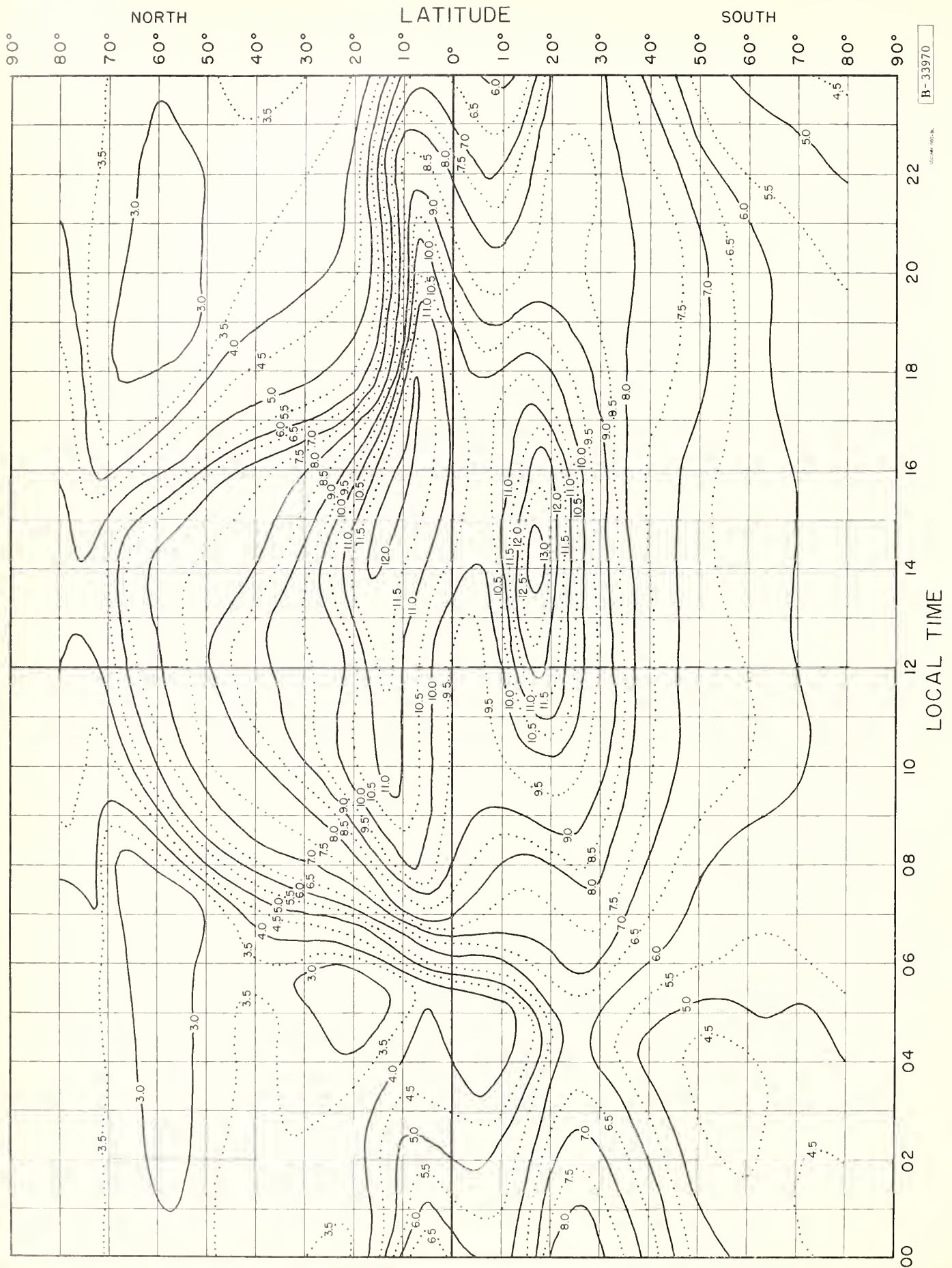
FIG. 7. MEDIAN F2 - ZERO - MUF, IN Mc, I ZONE (PACIFIC), PREDICTED FOR DECEMBER 1962
